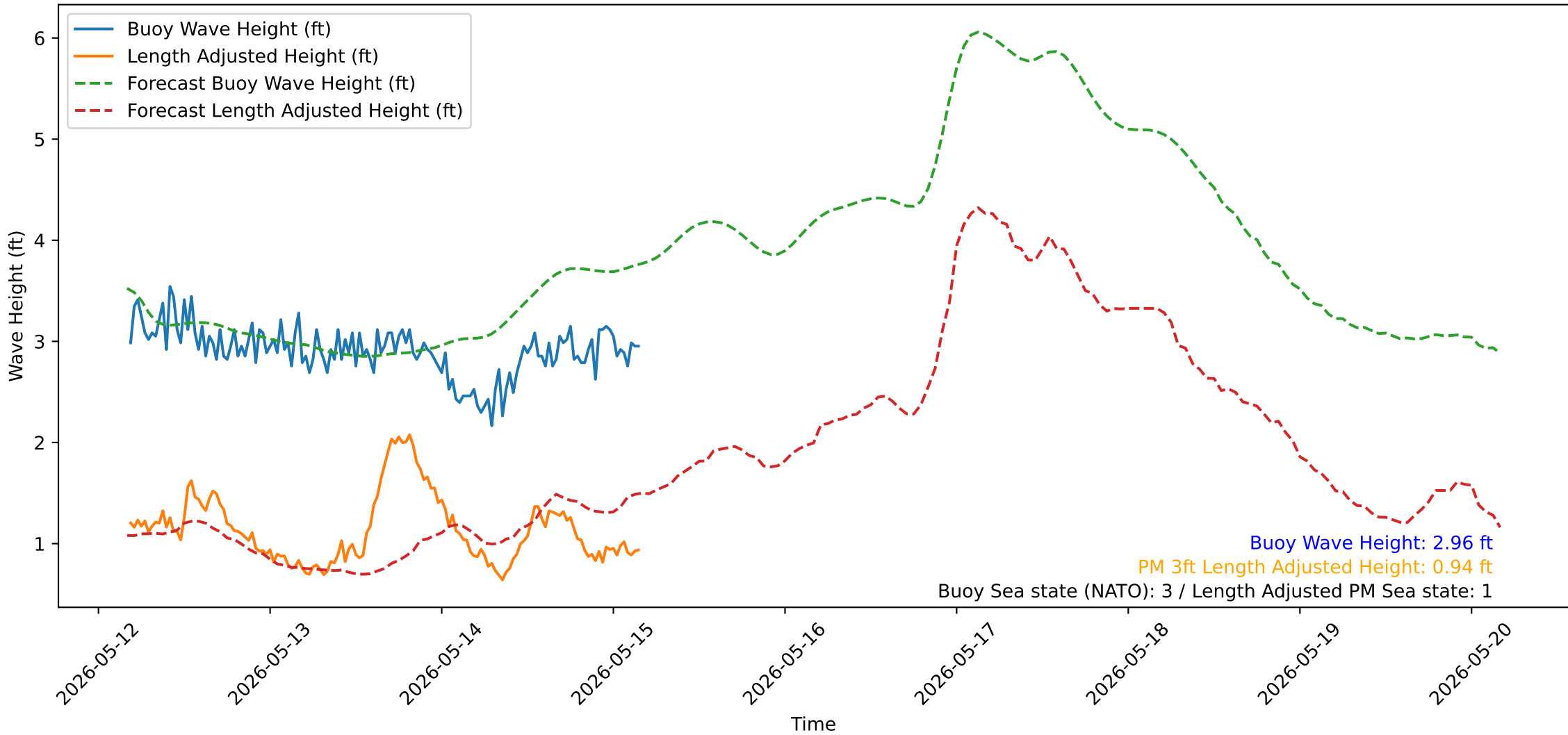
Wave Heights over Time for Oceanside Harbor at 2026-05-15 04:20:35
