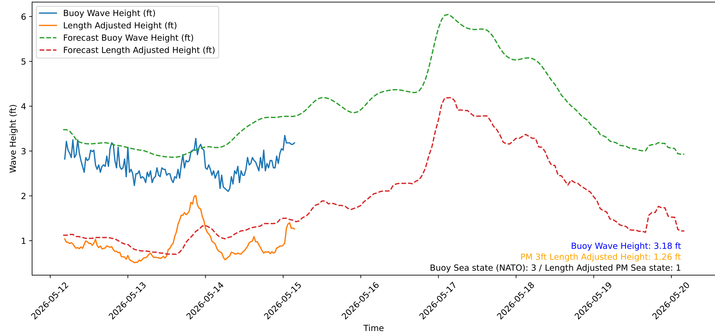
Wave Heights over Time for Green Beach at 2026-05-15 04:21:26
