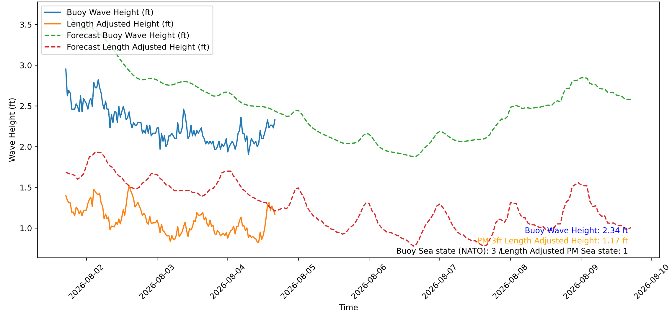
Wave Heights over Time for Red Beach at 2026-08-04 16:40:46
