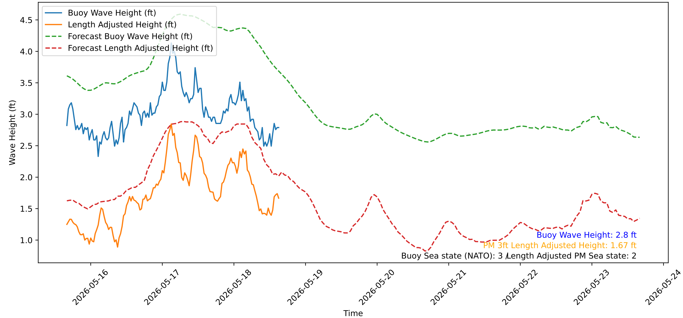
Wave Heights over Time for Red Beach at 2026-05-18 15:50:52
