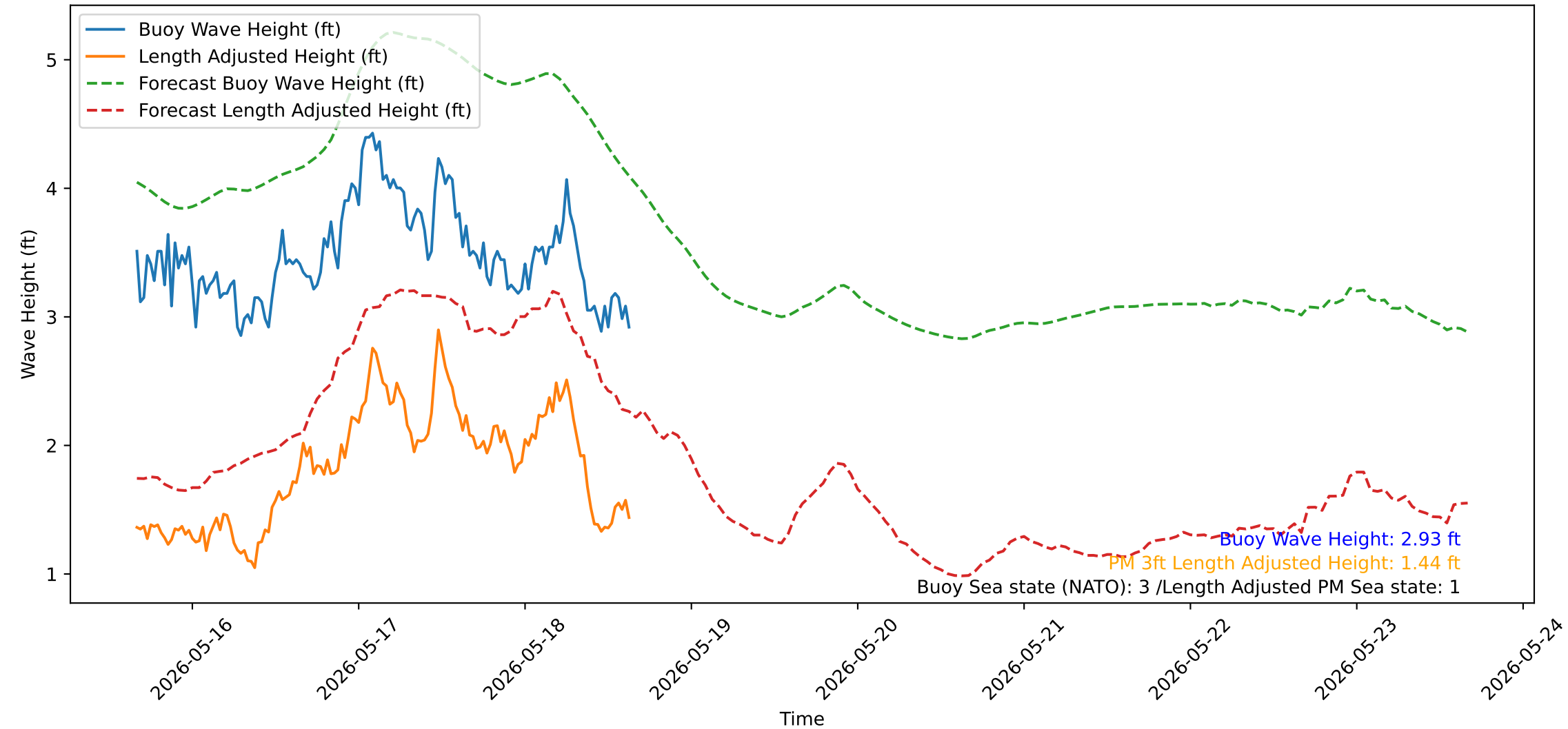
Wave Heights over Time for Green Beach at 2026-05-18 15:51:14
