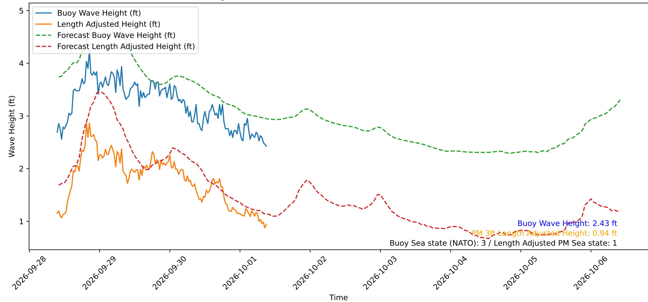
Wave Heights over Time for Oceanside Harbor at 2026-10-01 09:40:29
