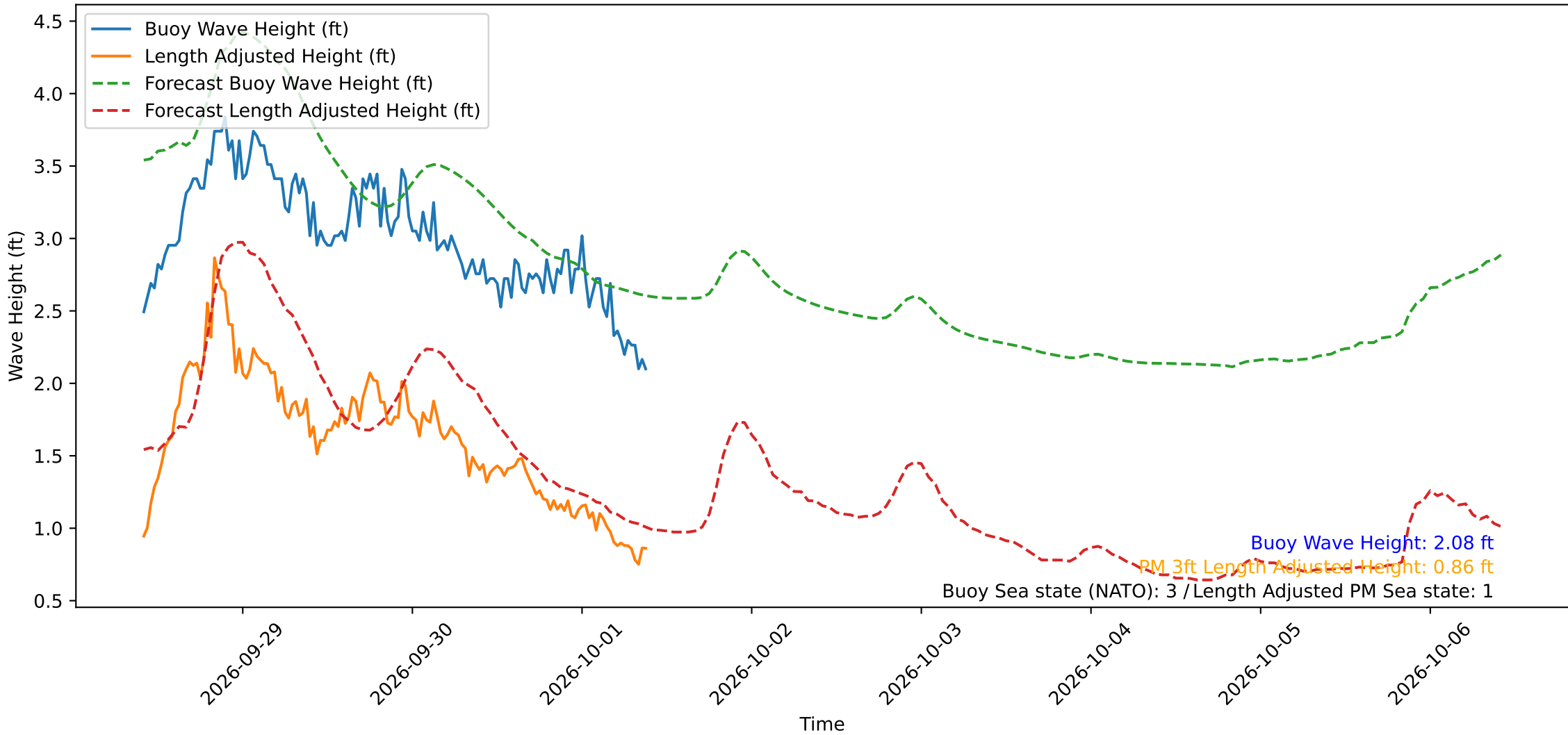
Wave Heights over Time for Red Beach at 2026-10-01 09:40:49
