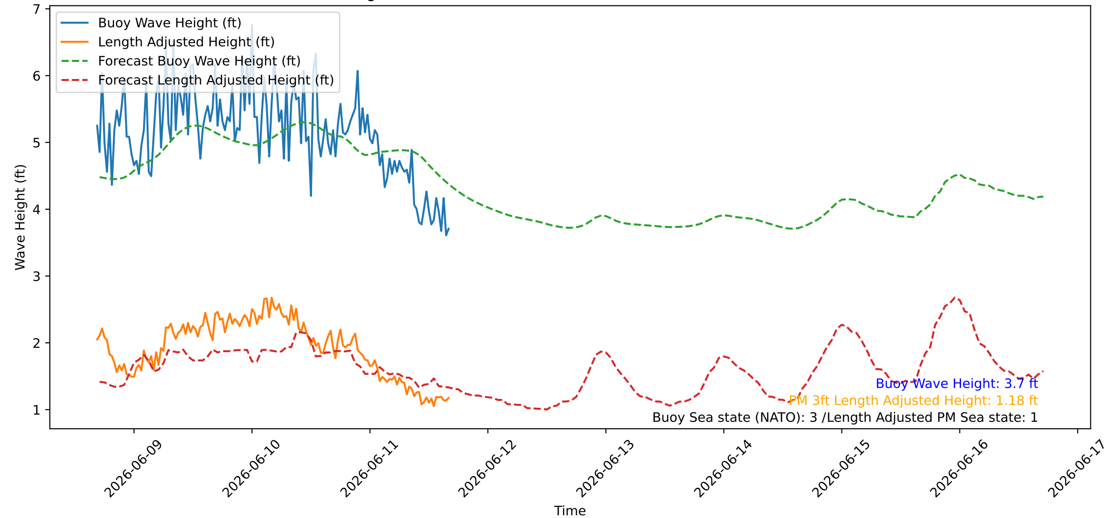
Wave Heights over Time for Oceanside Harbor at 2026-06-11 16:40:26
