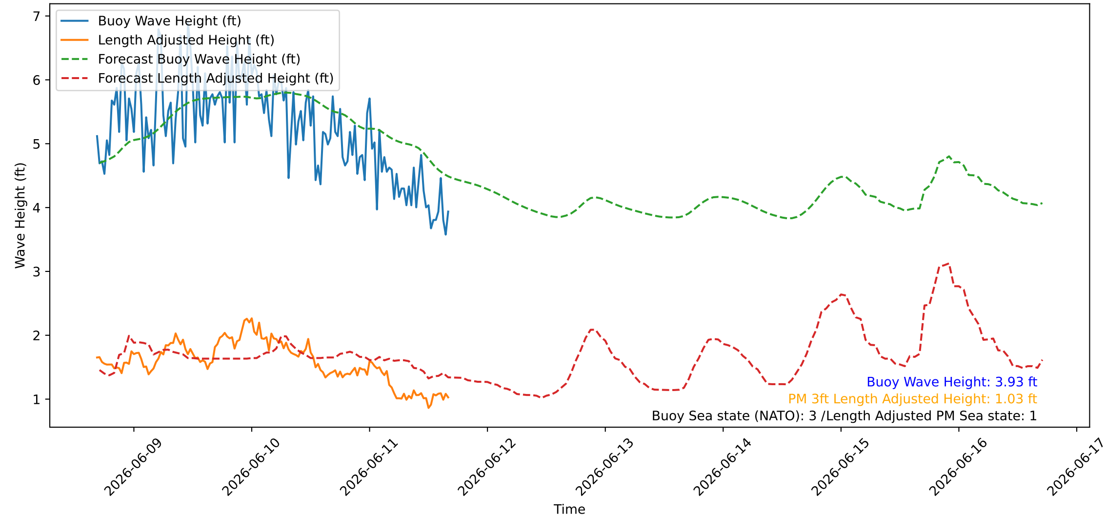
Wave Heights over Time for Green Beach at 2026-06-11 16:41:08
