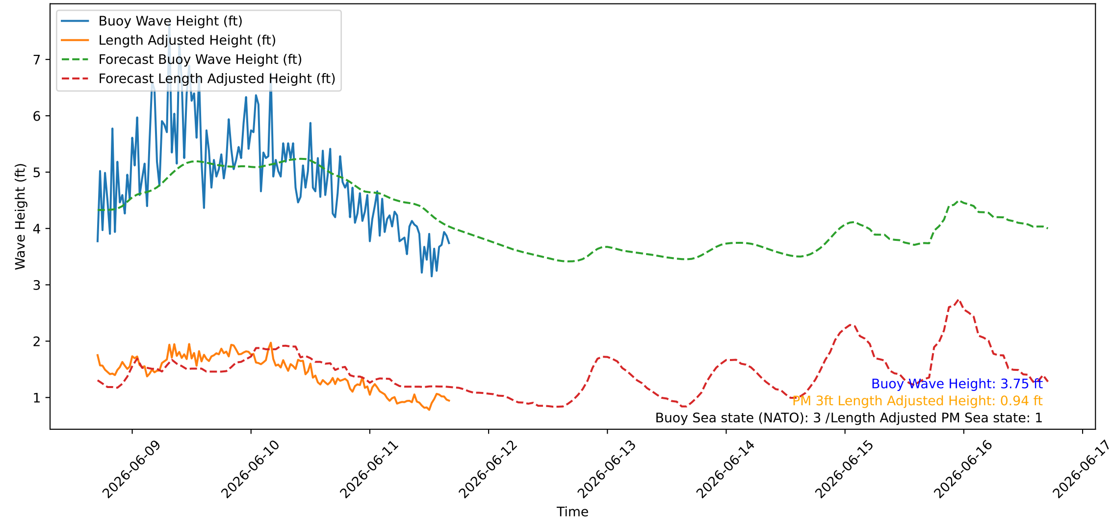
Wave Heights over Time for Red Beach at 2026-06-11 16:40:45
