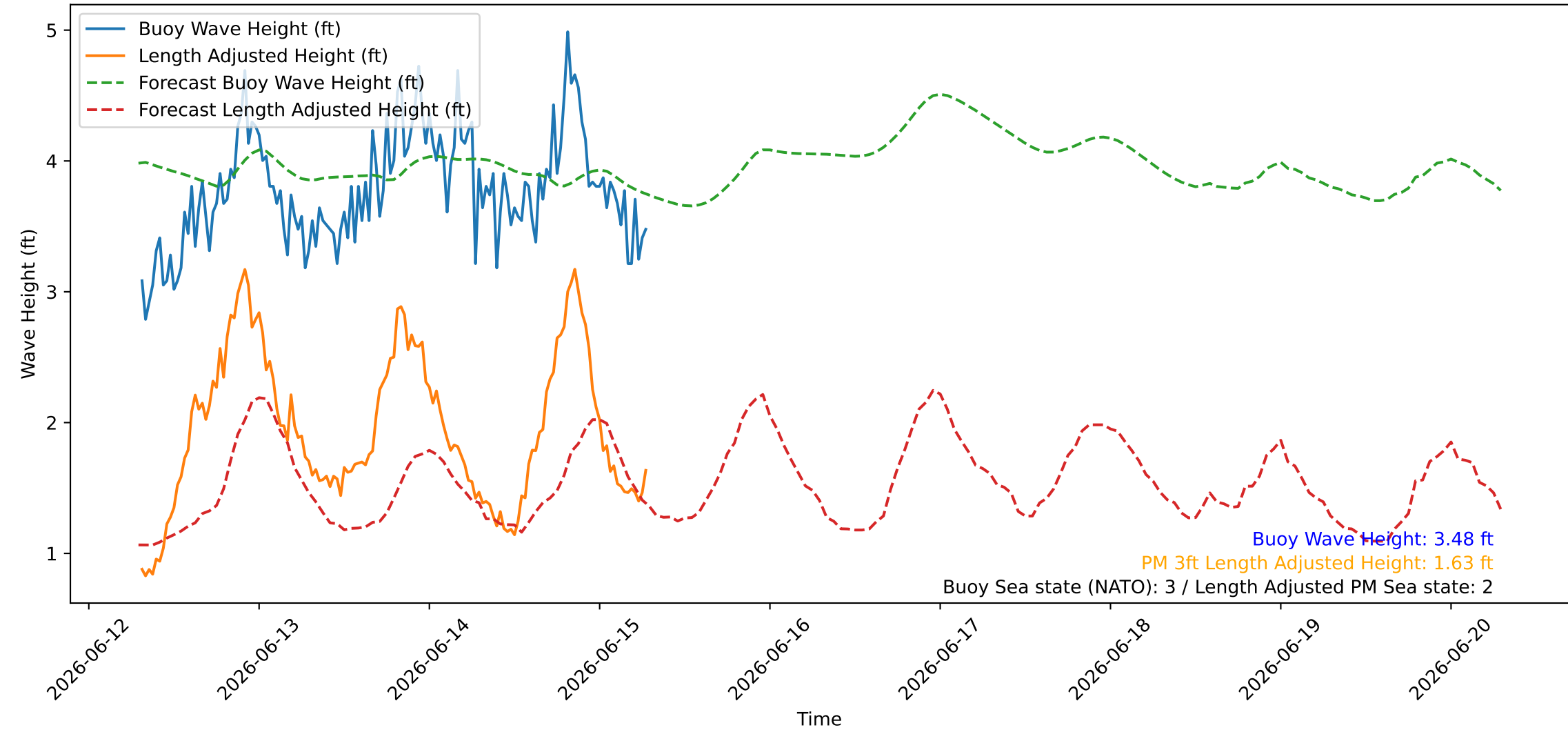
Wave Heights over Time for Oceanside Harbor at 2026-06-15 07:20:26
