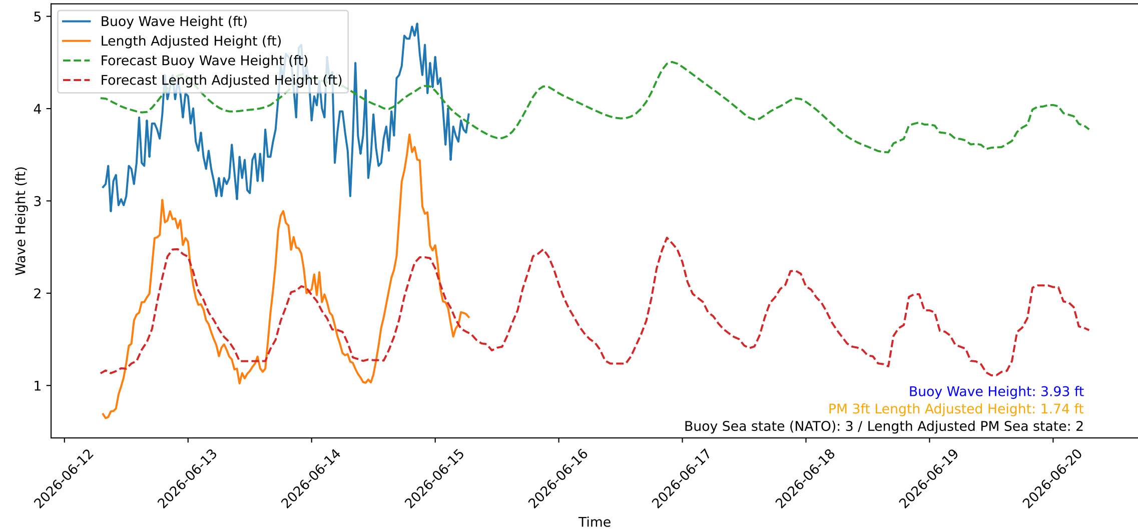
Wave Heights over Time for Green Beach at 2026-06-15 07:21:09
