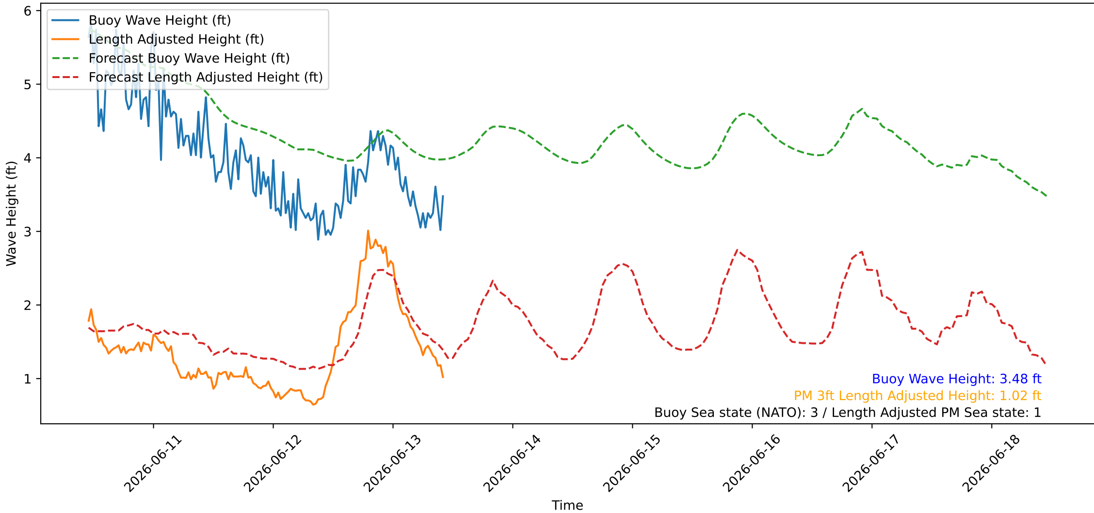
Wave Heights over Time for Green Beach at 2026-06-13 10:51:09
