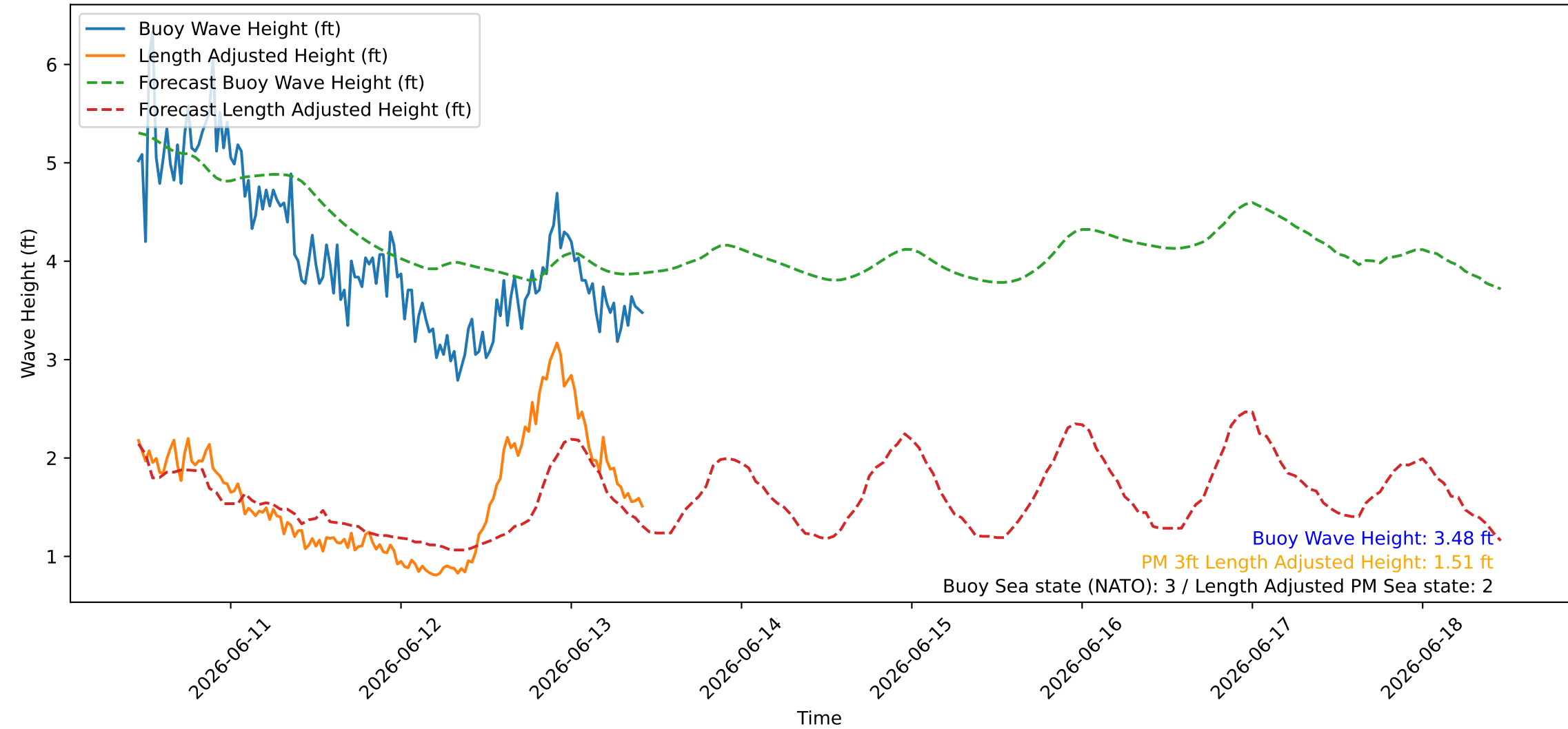
Wave Heights over Time for Oceanside Harbor at 2026-06-13 10:50:26
