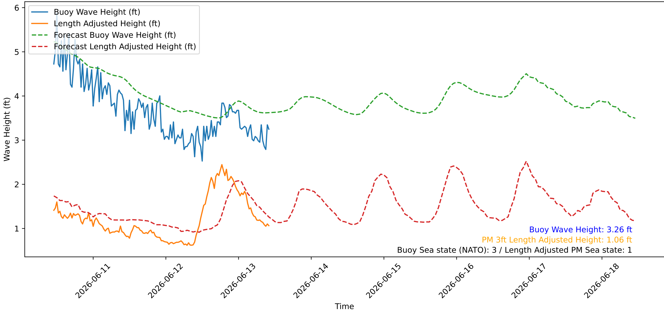
Wave Heights over Time for Red Beach at 2026-06-13 10:50:46
