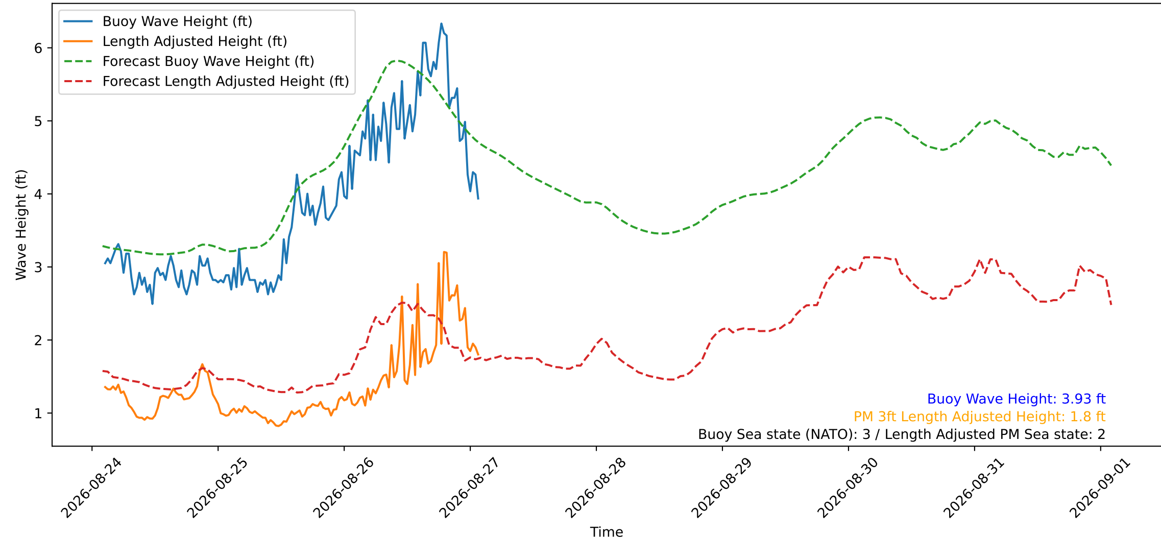
Wave Heights over Time for Green Beach at 2026-08-27 02:11:13
