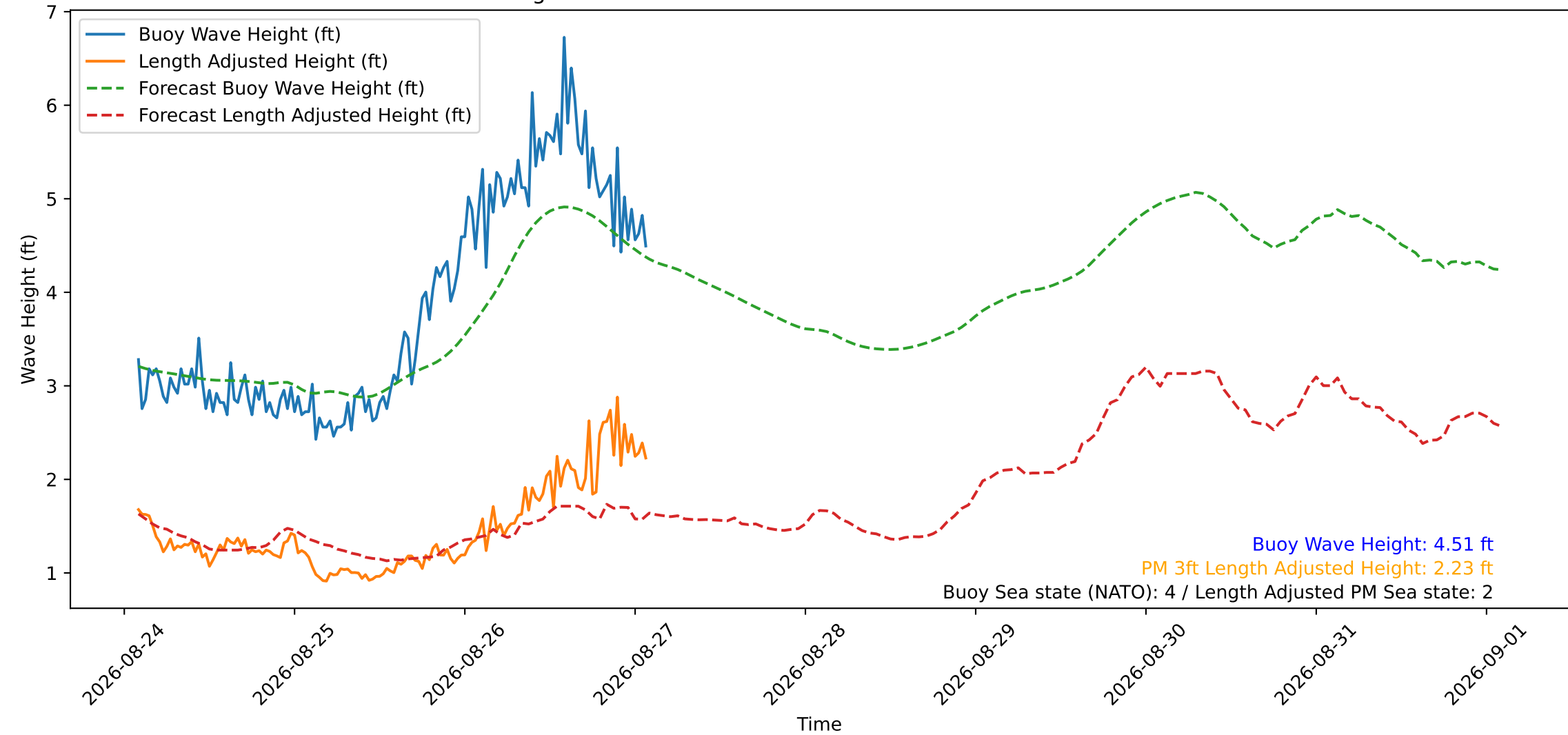
Wave Heights over Time for Oceanside Harbor at 2026-08-27 02:10:30
