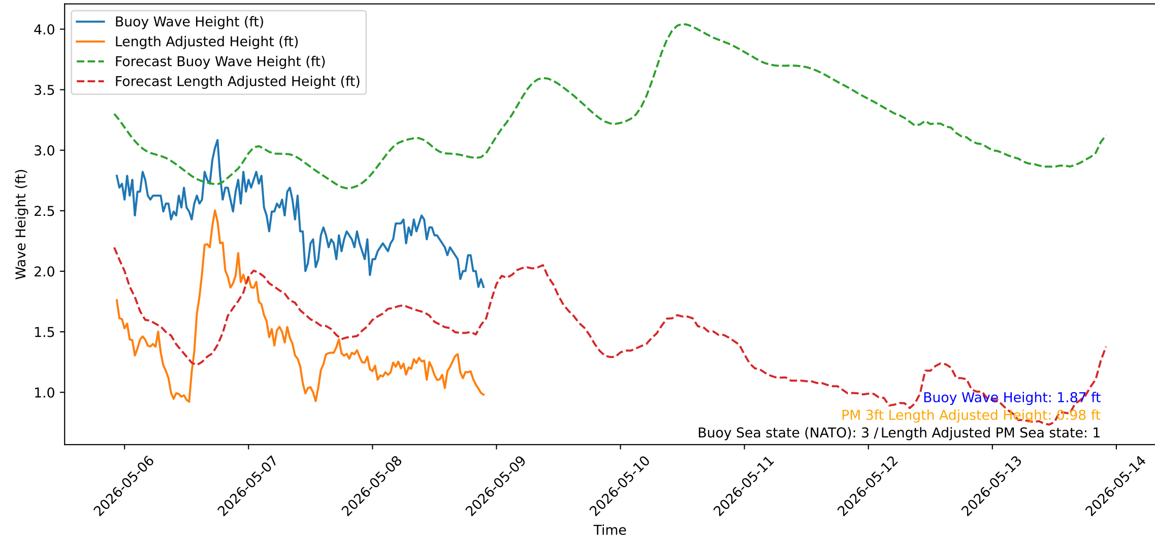
Wave Heights over Time for Oceanside Harbor at 2026-05-08 22:20:31
