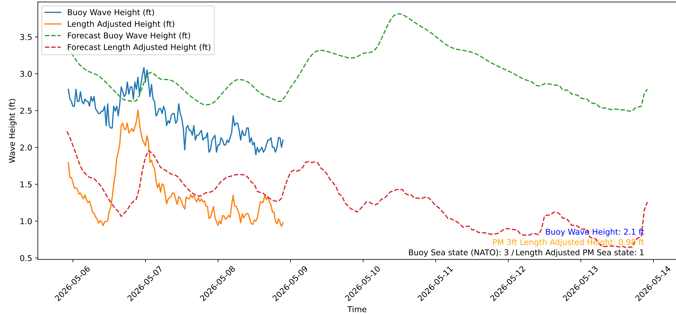
Wave Heights over Time for Red Beach at 2026-05-08 22:20:51
