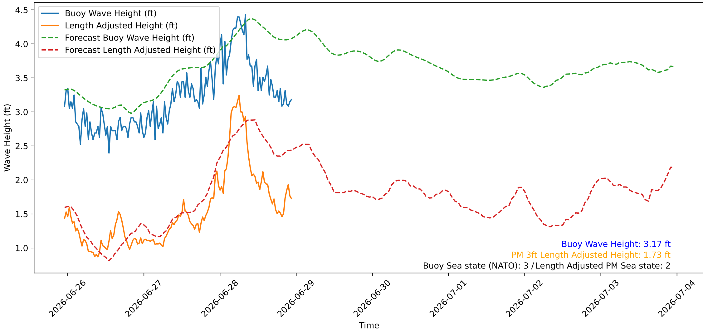
Wave Heights over Time for Oceanside Harbor at 2026-06-28 23:10:25
