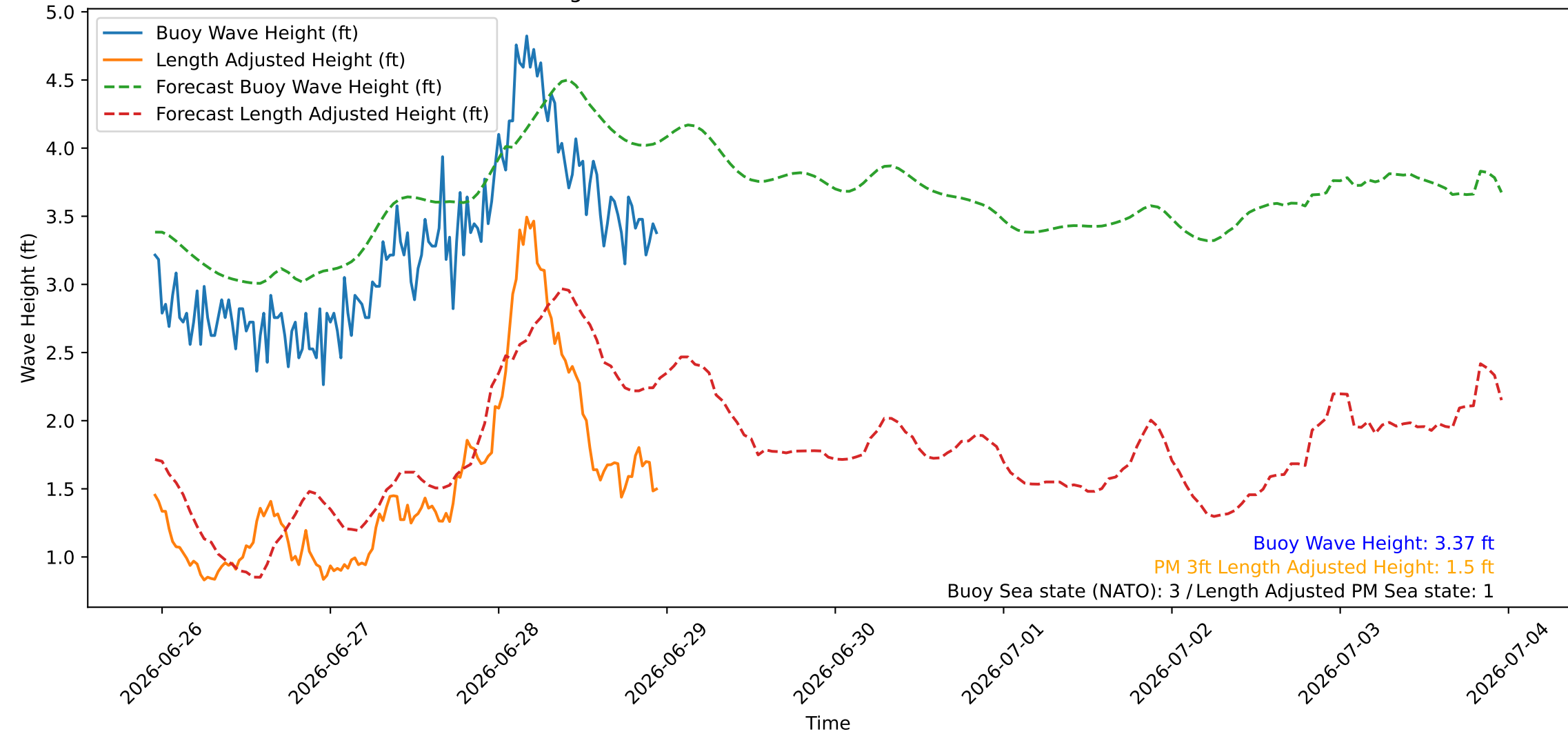
Wave Heights over Time for Green Beach at 2026-06-28 23:11:07
