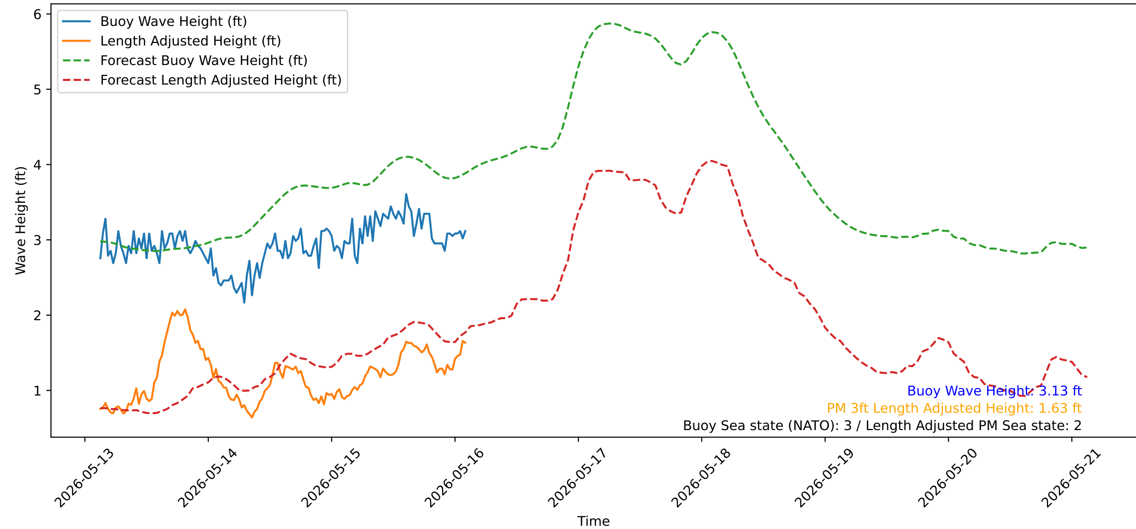
Wave Heights over Time for Oceanside Harbor at 2026-05-16 02:50:32
