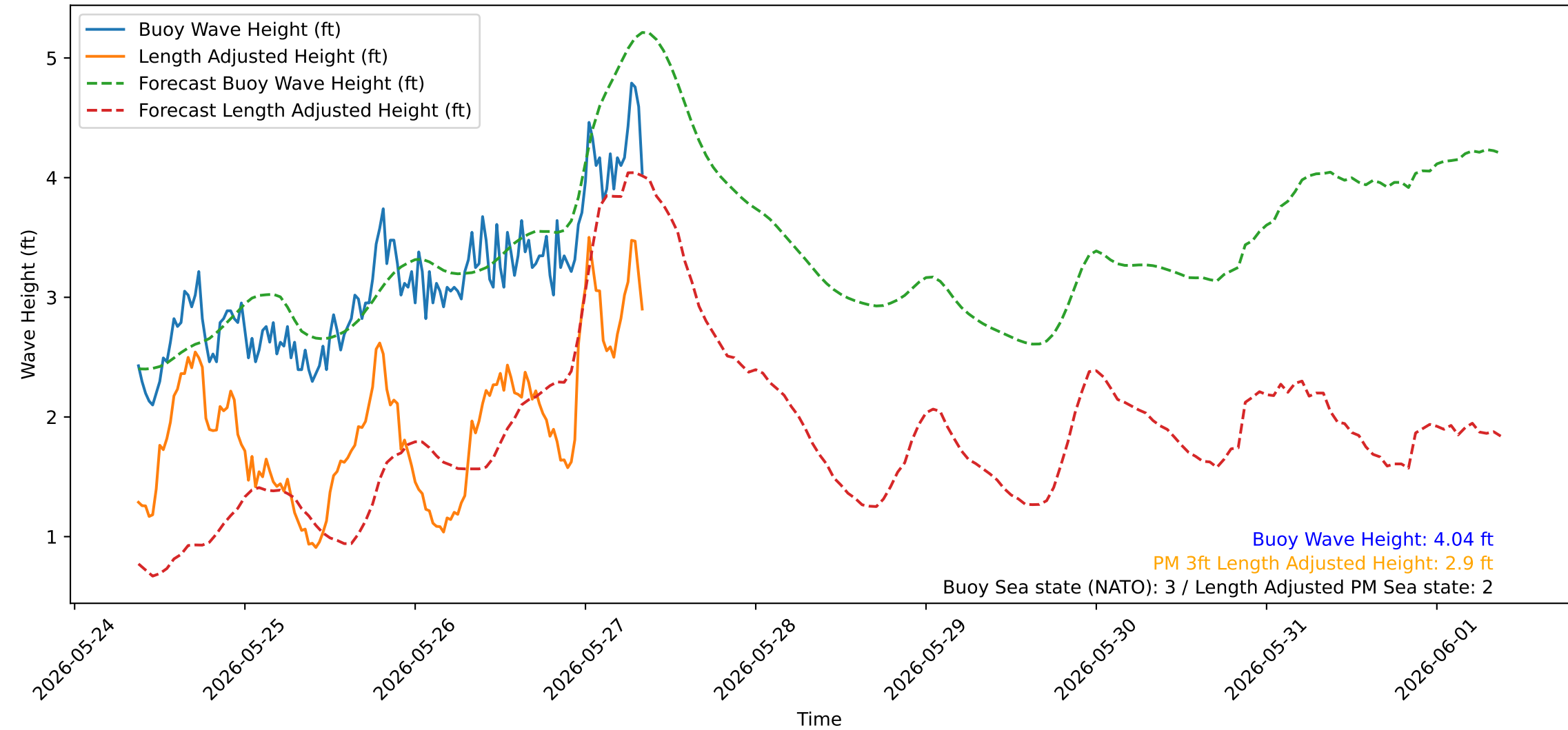
Wave Heights over Time for Red Beach at 2026-05-27 08:50:46
