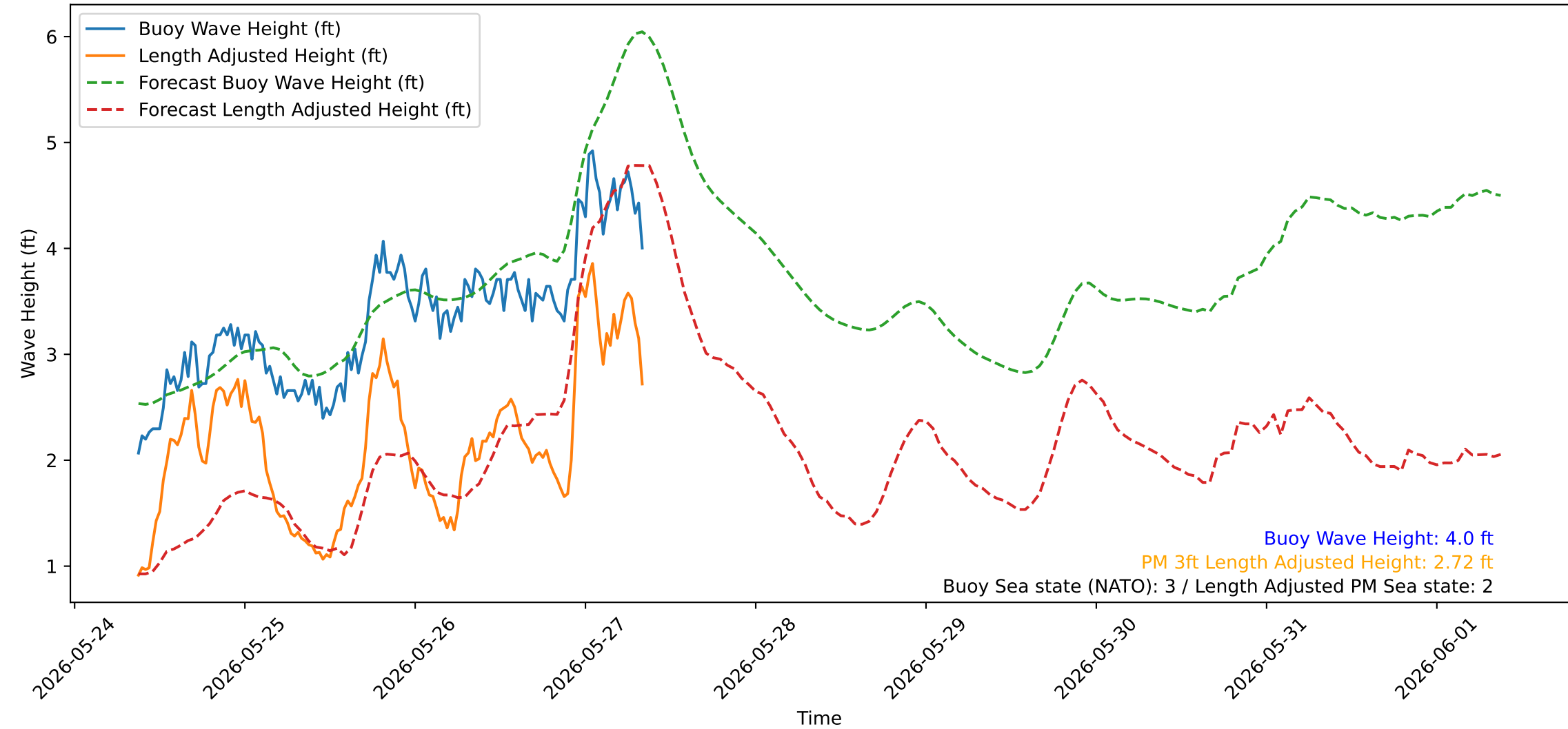
Wave Heights over Time for Green Beach at 2026-05-27 08:51:09
