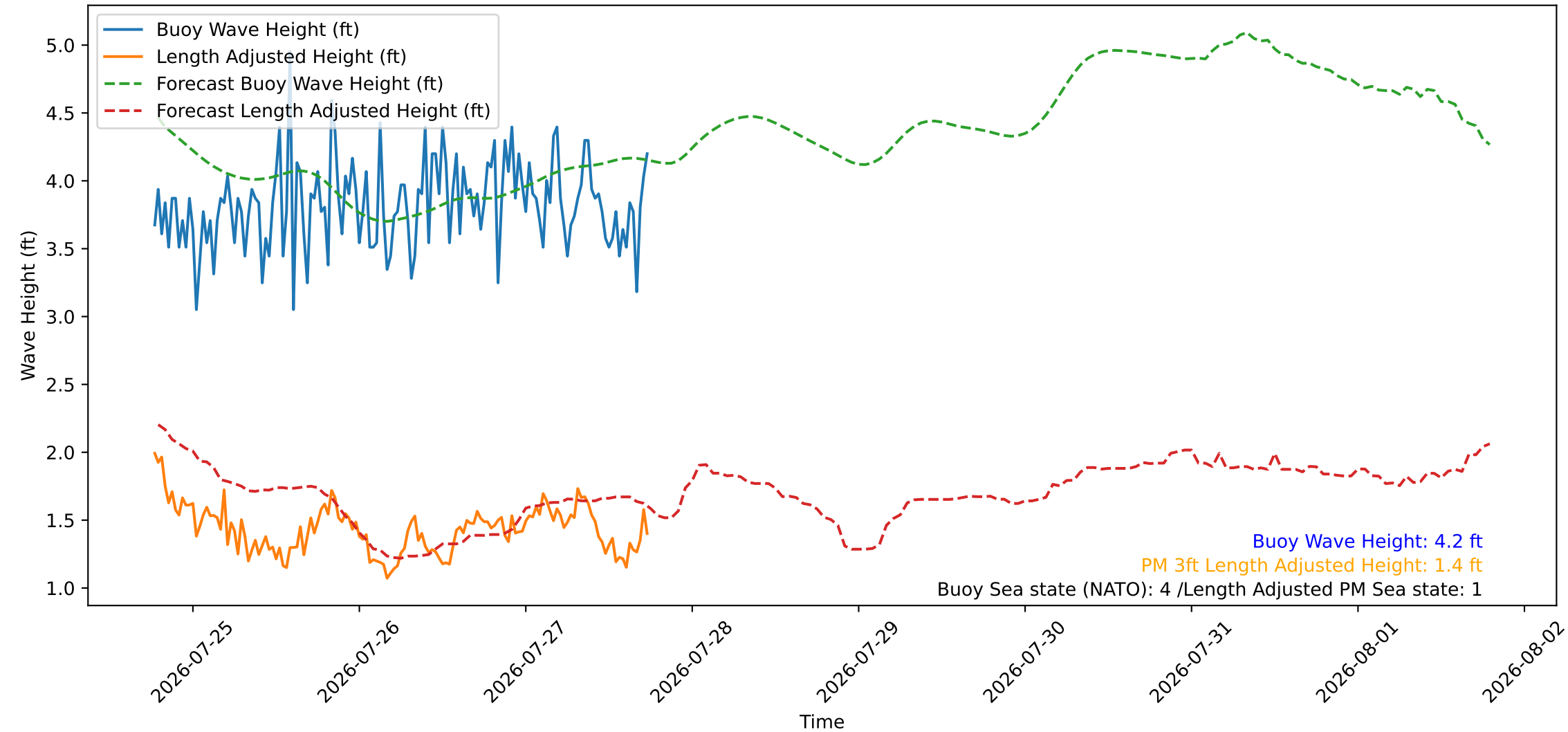
Wave Heights over Time for Oceanside Harbor at 2026-07-27 18:30:27
