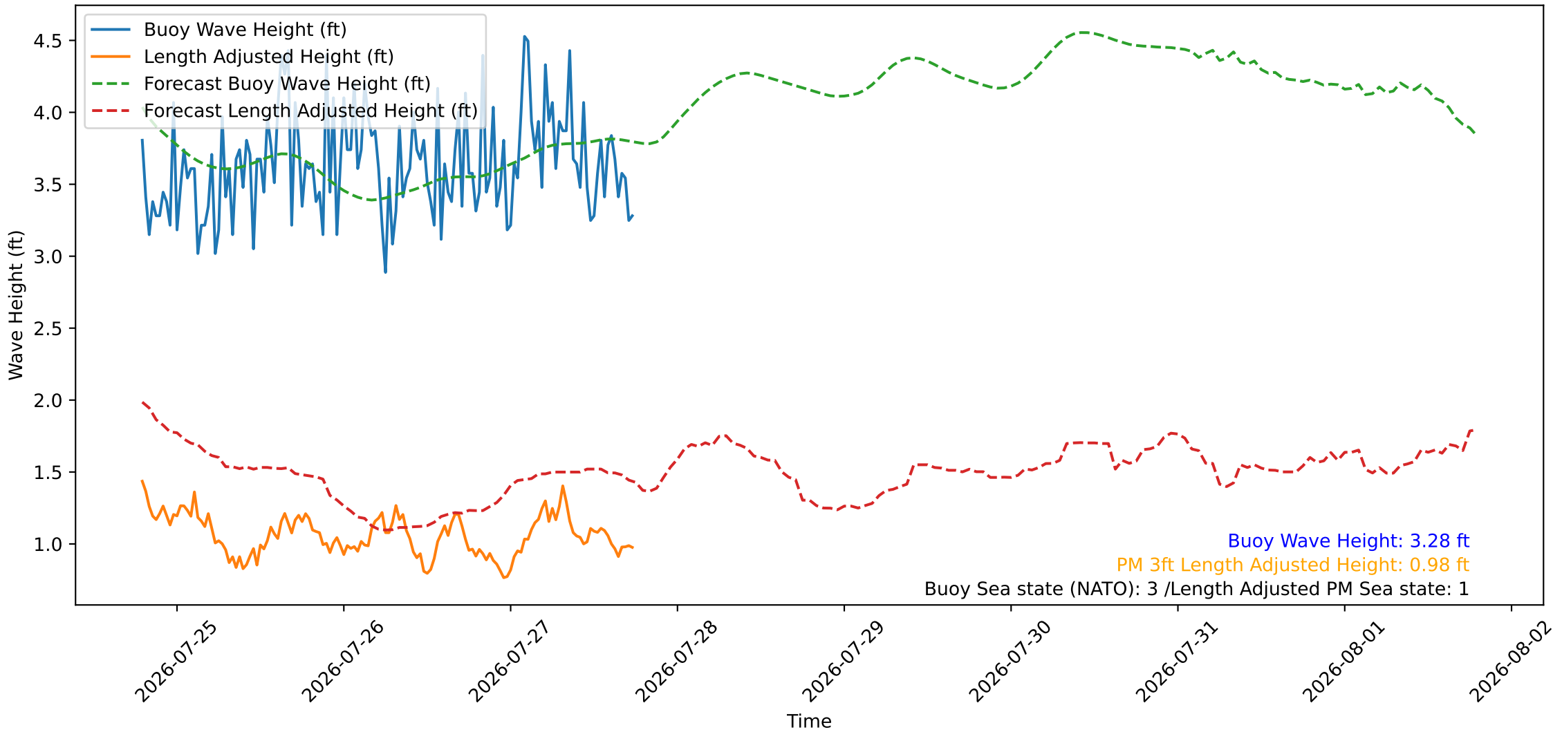
Wave Heights over Time for Red Beach at 2026-07-27 18:30:47
