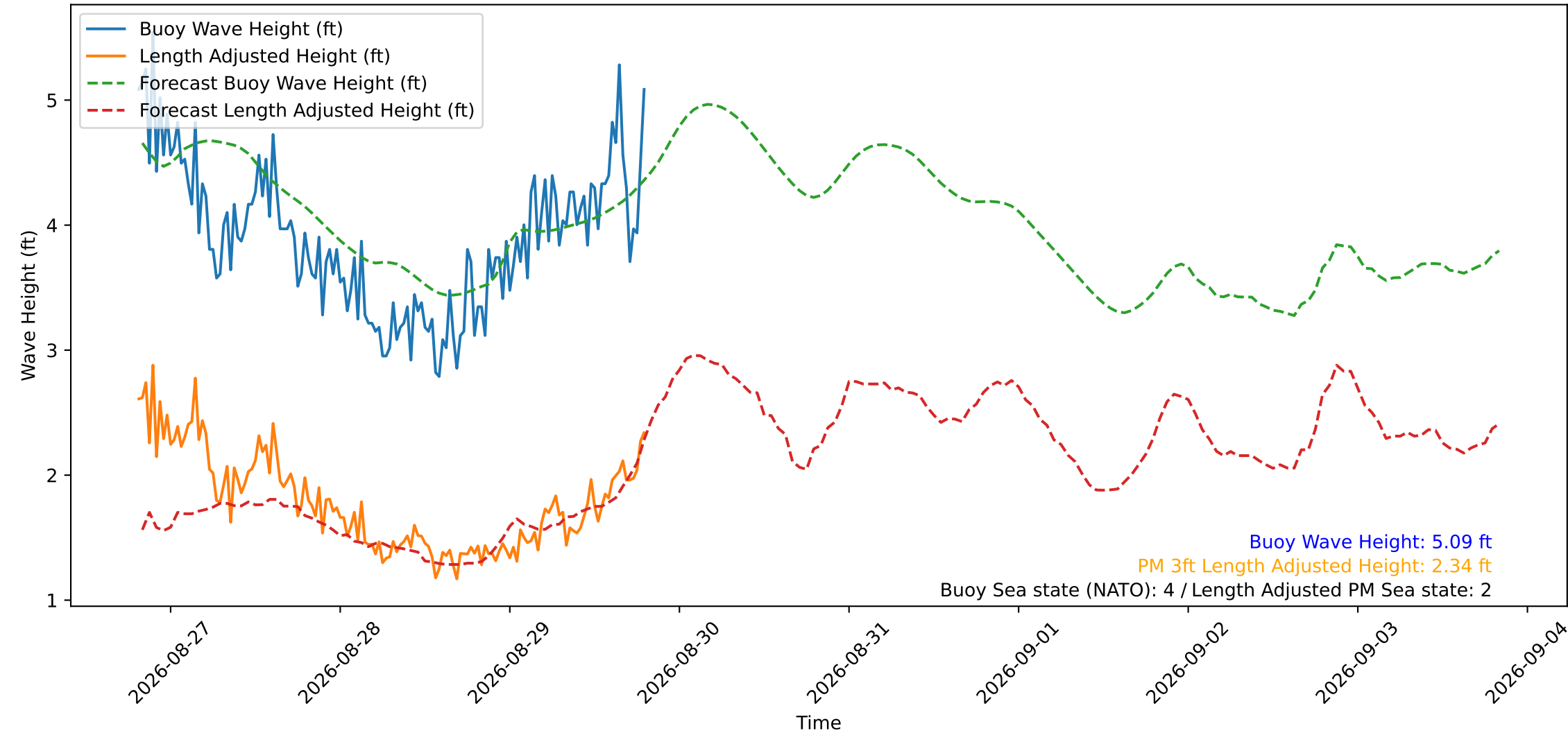
Wave Heights over Time for Oceanside Harbor at 2026-08-29 19:40:30
