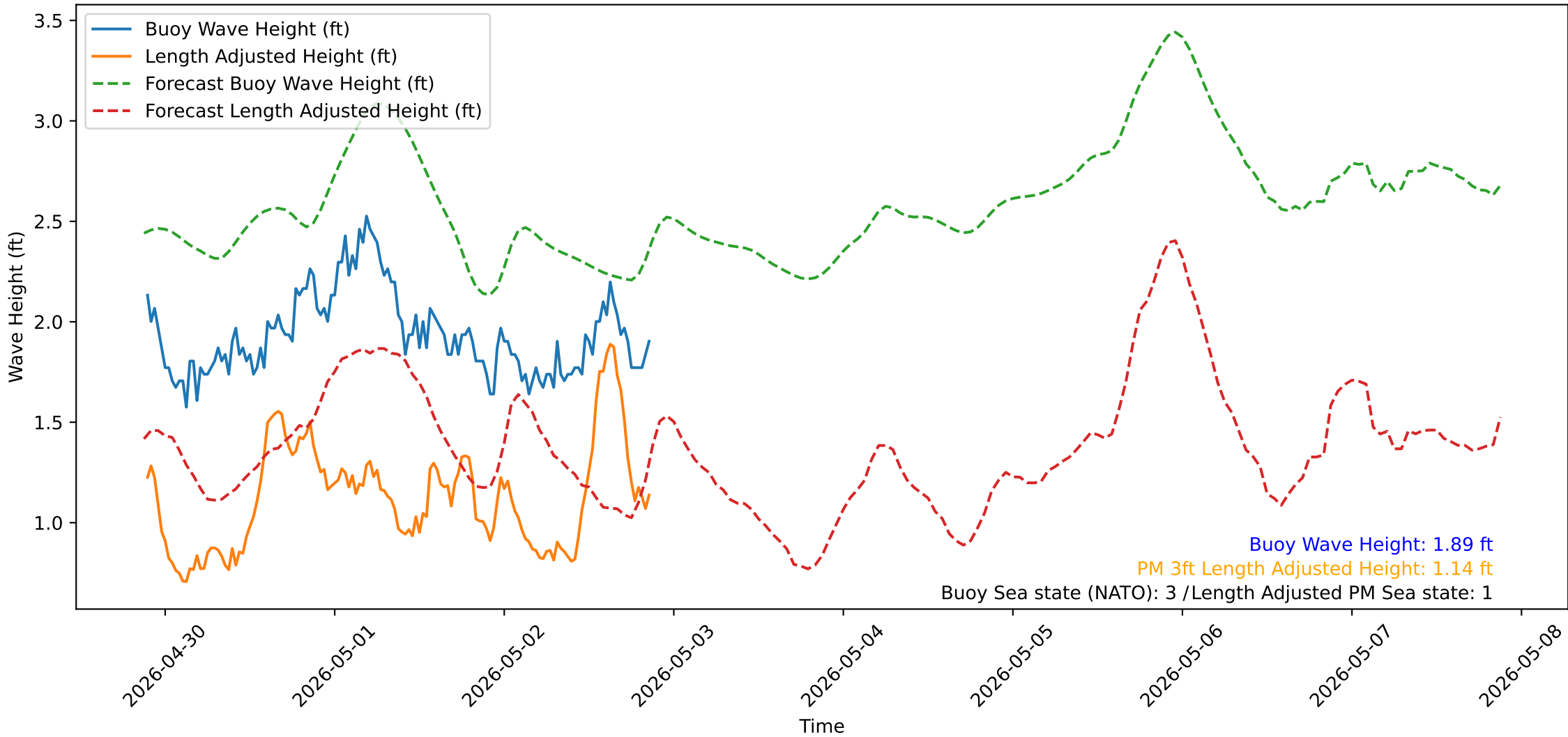
Wave Heights over Time for Red Beach at 2026-05-02 21:10:51
