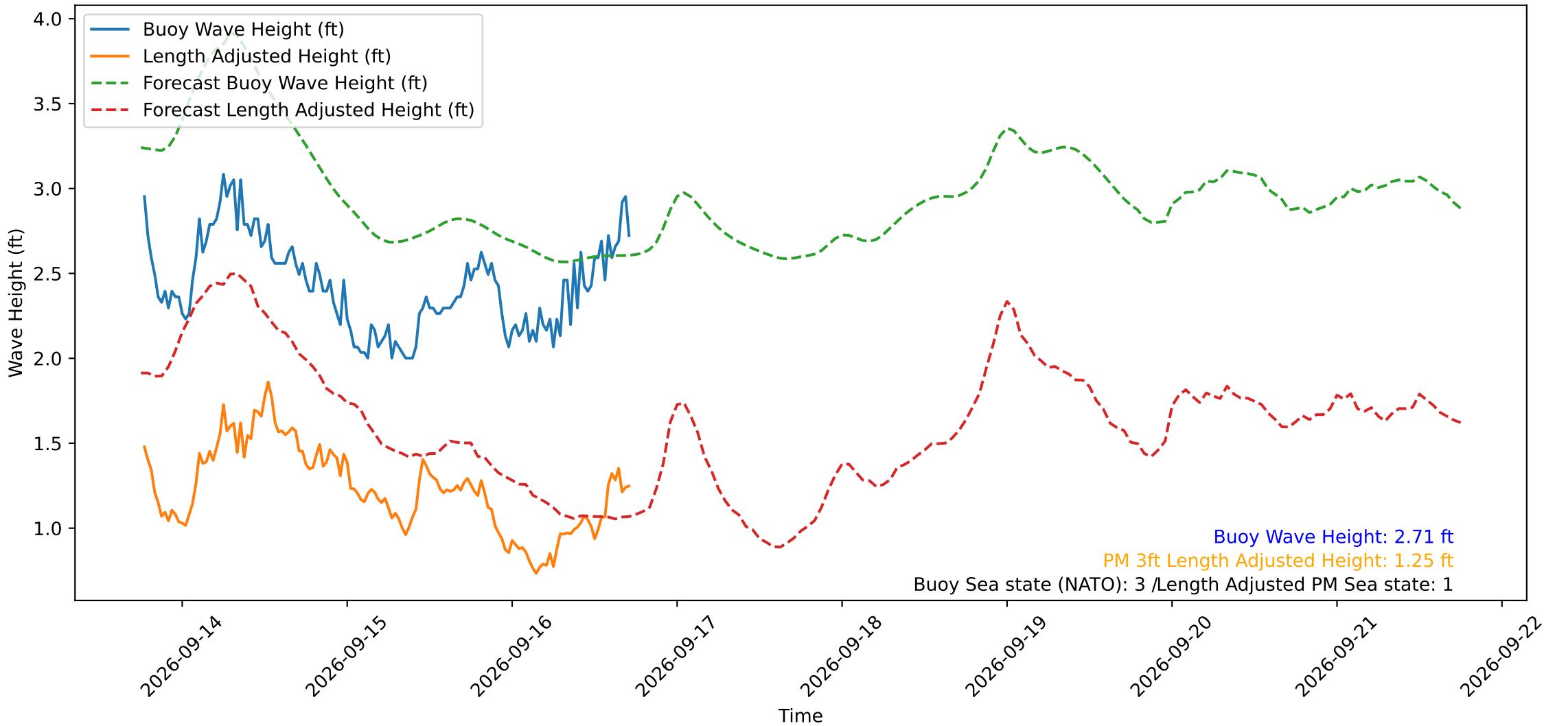
Wave Heights over Time for Red Beach at 2026-09-16 18:00:49
