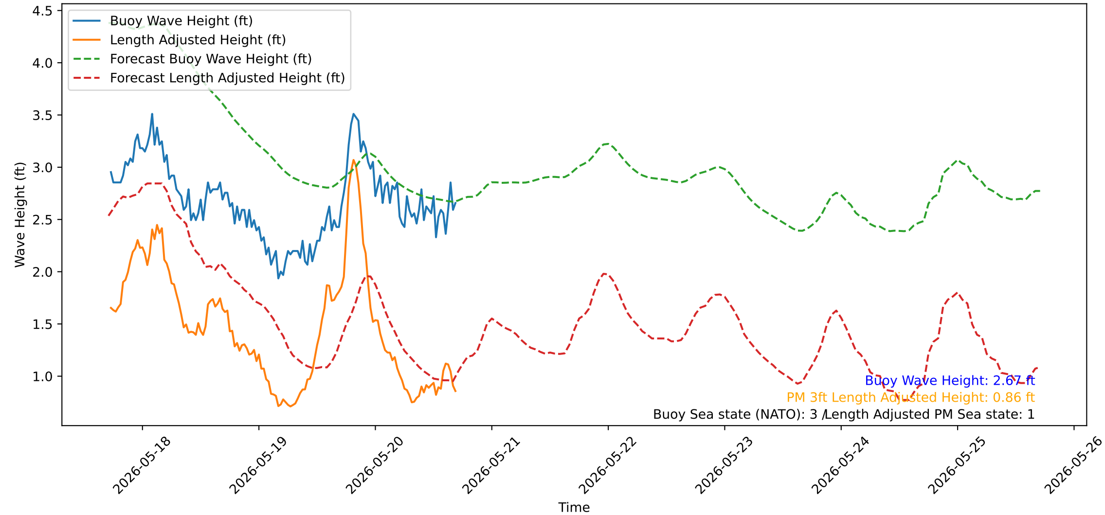
Wave Heights over Time for Red Beach at 2026-05-20 17:10:51
