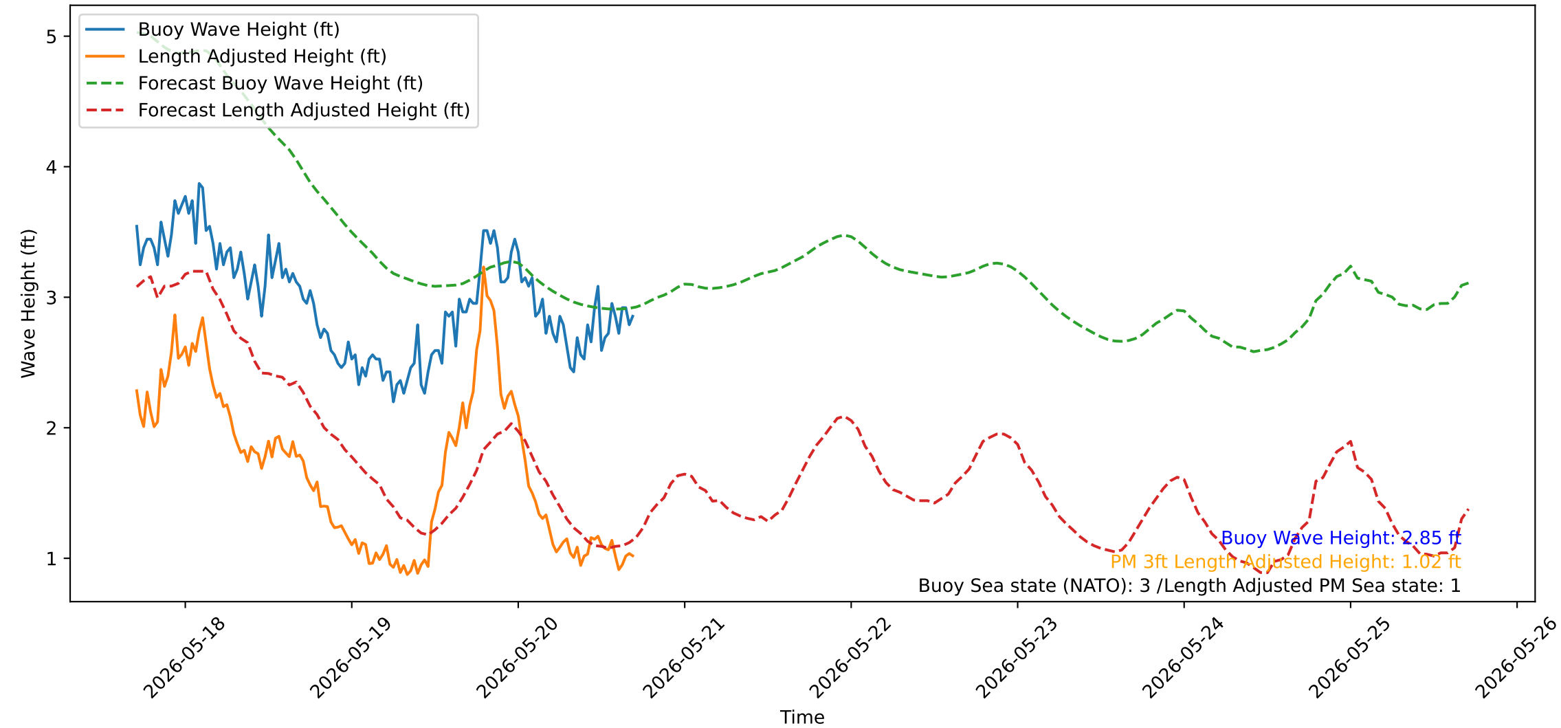
Wave Heights over Time for Oceanside Harbor at 2026-05-20 17:10:31
