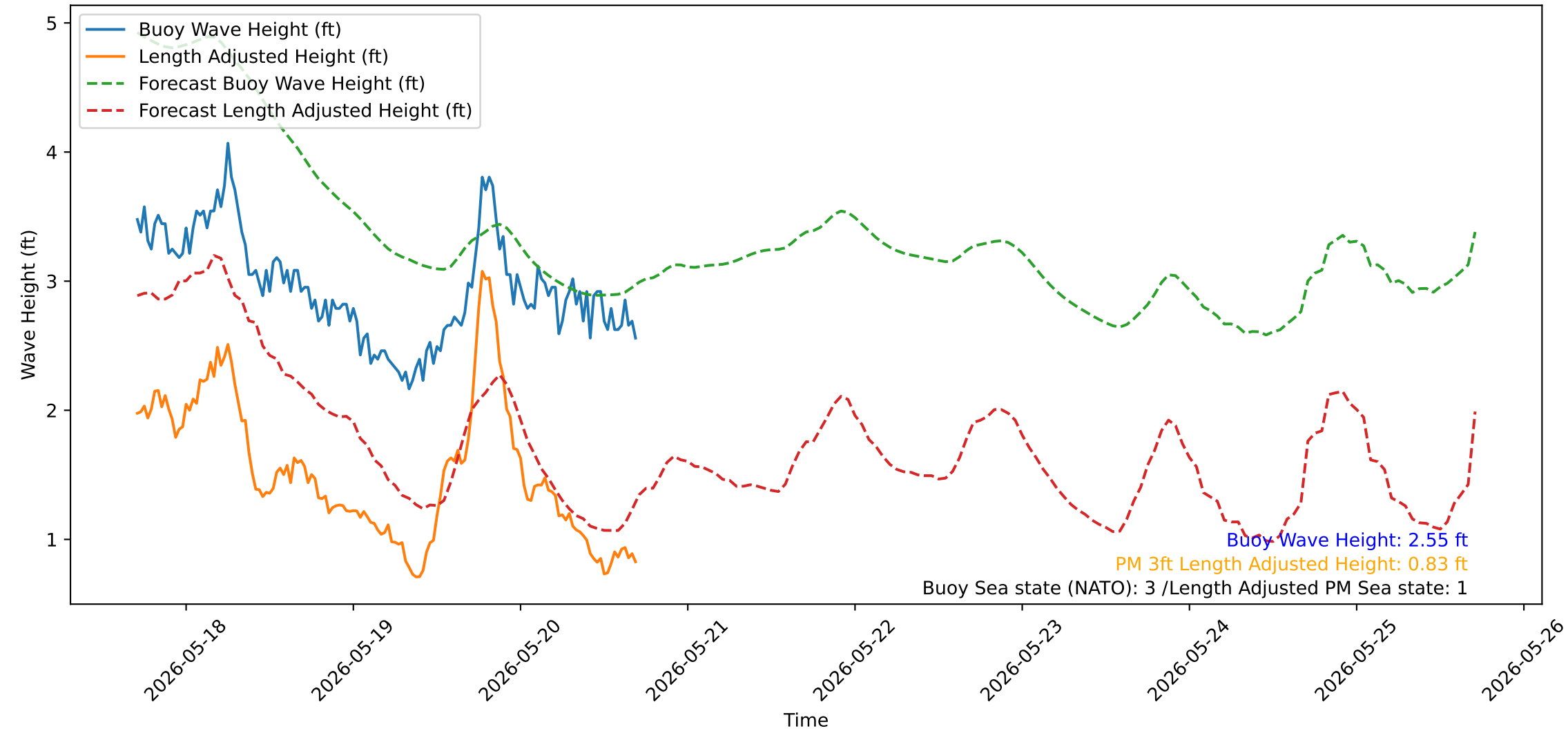
Wave Heights over Time for Green Beach at 2026-05-20 17:11:14
