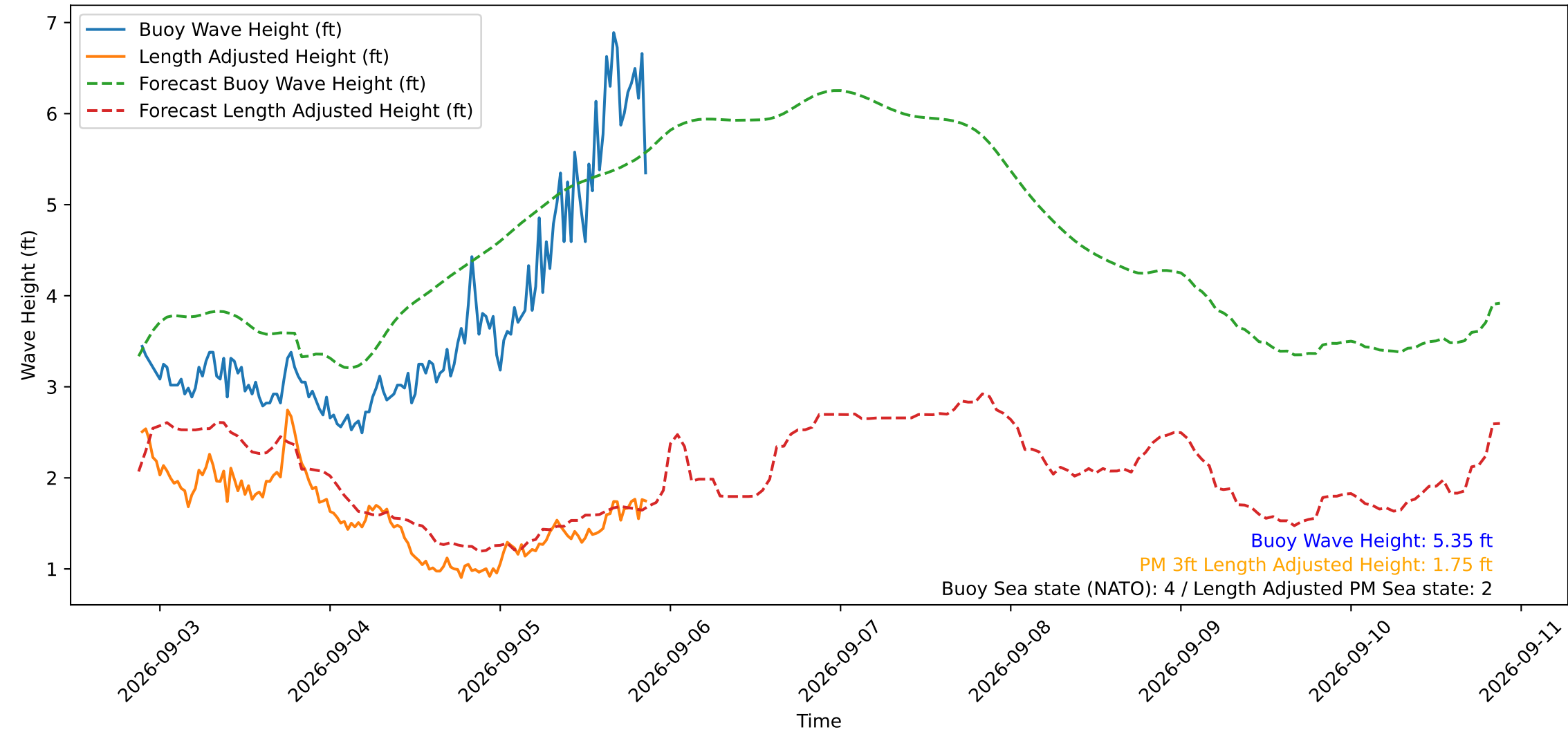
Wave Heights over Time for Green Beach at 2026-09-05 21:11:11
