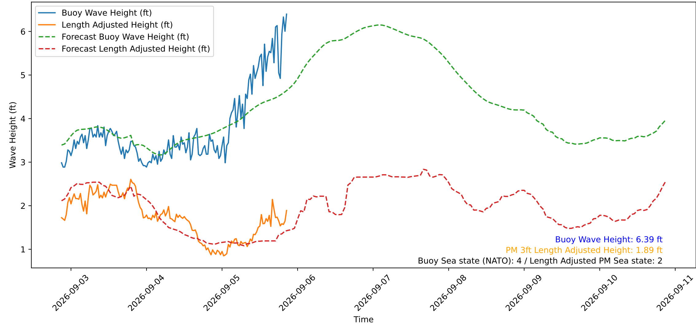
Wave Heights over Time for Oceanside Harbor at 2026-09-05 21:10:29
