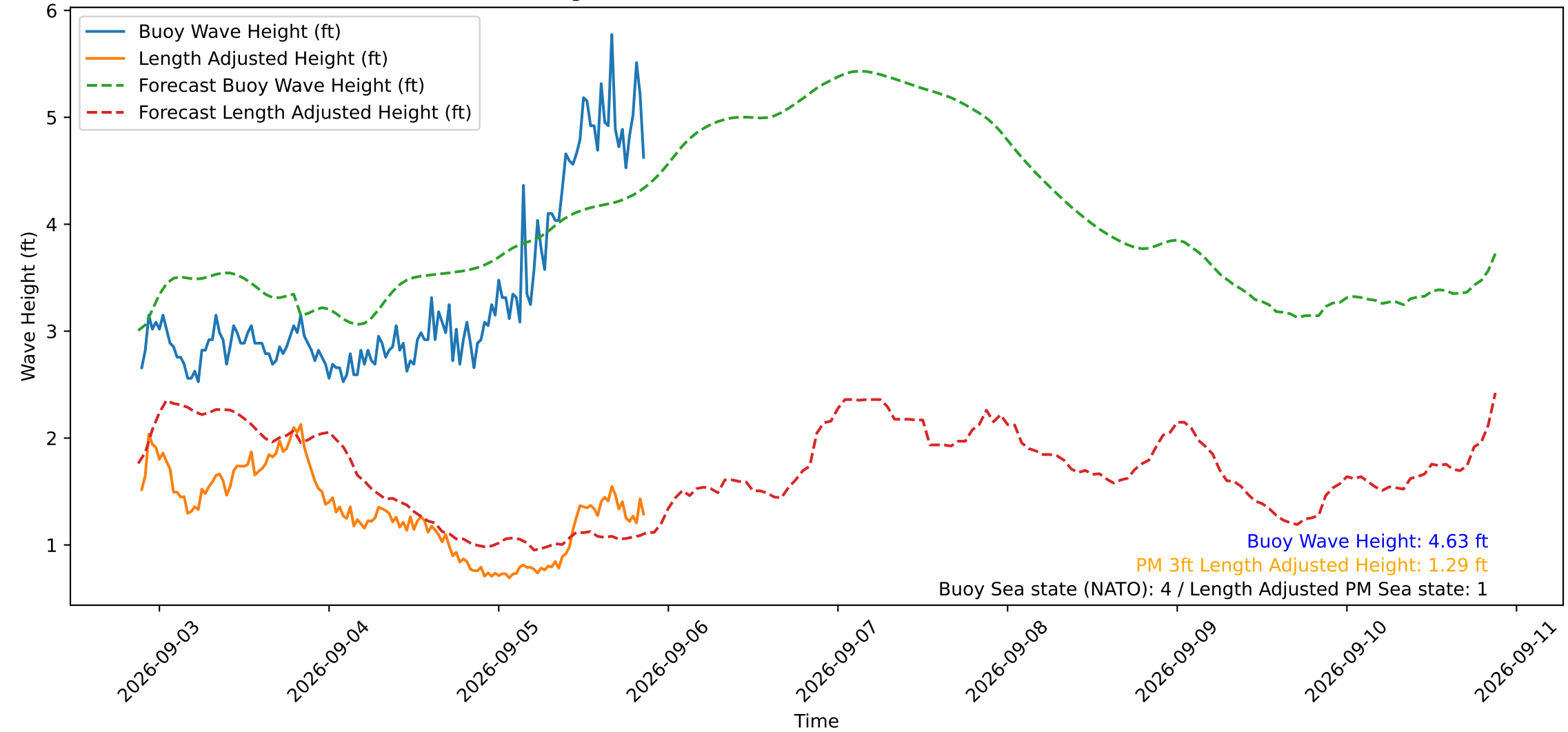
Wave Heights over Time for Red Beach at 2026-09-05 21:10:49
