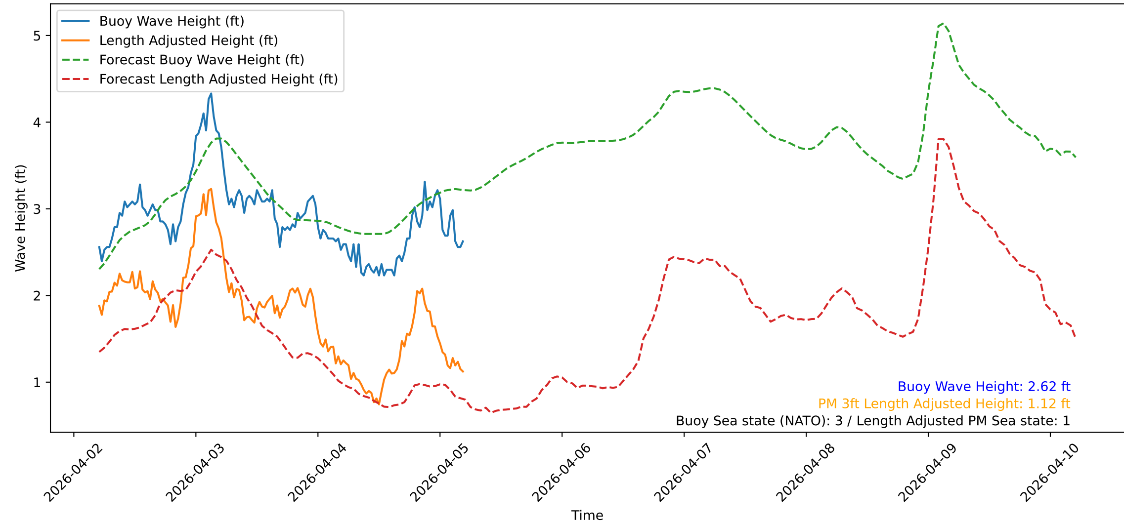
Wave Heights over Time for Green Beach at 2026-04-05 05:11:09
