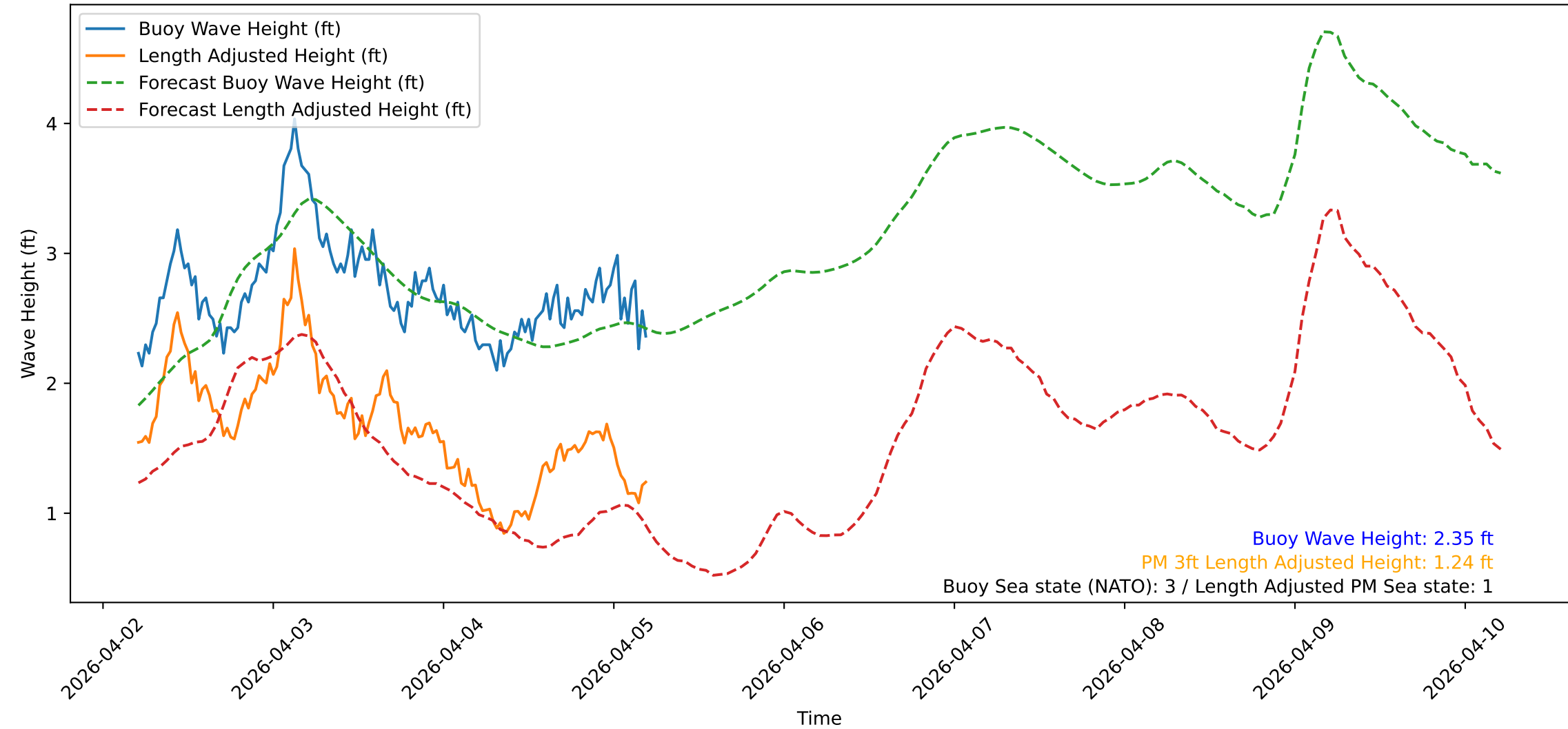
Wave Heights over Time for Oceanside Harbor at 2026-04-05 05:10:31
