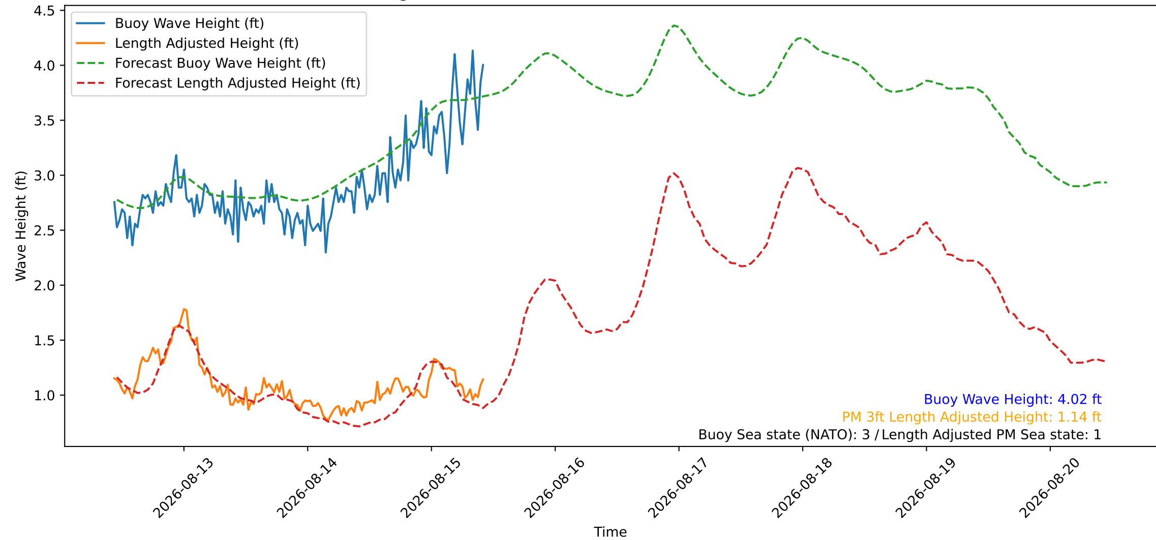
Wave Heights over Time for Oceanside Harbor at 2026-08-15 10:40:27
