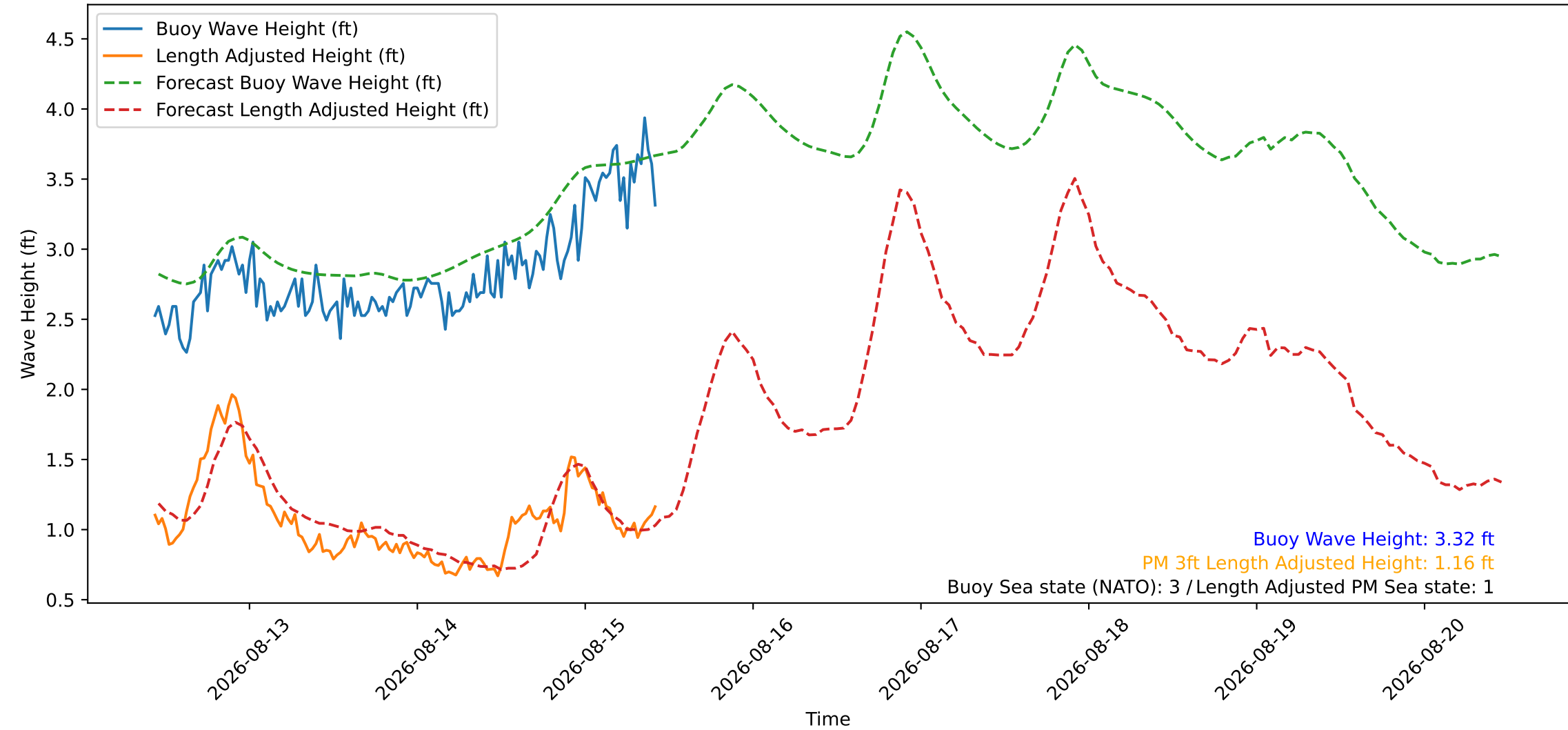
Wave Heights over Time for Green Beach at 2026-08-15 10:41:09
