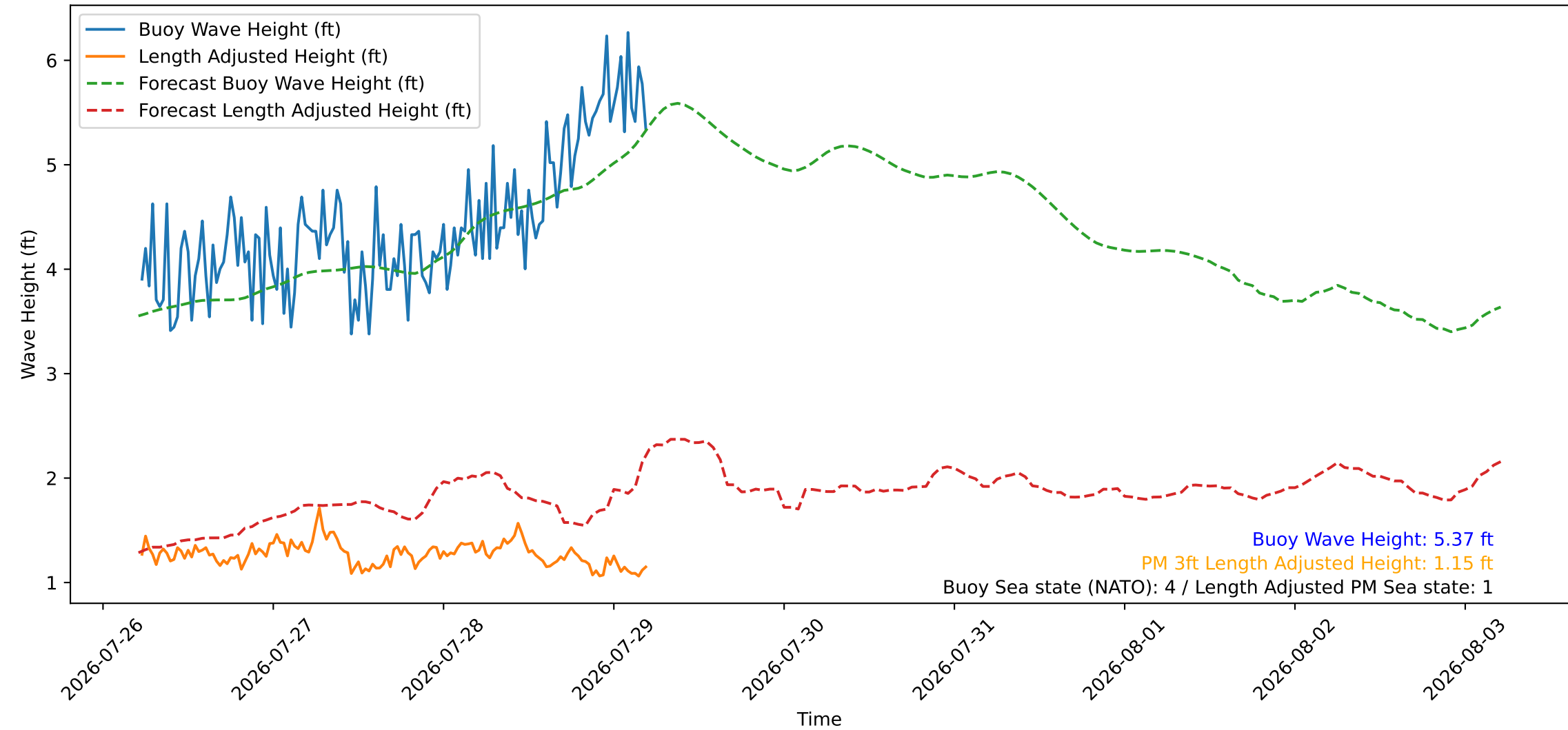
Wave Heights over Time for Green Beach at 2026-07-29 05:21:10
