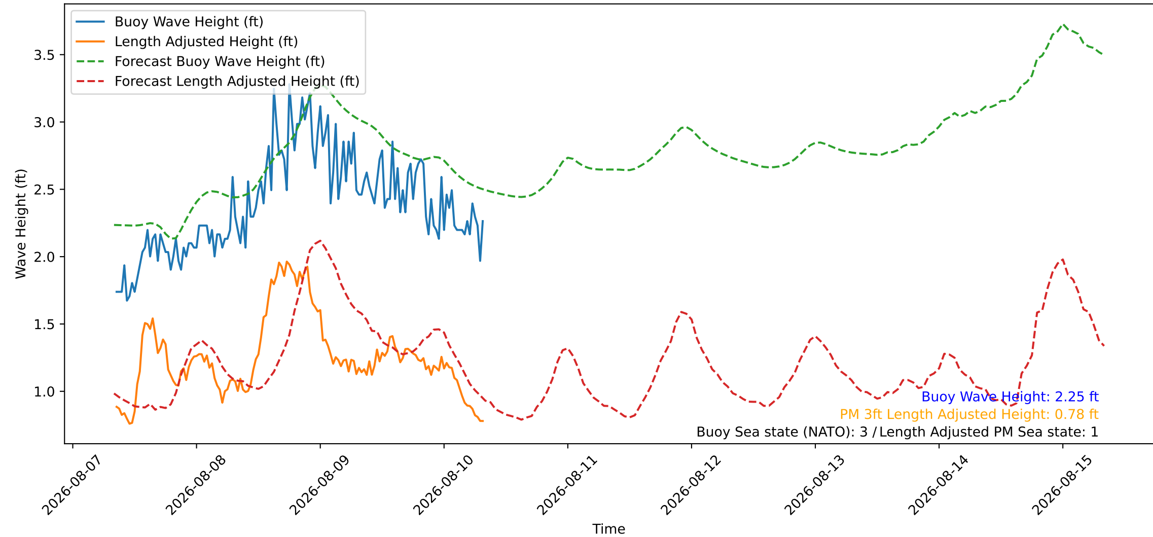
Wave Heights over Time for Oceanside Harbor at 2026-08-10 08:20:26
