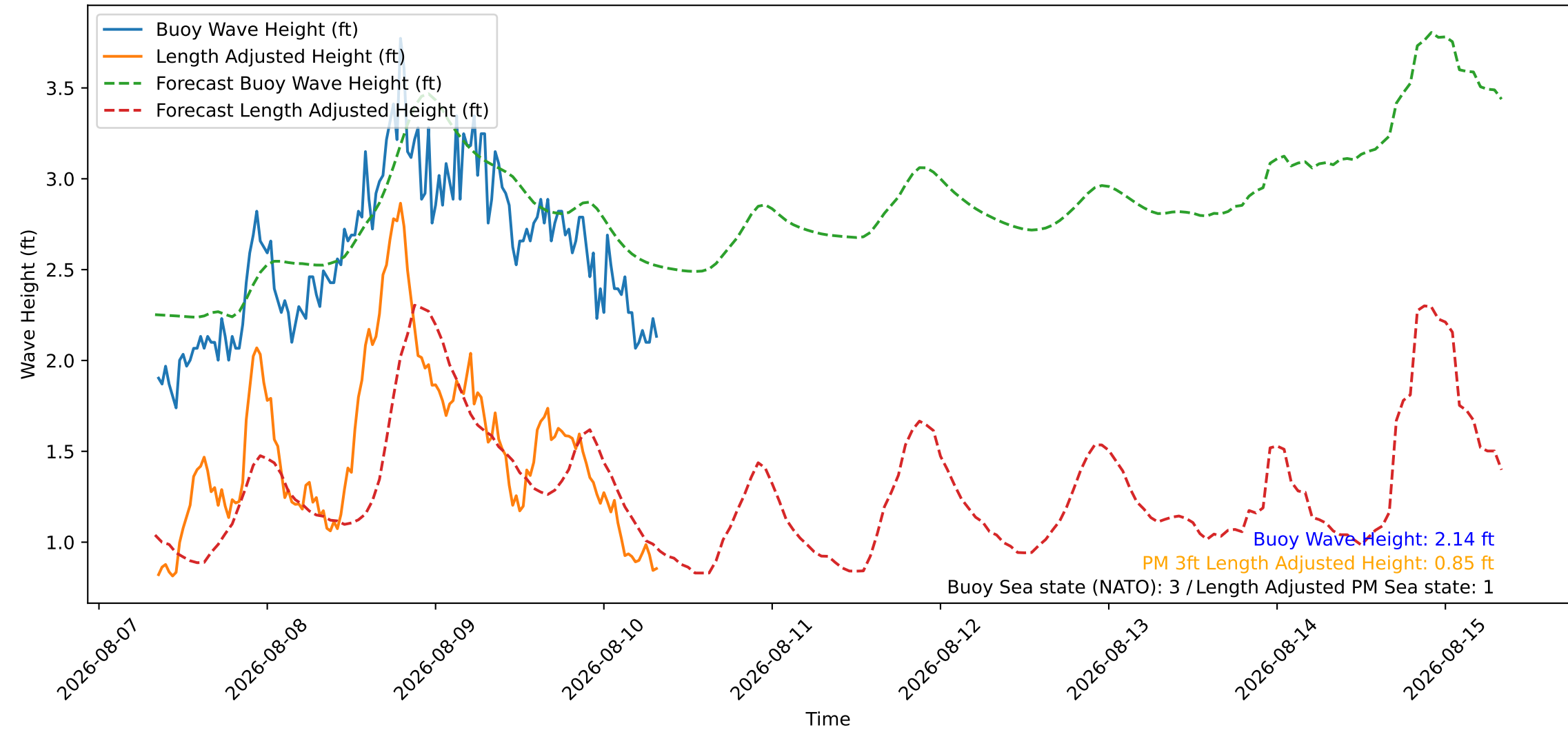
Wave Heights over Time for Green Beach at 2026-08-10 08:21:10
