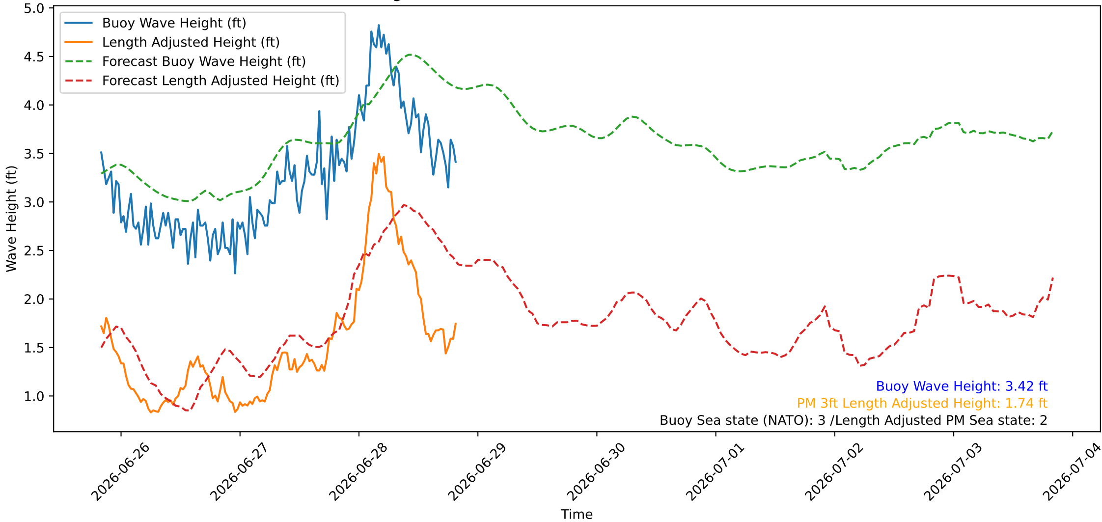
Wave Heights over Time for Green Beach at 2026-06-28 20:11:07
