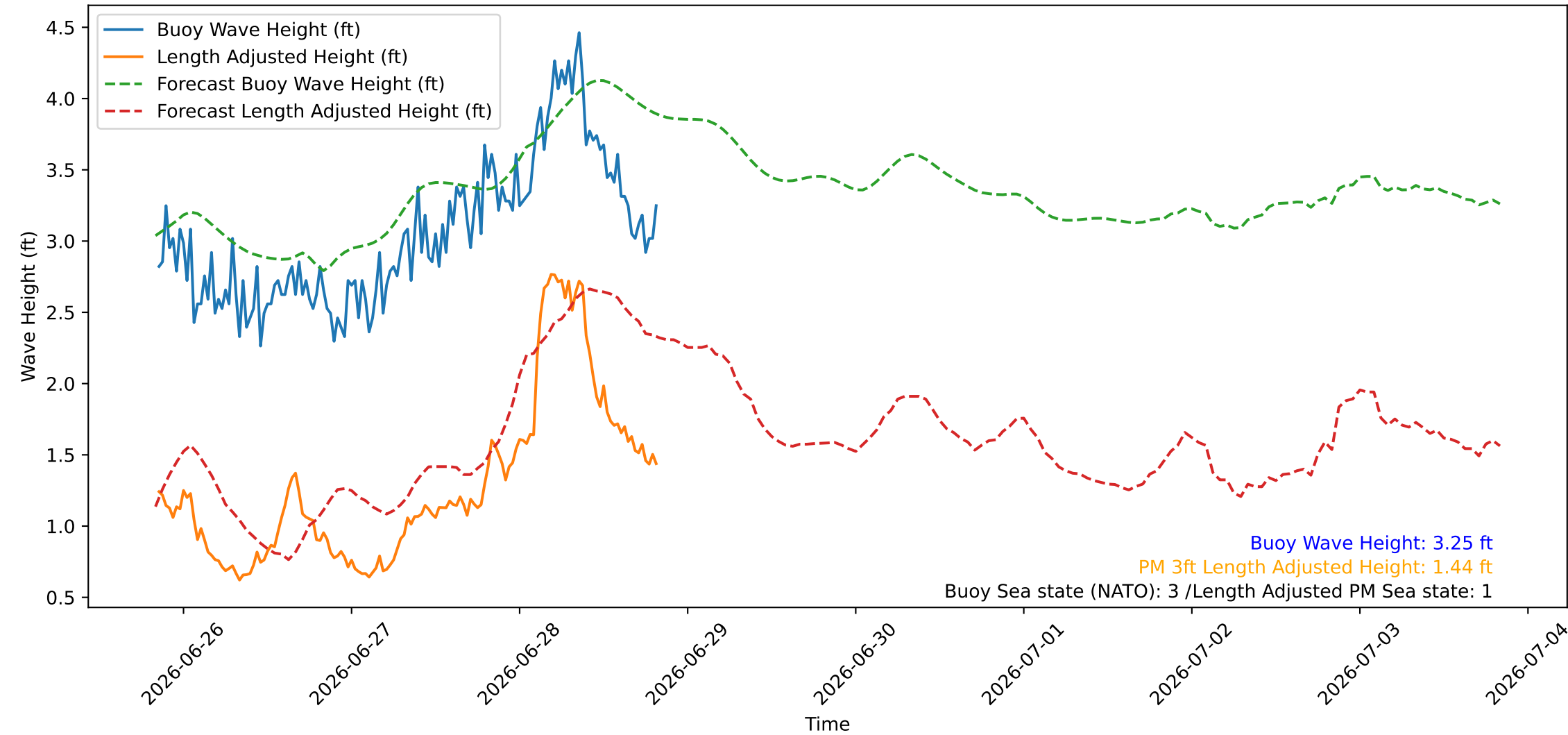
Wave Heights over Time for Red Beach at 2026-06-28 20:10:45
