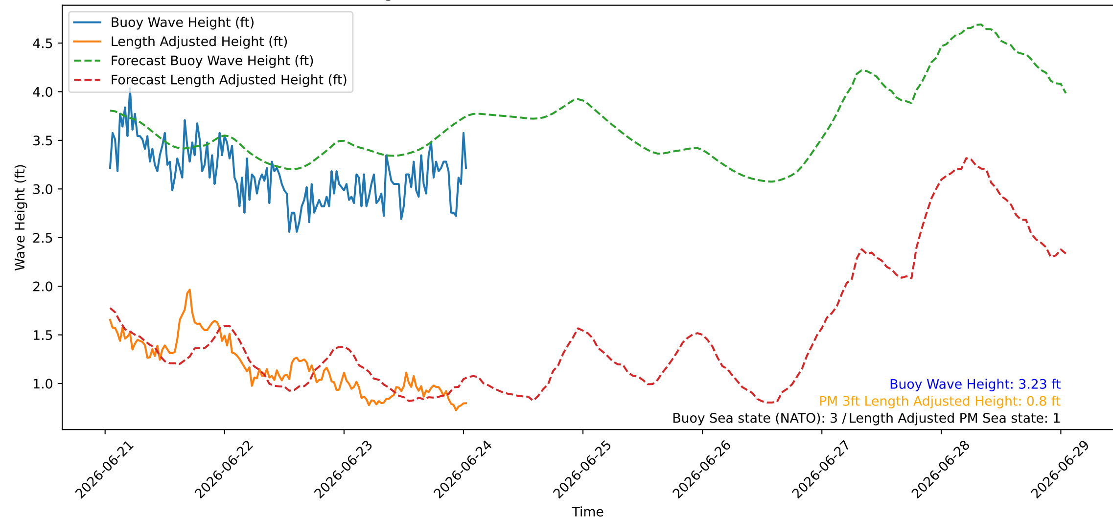
Wave Heights over Time for Oceanside Harbor at 2026-06-24 01:00:26
