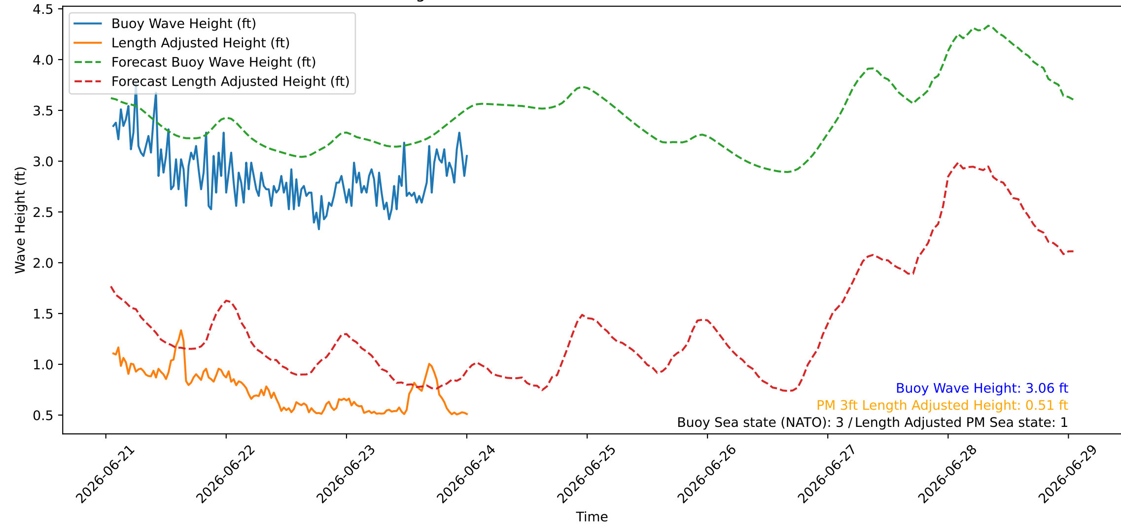
Wave Heights over Time for Red Beach at 2026-06-24 01:00:45
