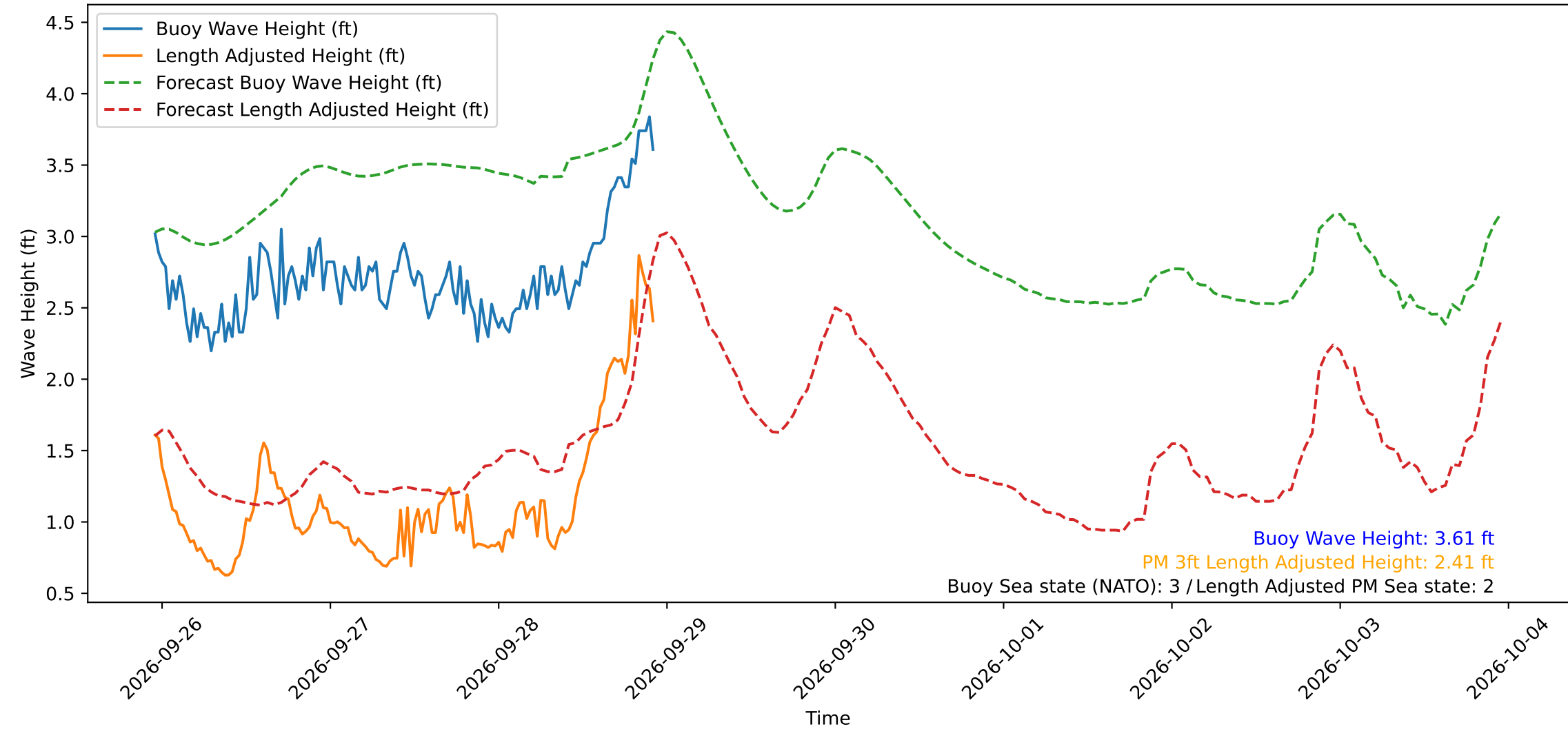
Wave Heights over Time for Red Beach at 2026-09-28 22:40:50
