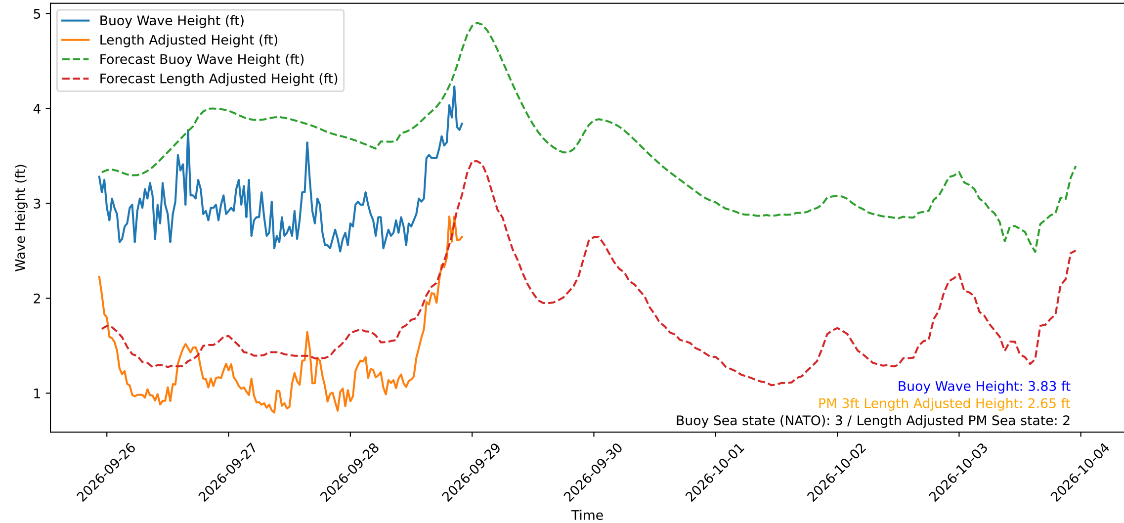
Wave Heights over Time for Oceanside Harbor at 2026-09-28 22:40:30
