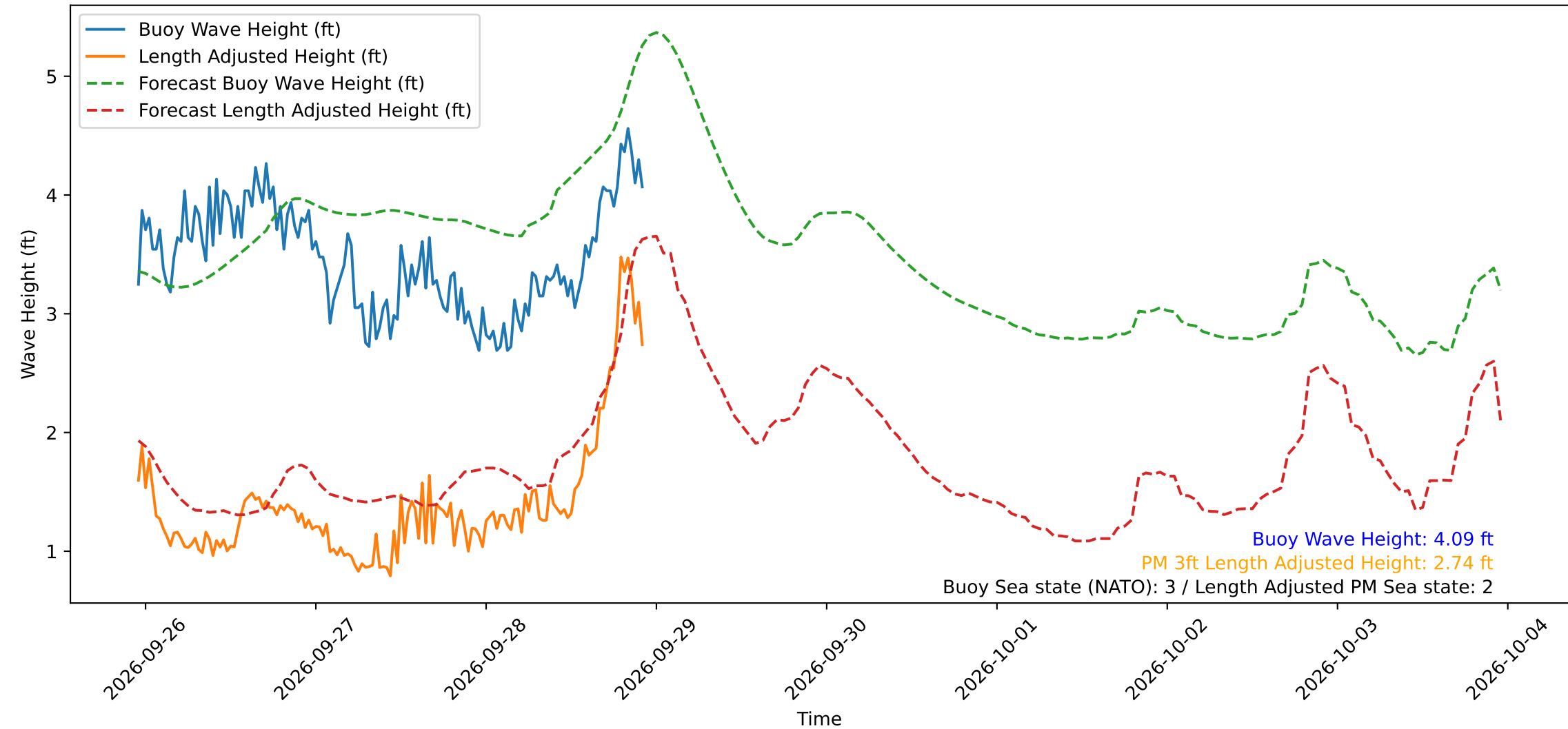
Wave Heights over Time for Green Beach at 2026-09-28 22:41:13
