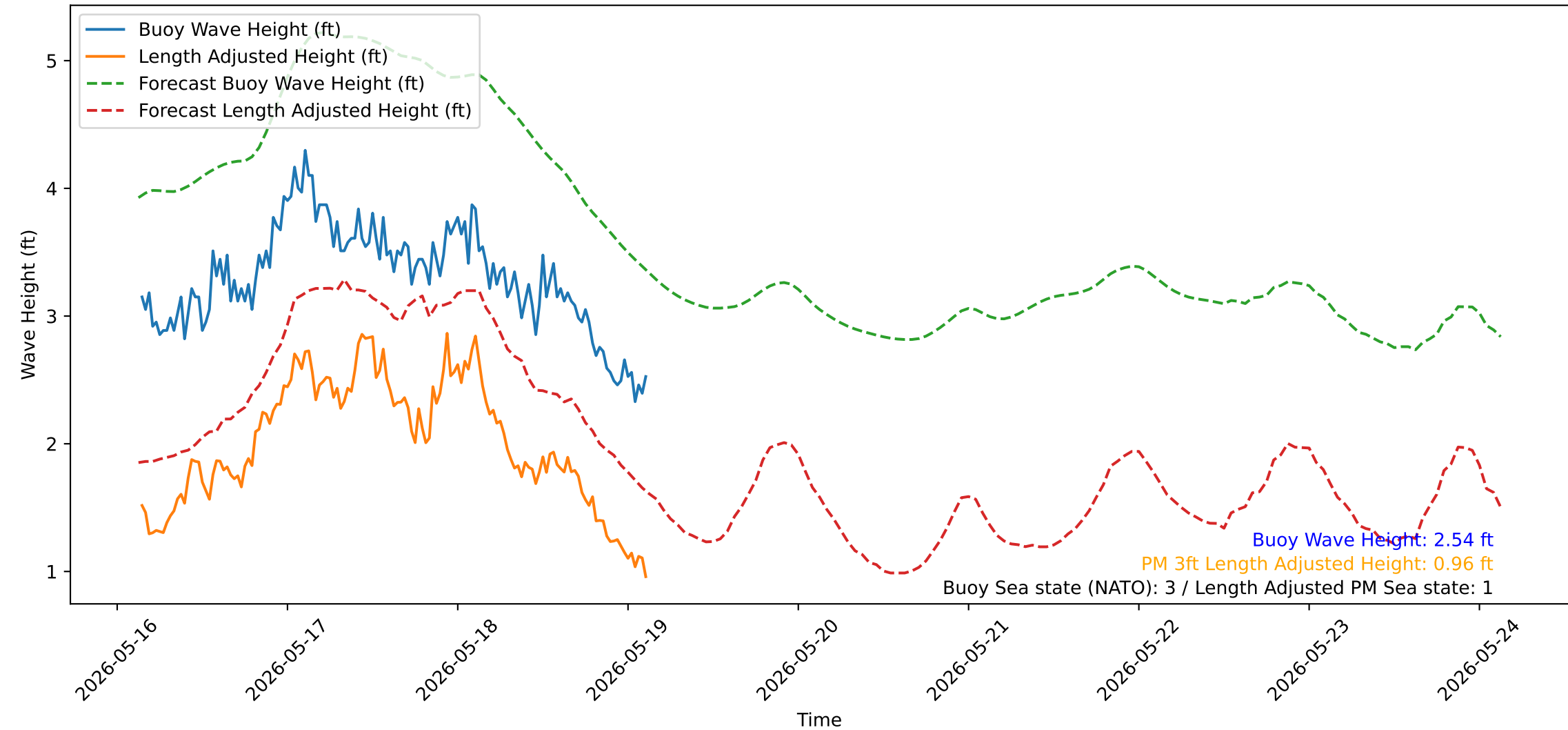
Wave Heights over Time for Oceanside Harbor at 2026-05-19 03:20:32
