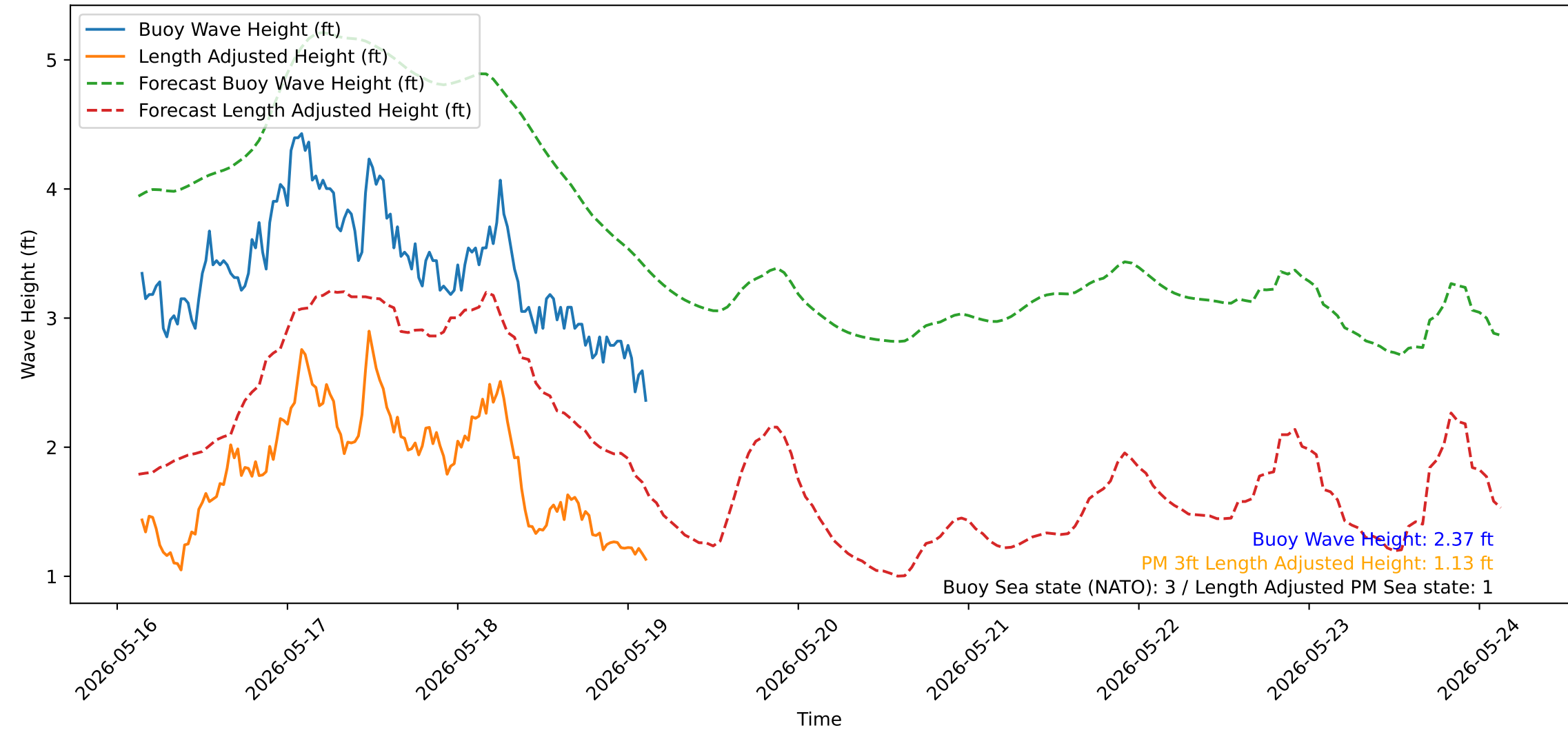
Wave Heights over Time for Green Beach at 2026-05-19 03:21:15
