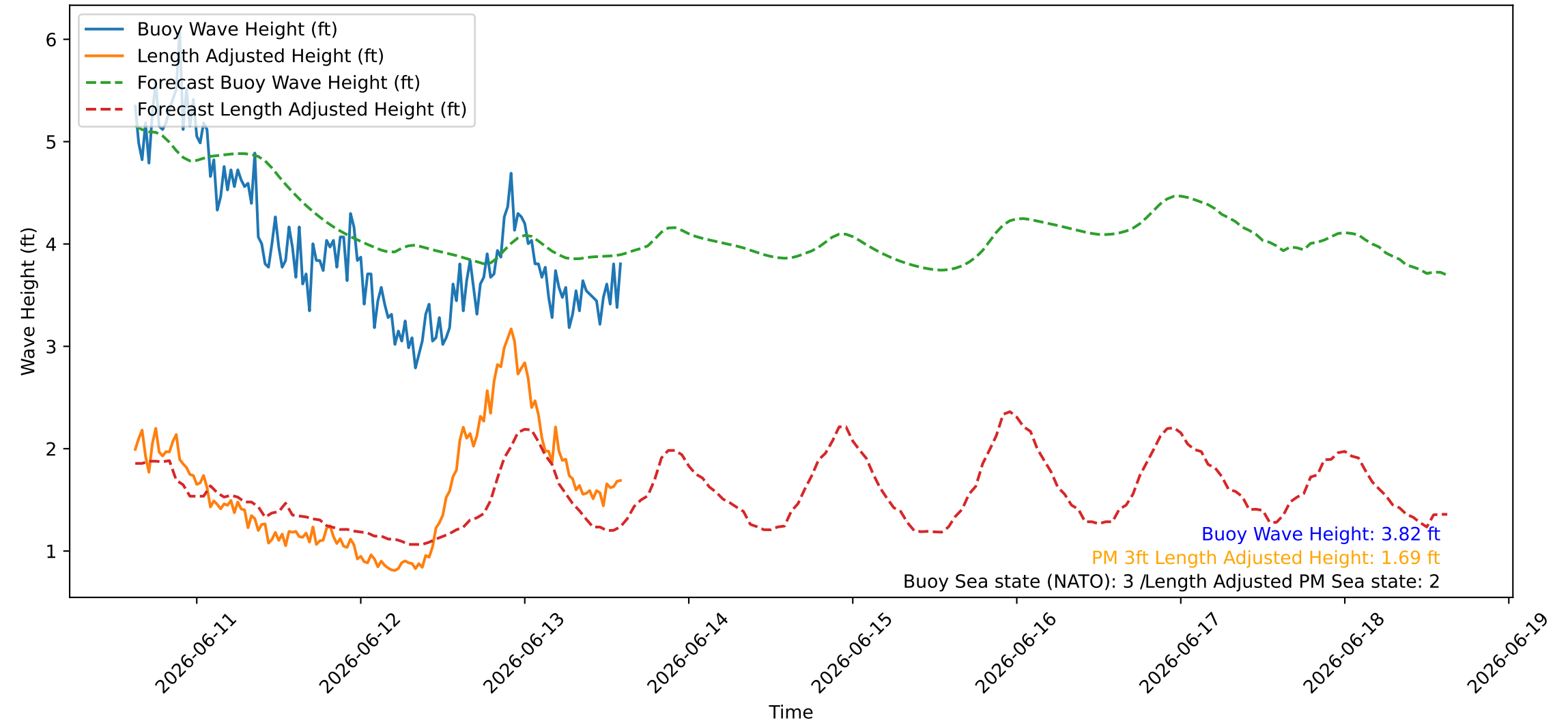
Wave Heights over Time for Oceanside Harbor at 2026-06-13 14:50:27
