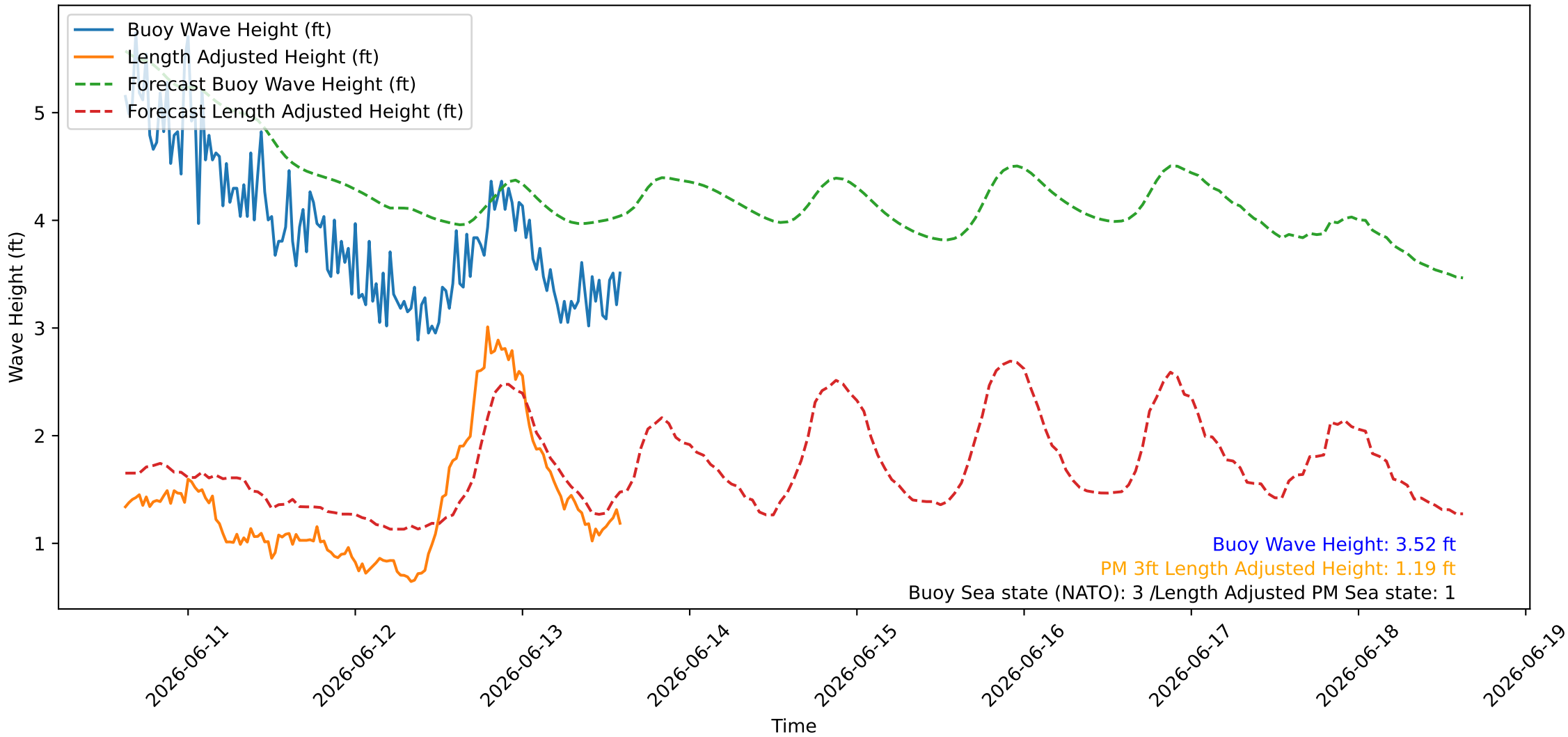
Wave Heights over Time for Green Beach at 2026-06-13 14:51:10
