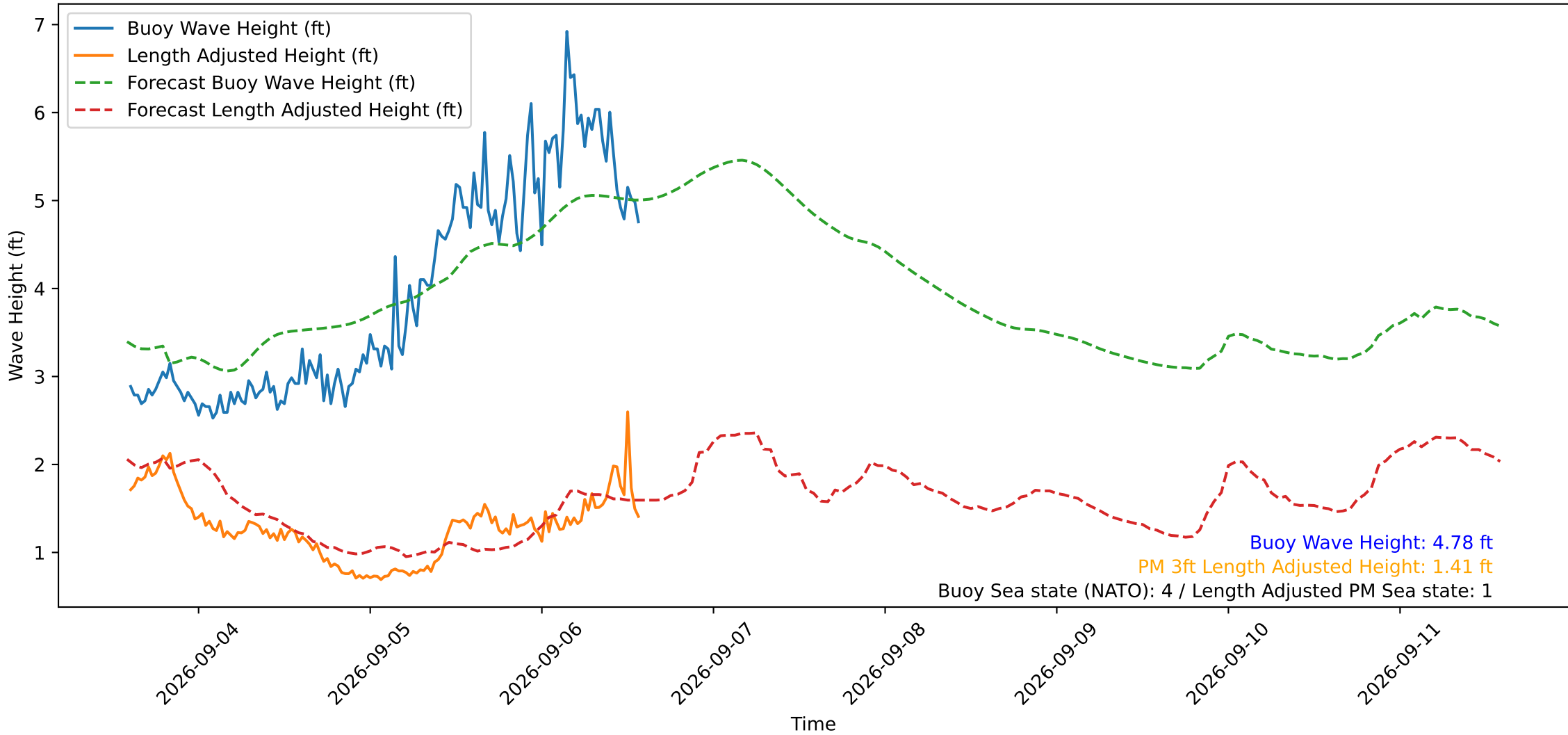
Wave Heights over Time for Red Beach at 2026-09-06 14:20:51
