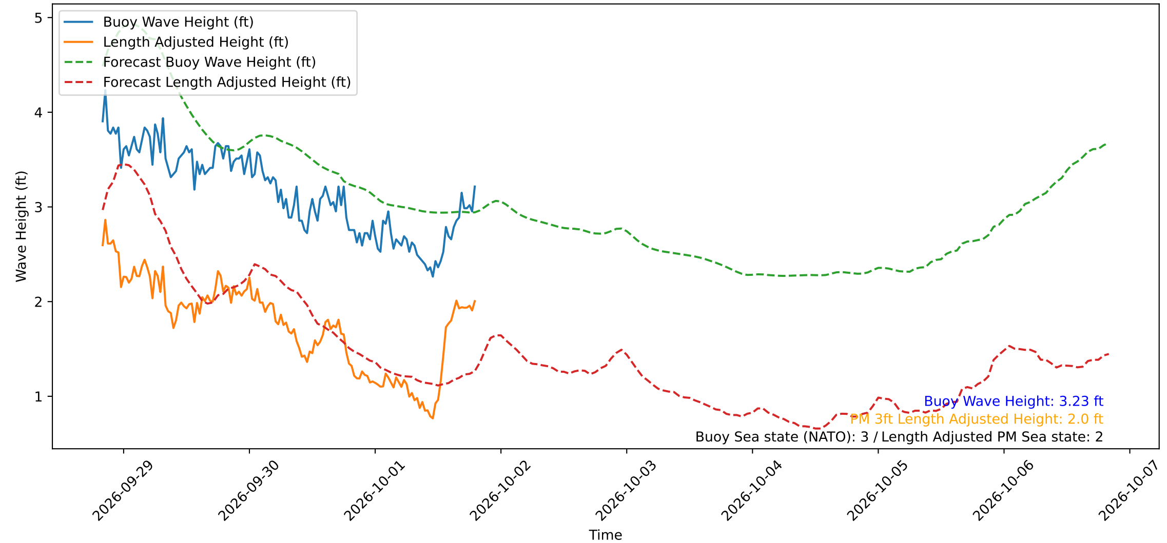
Wave Heights over Time for Oceanside Harbor at 2026-10-01 20:10:30
