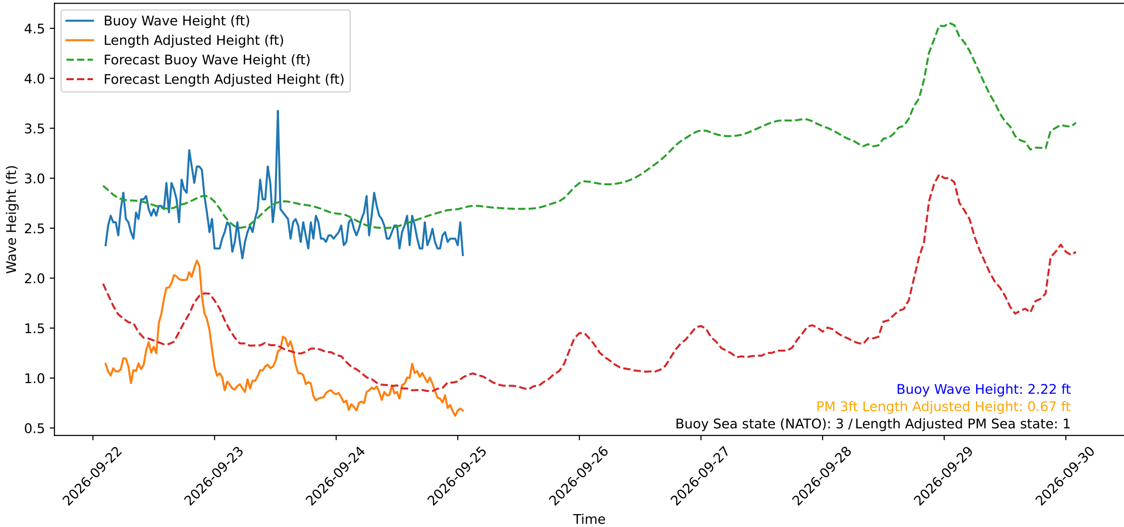
Wave Heights over Time for Red Beach at 2026-09-25 02:00:49
