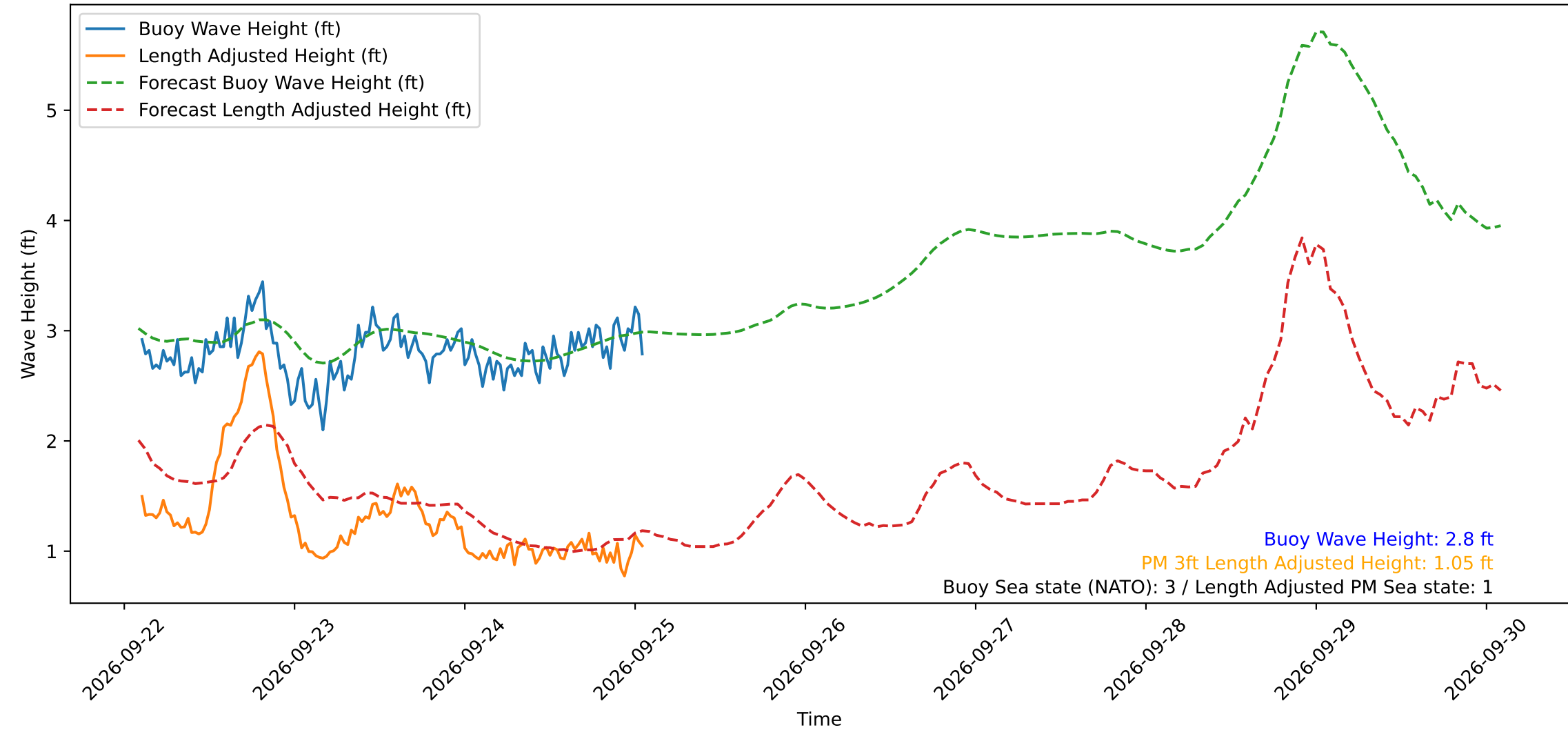
Wave Heights over Time for Green Beach at 2026-09-25 02:01:11
