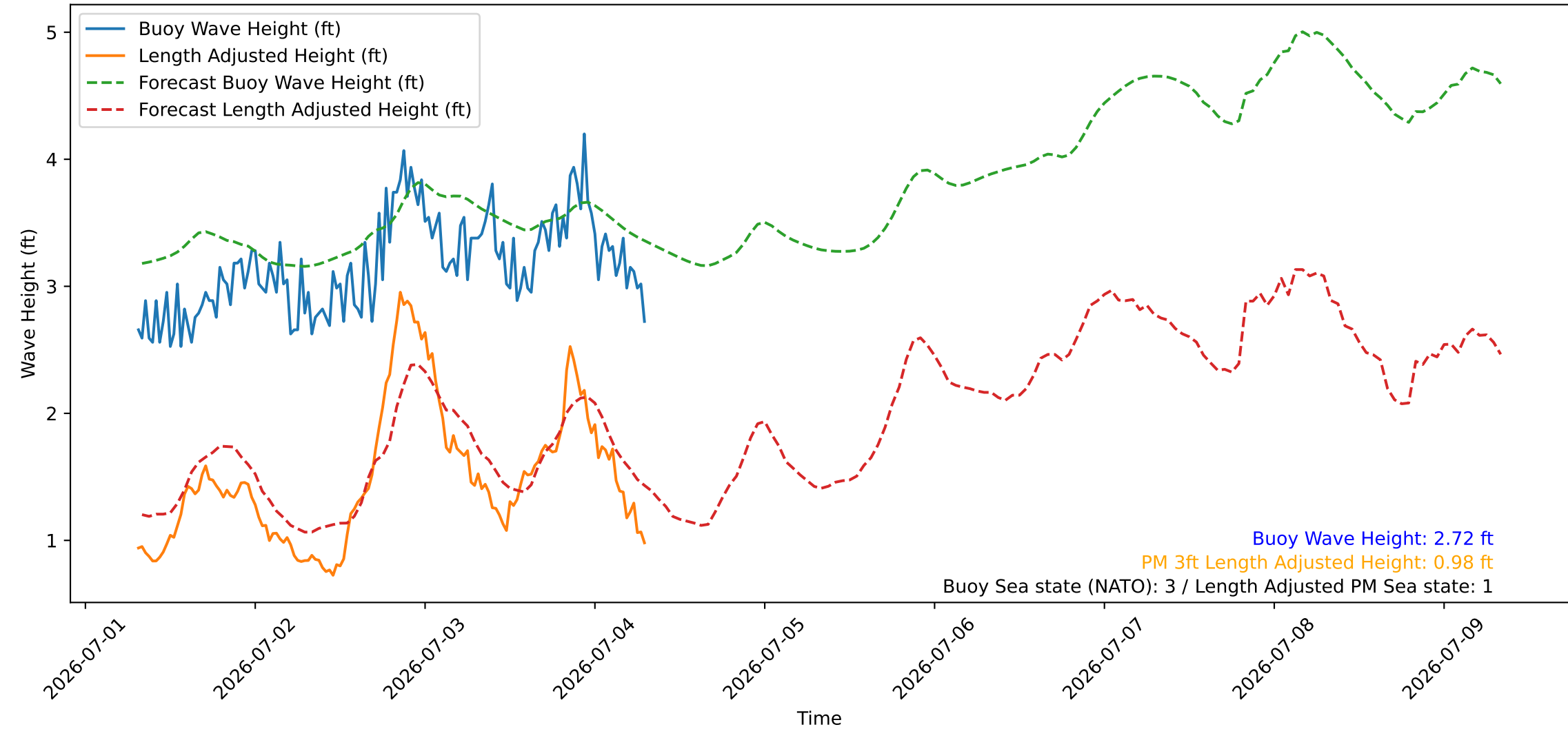
Wave Heights over Time for Green Beach at 2026-07-04 07:41:09
