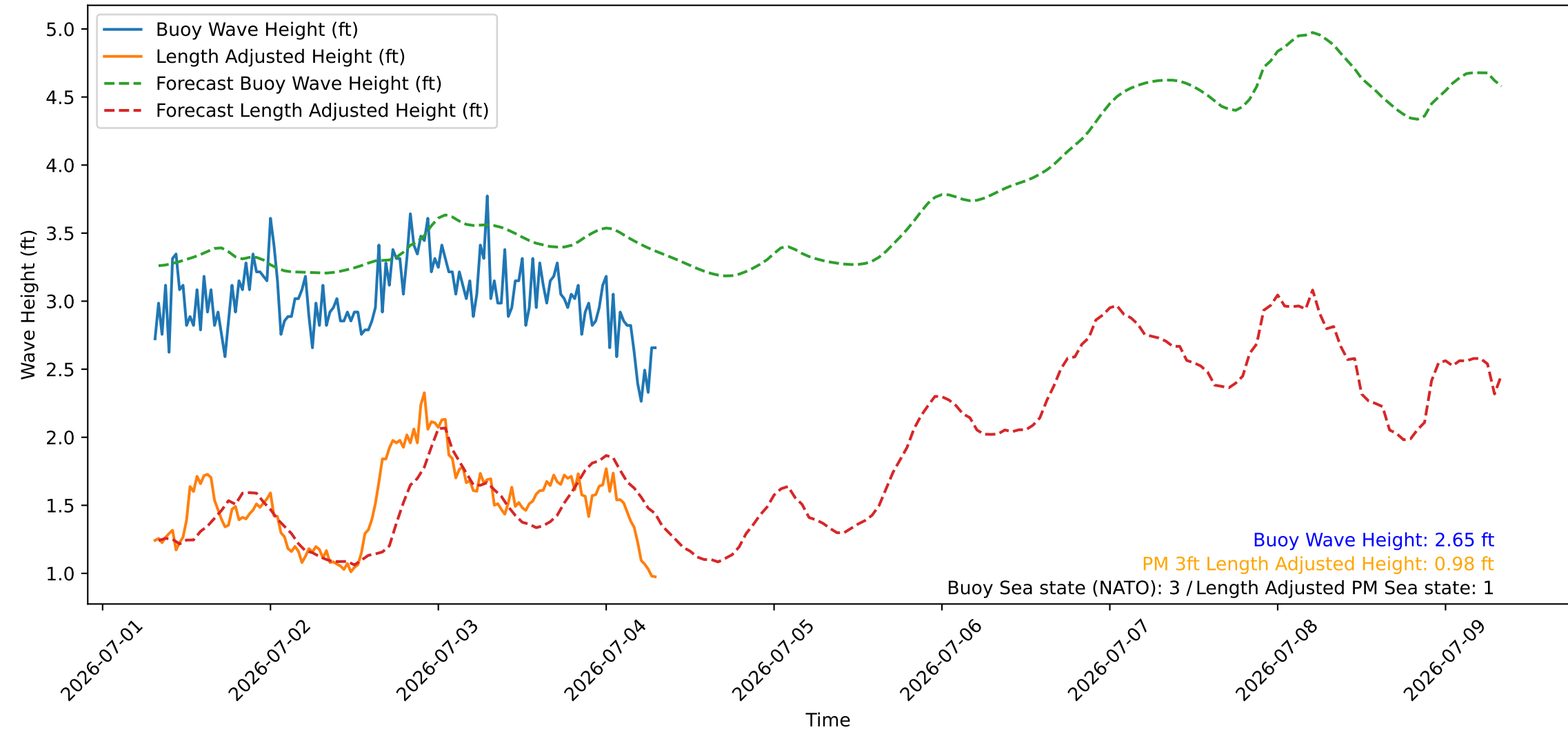
Wave Heights over Time for Oceanside Harbor at 2026-07-04 07:40:27
