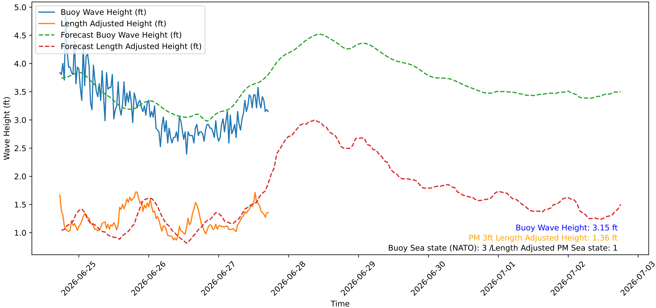
Wave Heights over Time for Oceanside Harbor at 2026-06-27 17:40:26
