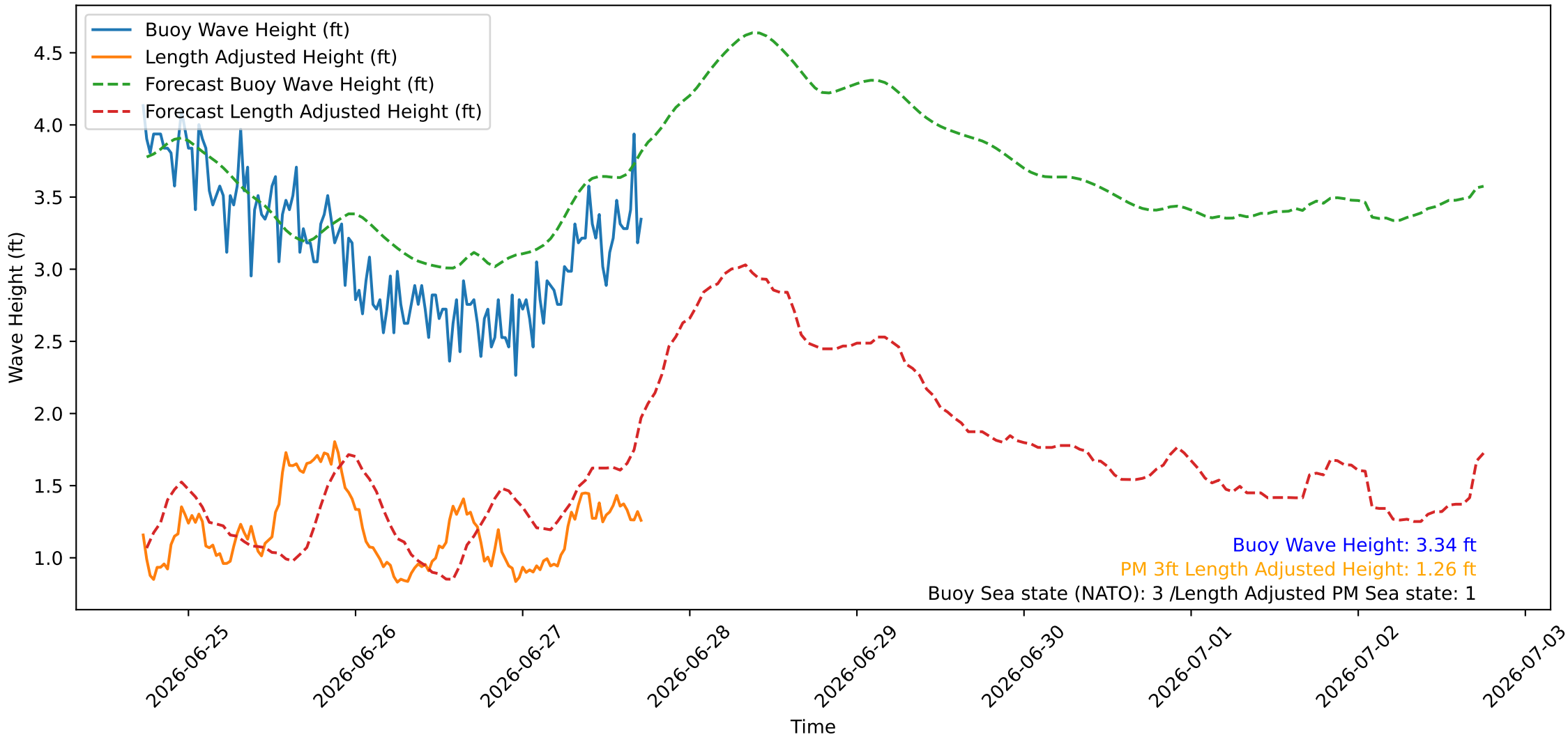
Wave Heights over Time for Green Beach at 2026-06-27 17:41:09
