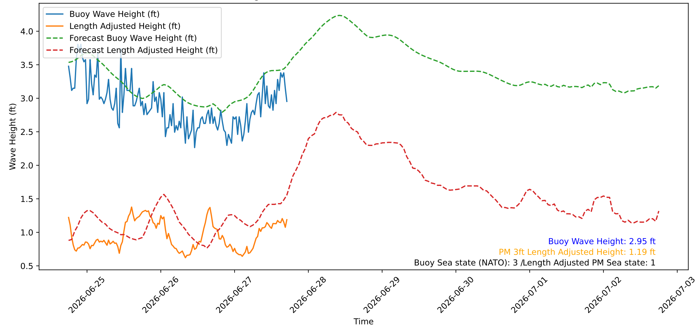
Wave Heights over Time for Red Beach at 2026-06-27 17:40:46
