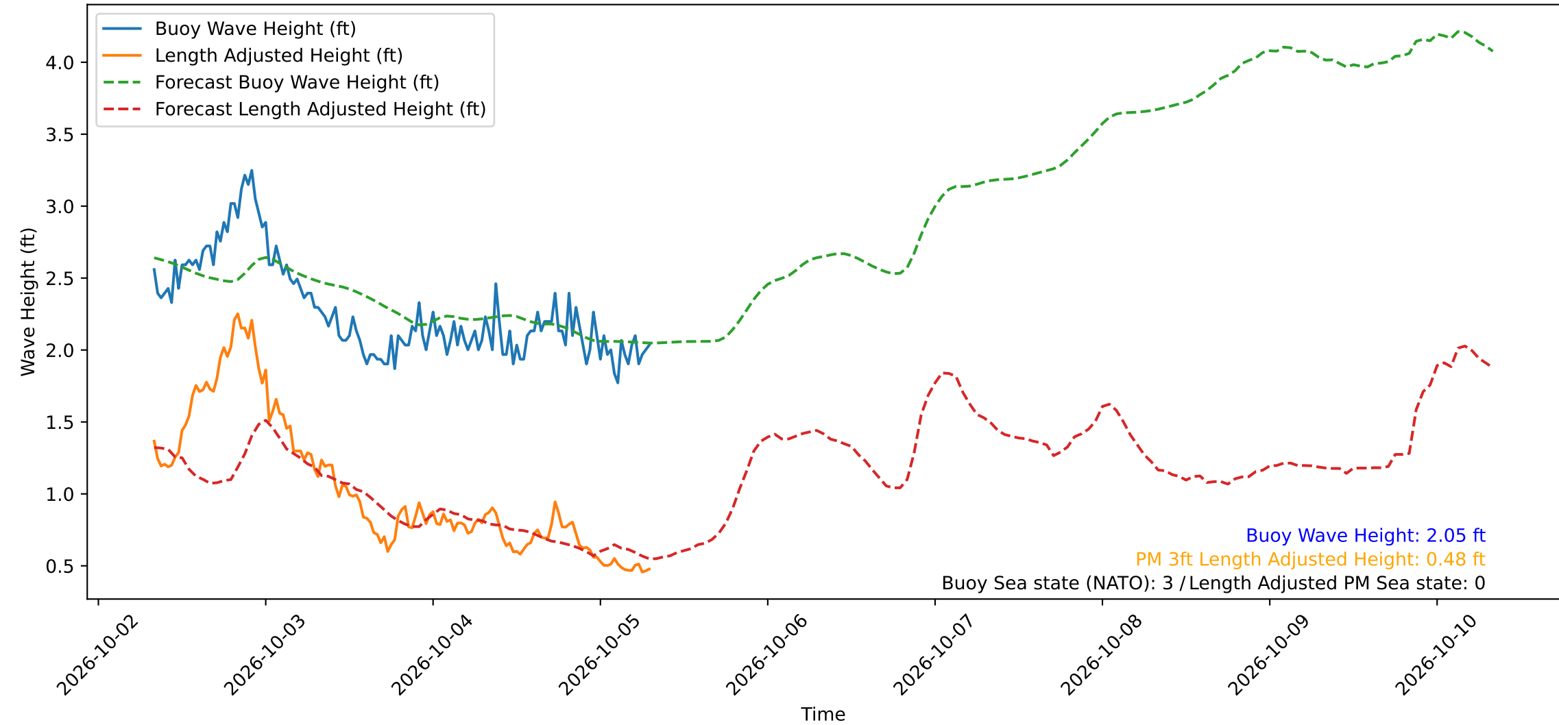
Wave Heights over Time for Red Beach at 2026-10-05 07:50:50
