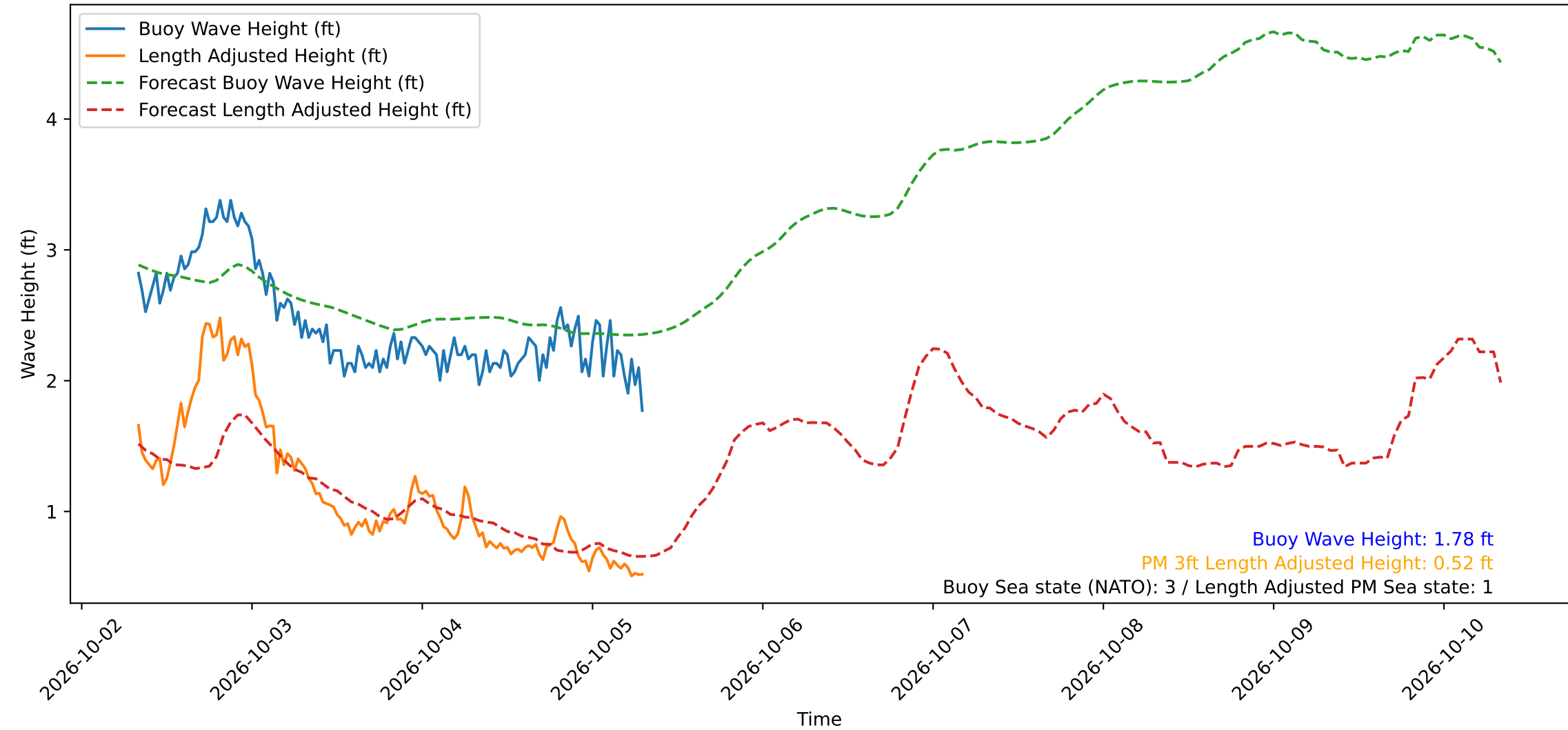
Wave Heights over Time for Green Beach at 2026-10-05 07:51:14
