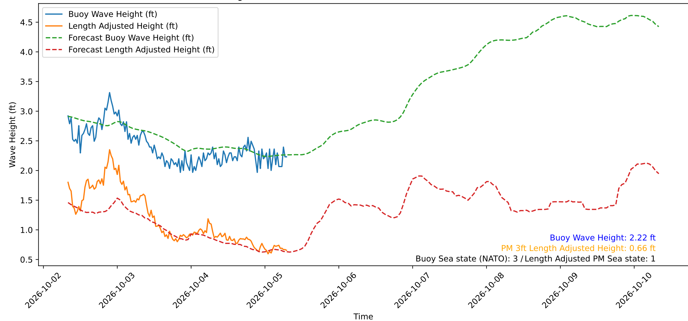
Wave Heights over Time for Oceanside Harbor at 2026-10-05 07:50:29
