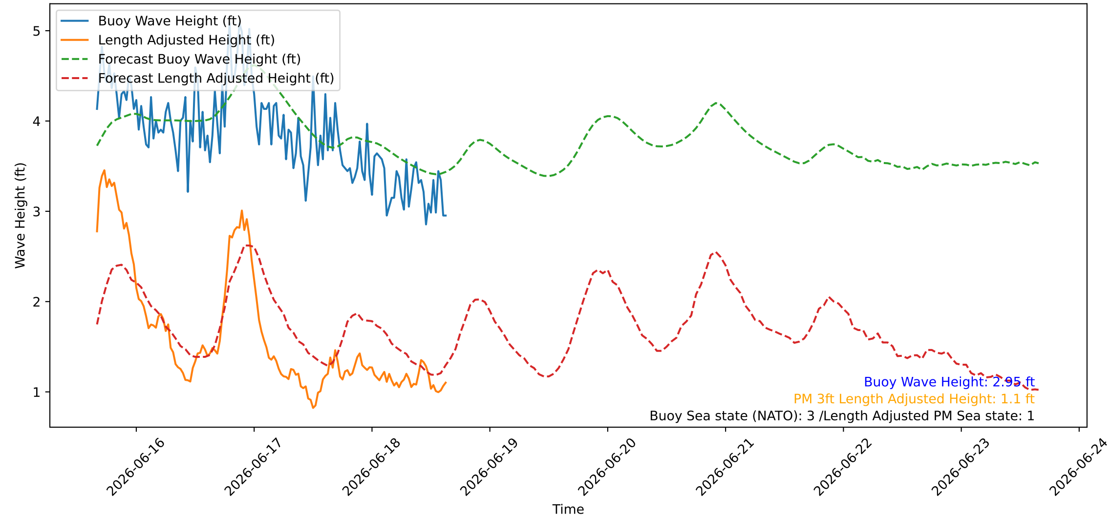
Wave Heights over Time for Green Beach at 2026-06-18 16:01:08
