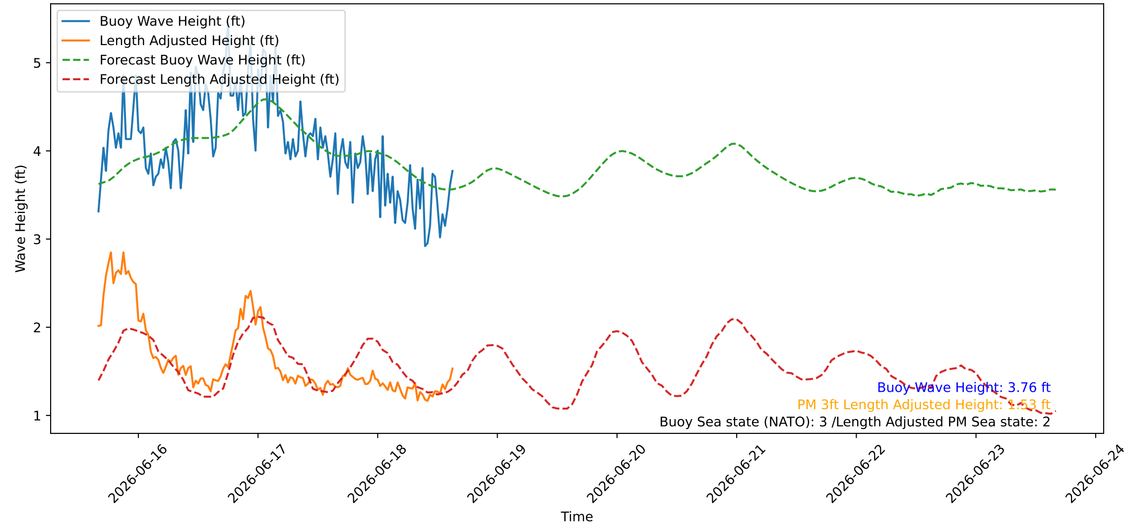
Wave Heights over Time for Oceanside Harbor at 2026-06-18 16:00:26
