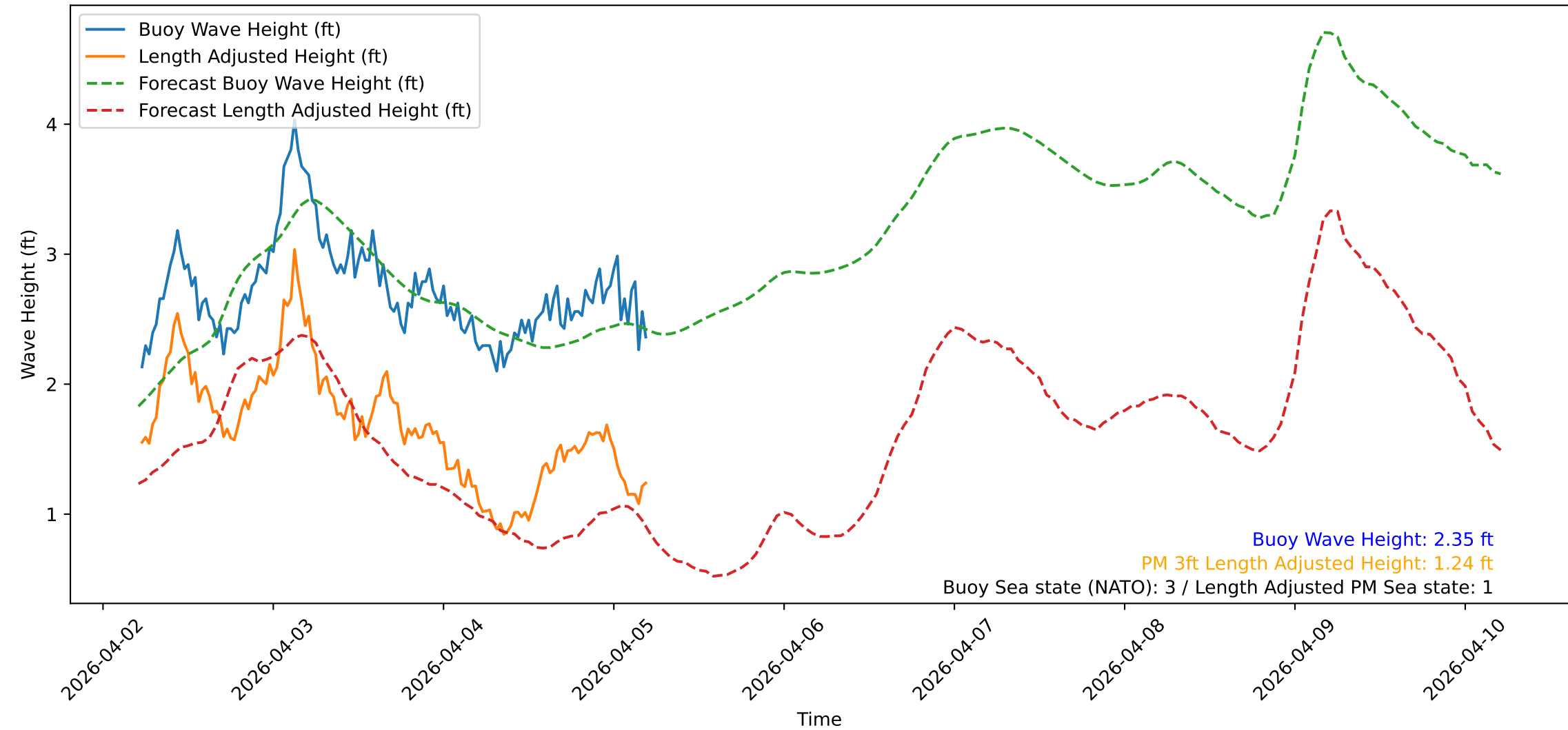
Wave Heights over Time for Oceanside Harbor at 2026-04-05 05:20:31
