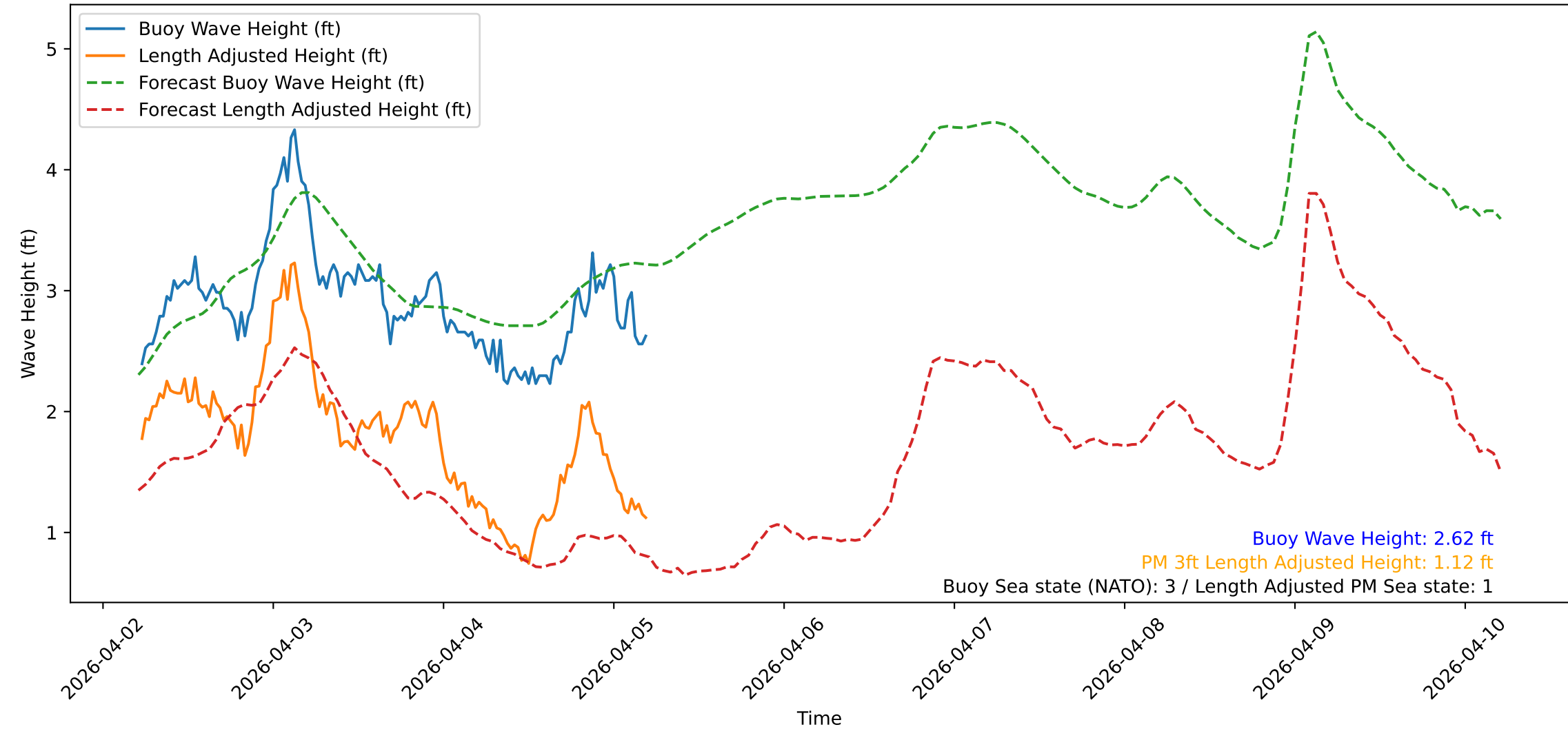
Wave Heights over Time for Green Beach at 2026-04-05 05:21:09
