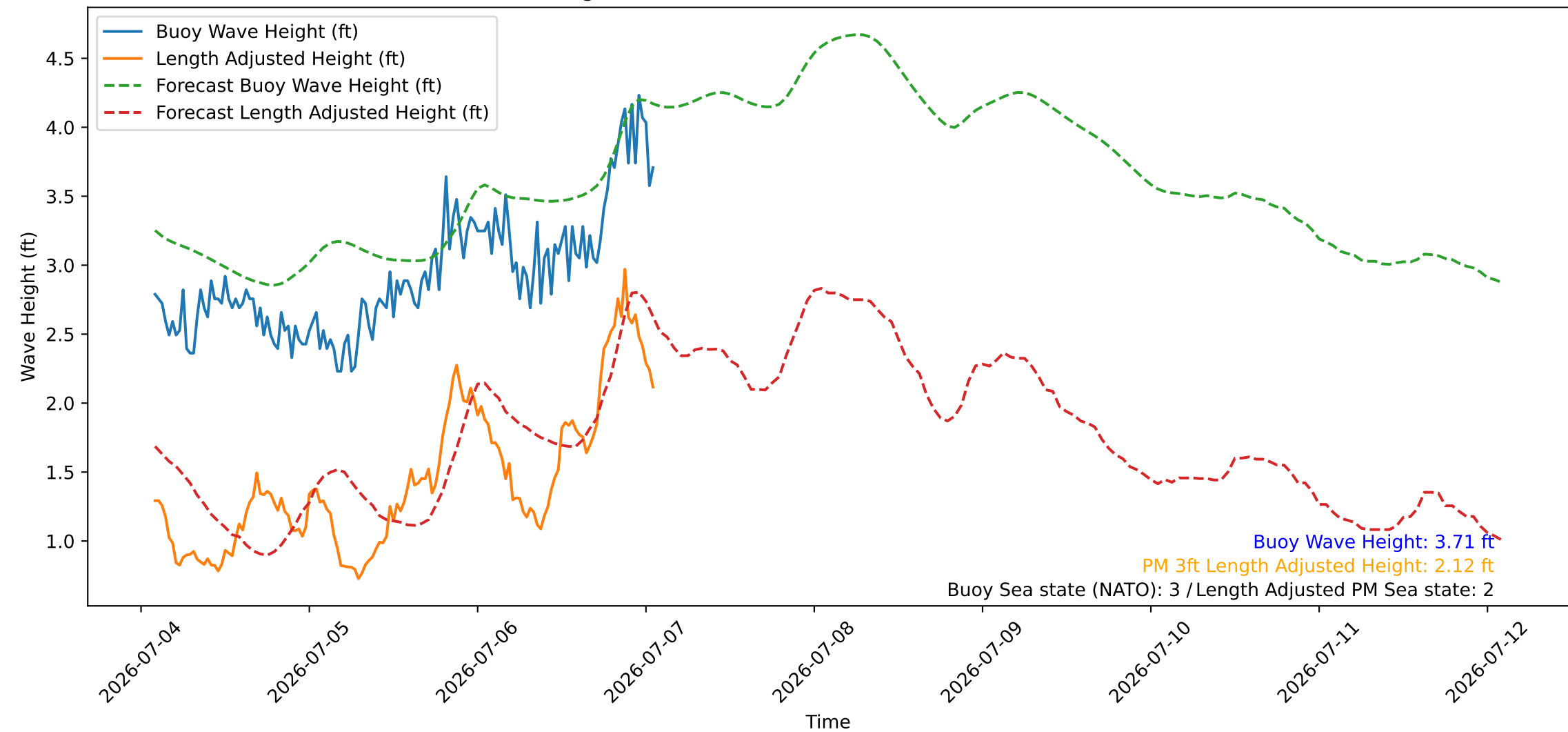
Wave Heights over Time for Red Beach at 2026-07-07 01:40:46
