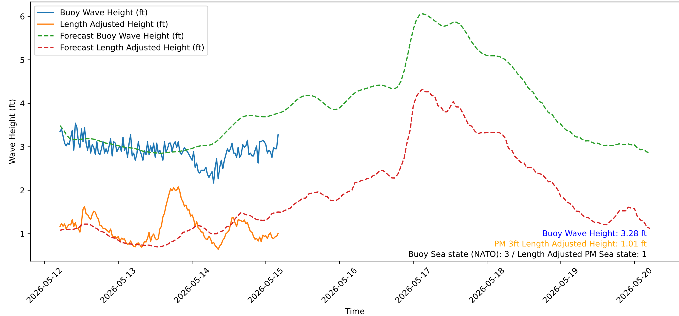
Wave Heights over Time for Oceanside Harbor at 2026-05-15 04:50:31
