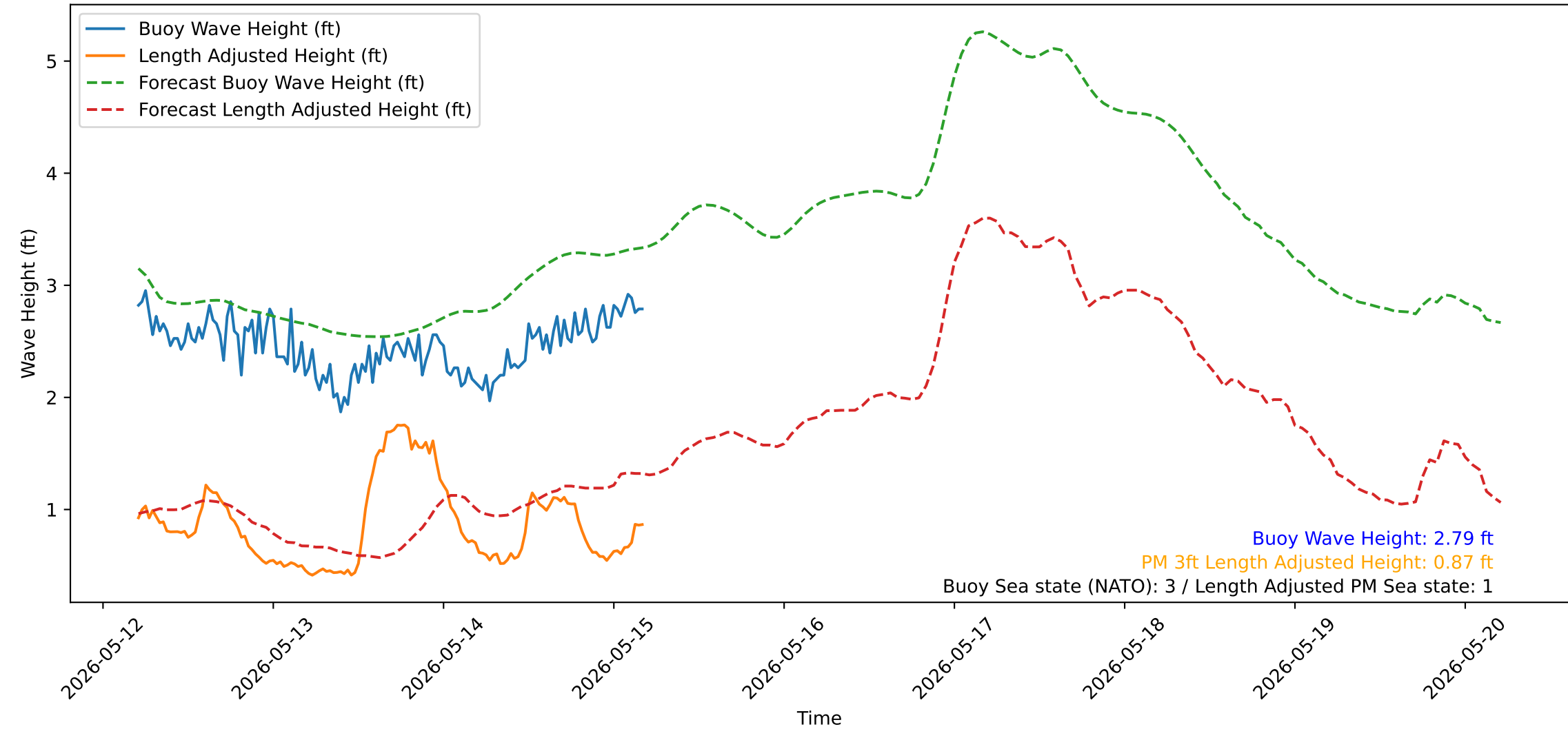
Wave Heights over Time for Red Beach at 2026-05-15 04:50:51
