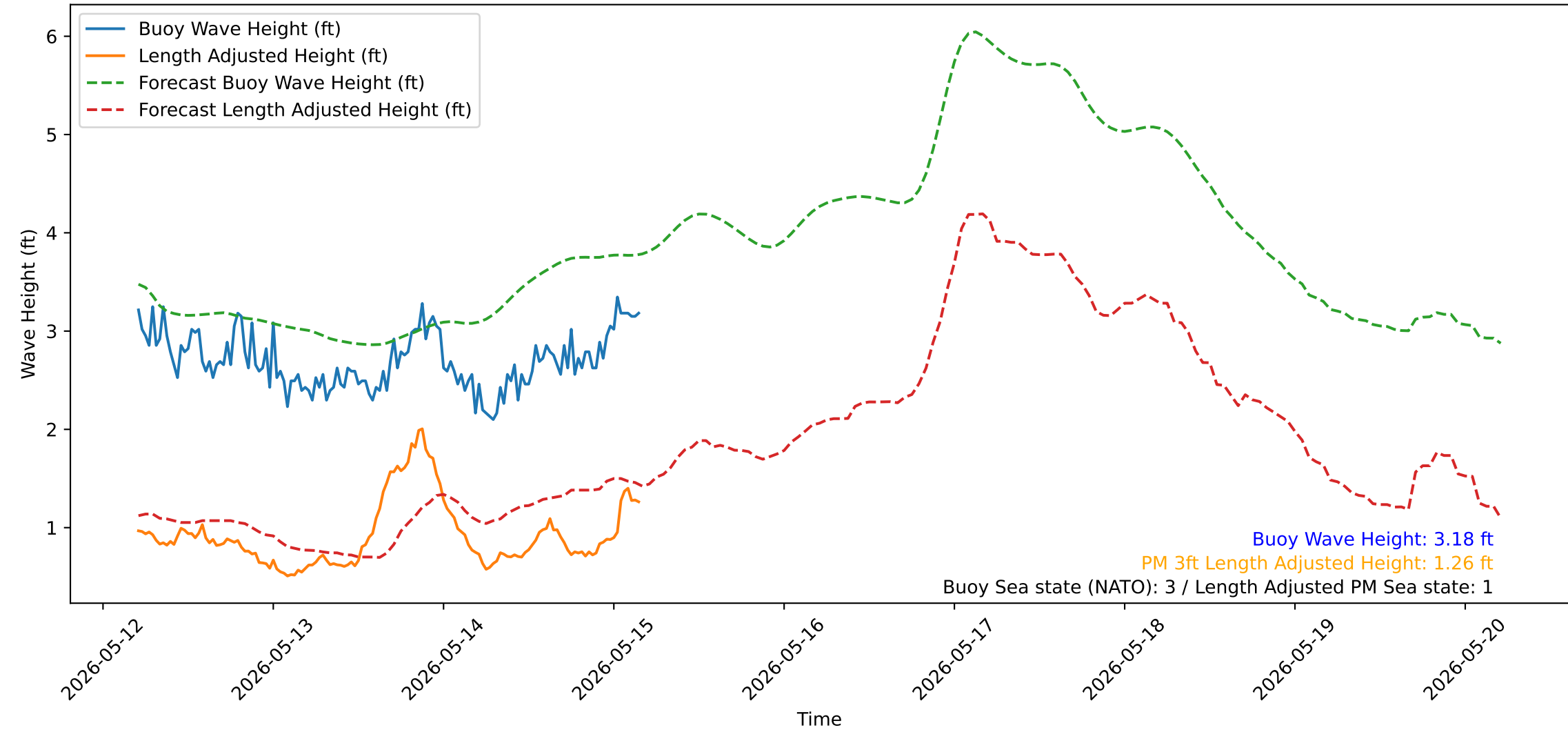
Wave Heights over Time for Green Beach at 2026-05-15 04:51:14
