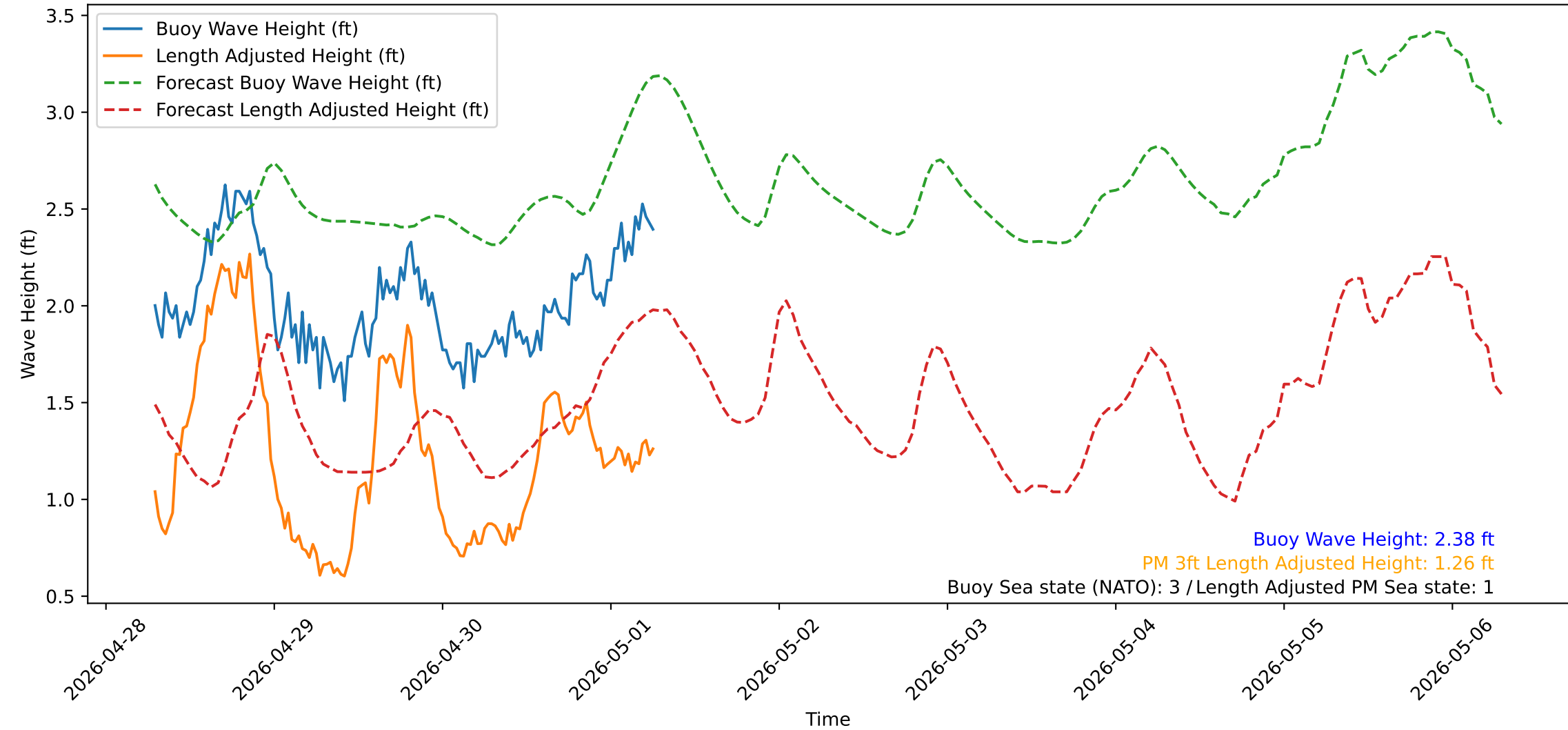
Wave Heights over Time for Red Beach at 2026-05-01 06:40:51
