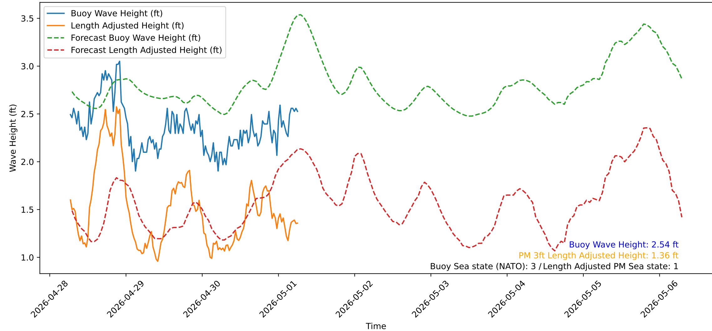
Wave Heights over Time for Oceanside Harbor at 2026-05-01 06:40:31
