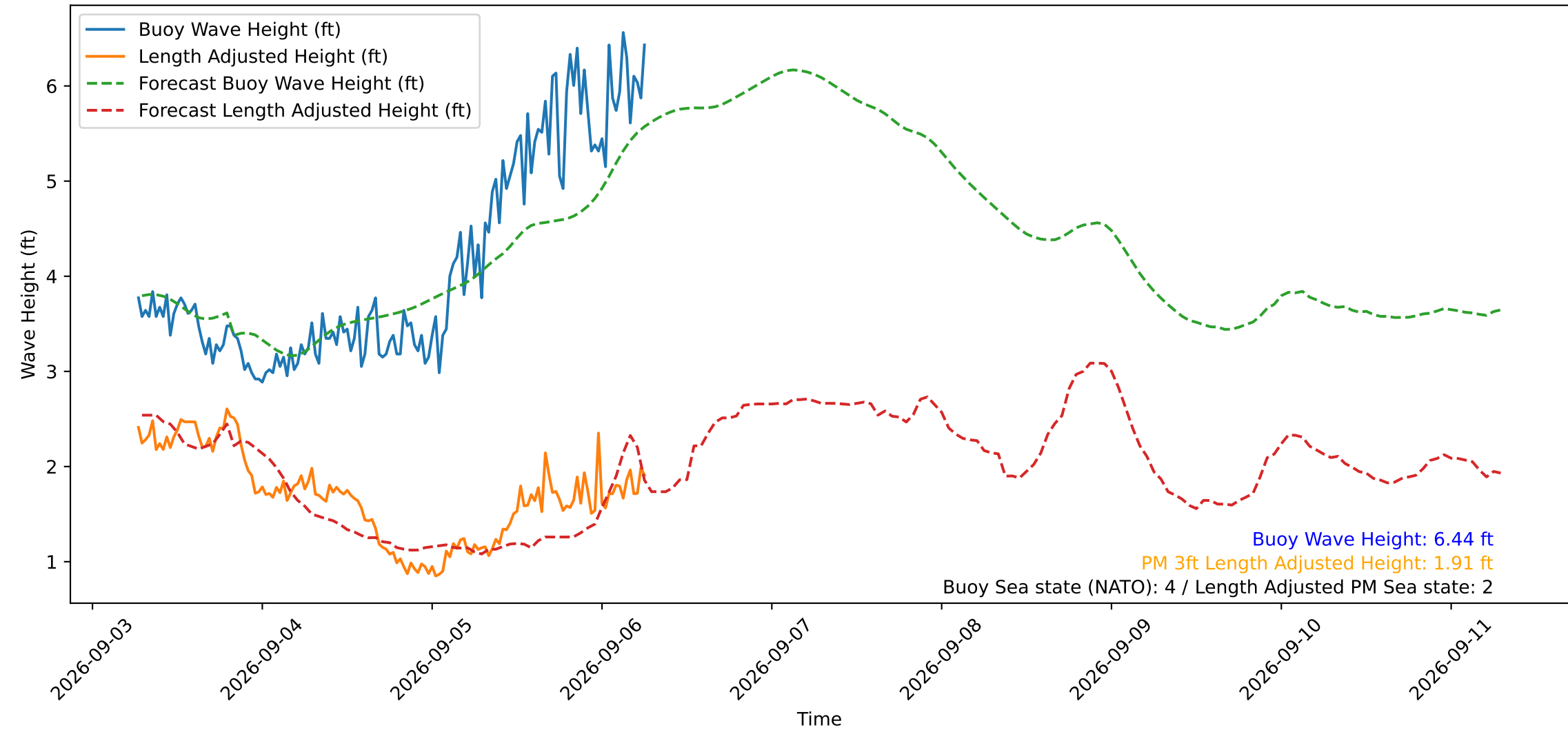
Wave Heights over Time for Oceanside Harbor at 2026-09-06 06:40:29
