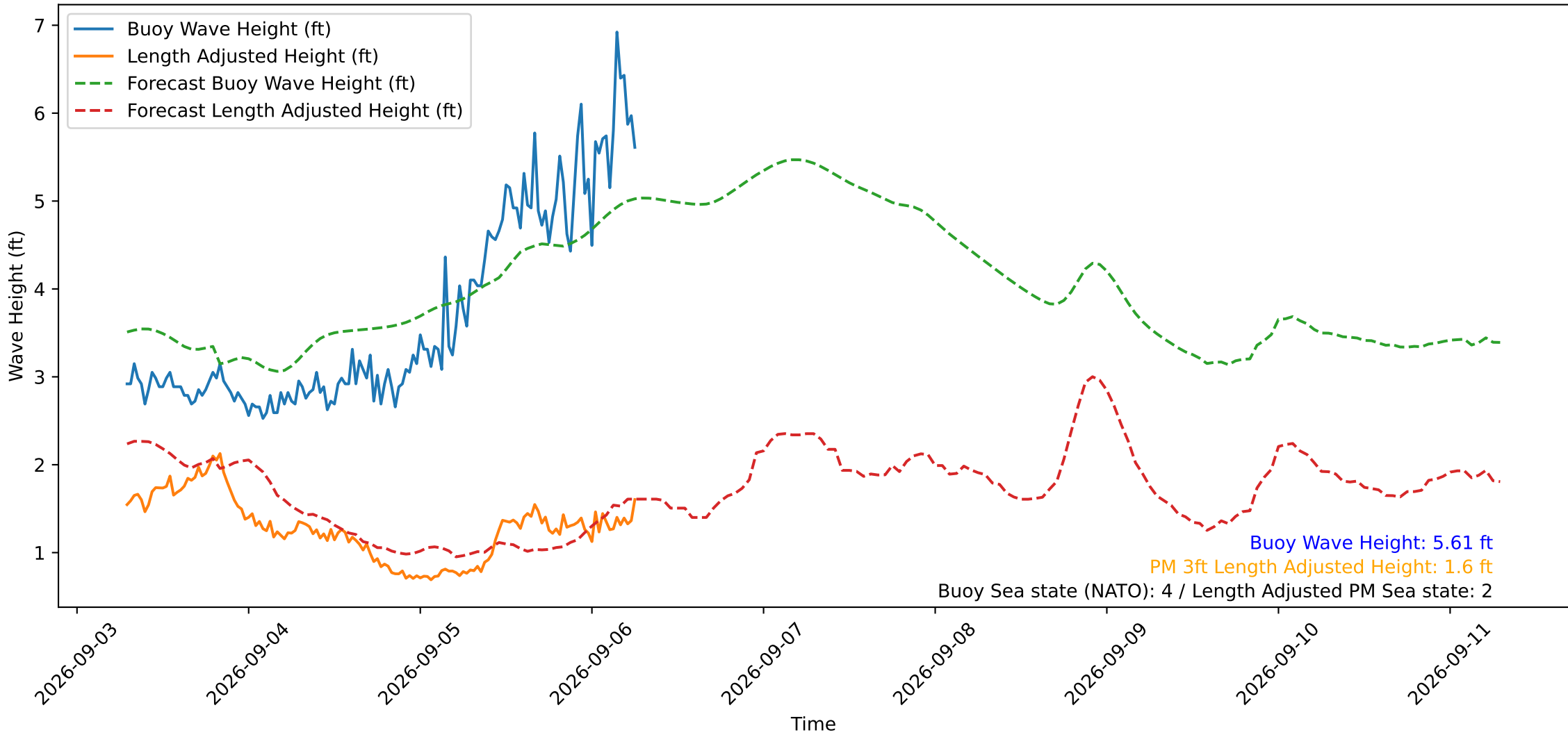
Wave Heights over Time for Red Beach at 2026-09-06 06:40:49
