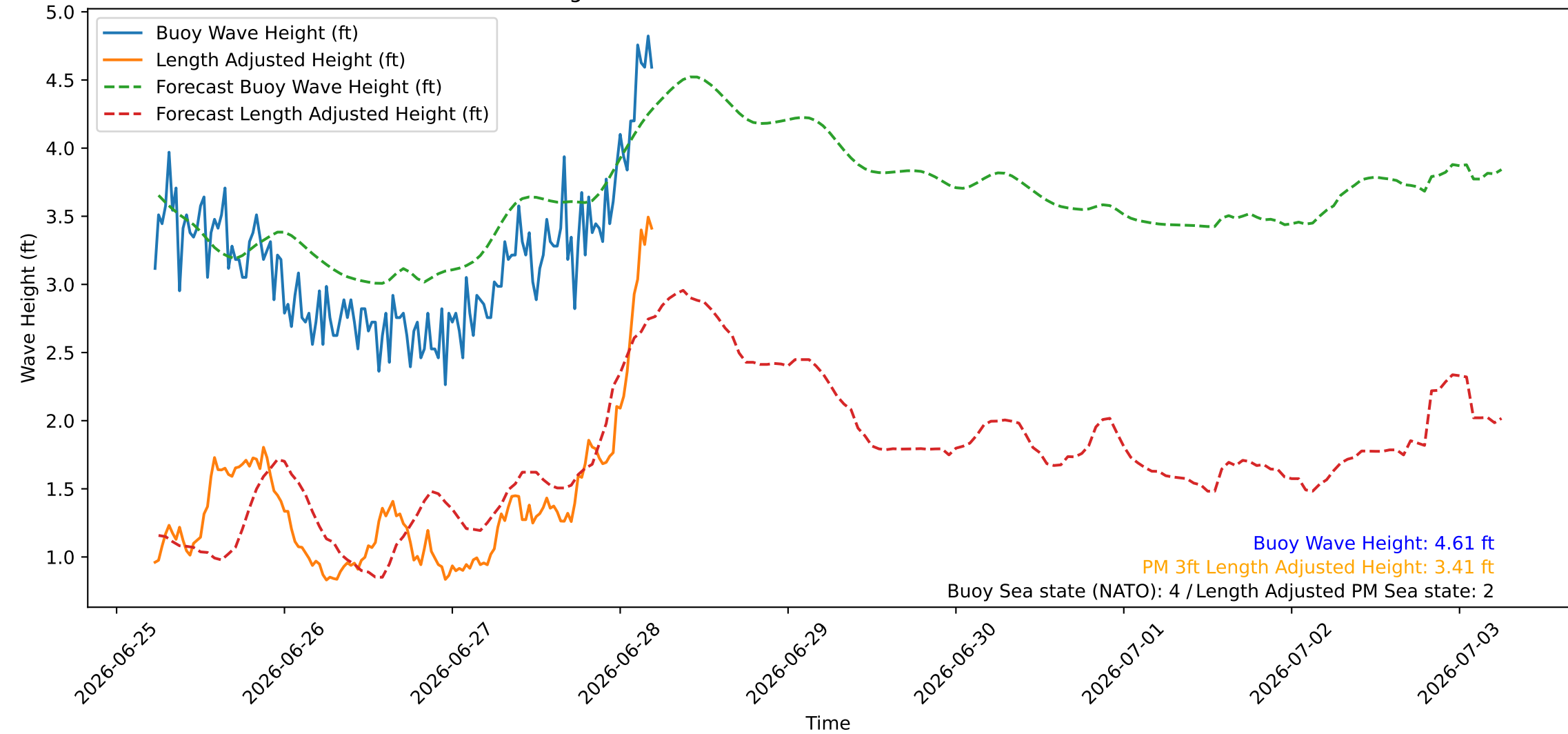
Wave Heights over Time for Green Beach at 2026-06-28 05:31:07
