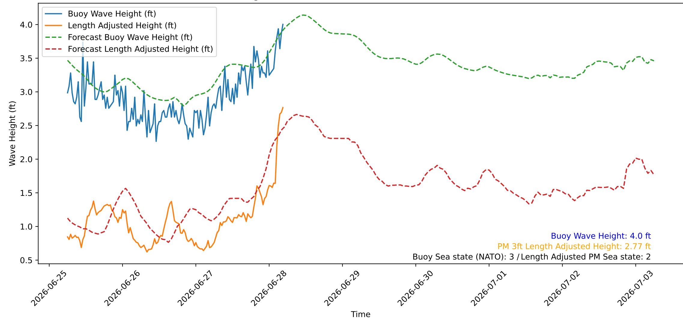
Wave Heights over Time for Red Beach at 2026-06-28 05:30:45
