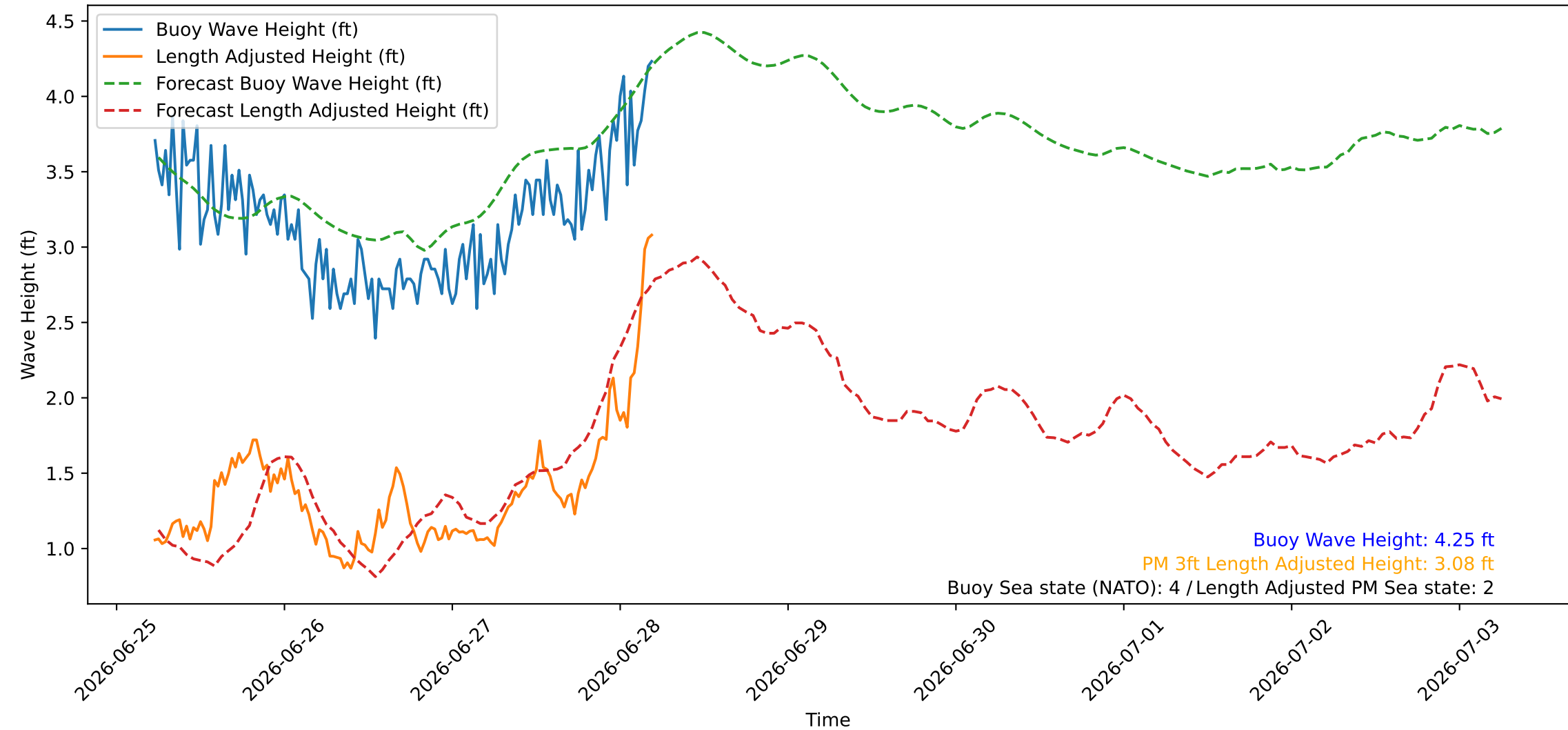
Wave Heights over Time for Oceanside Harbor at 2026-06-28 05:30:25
