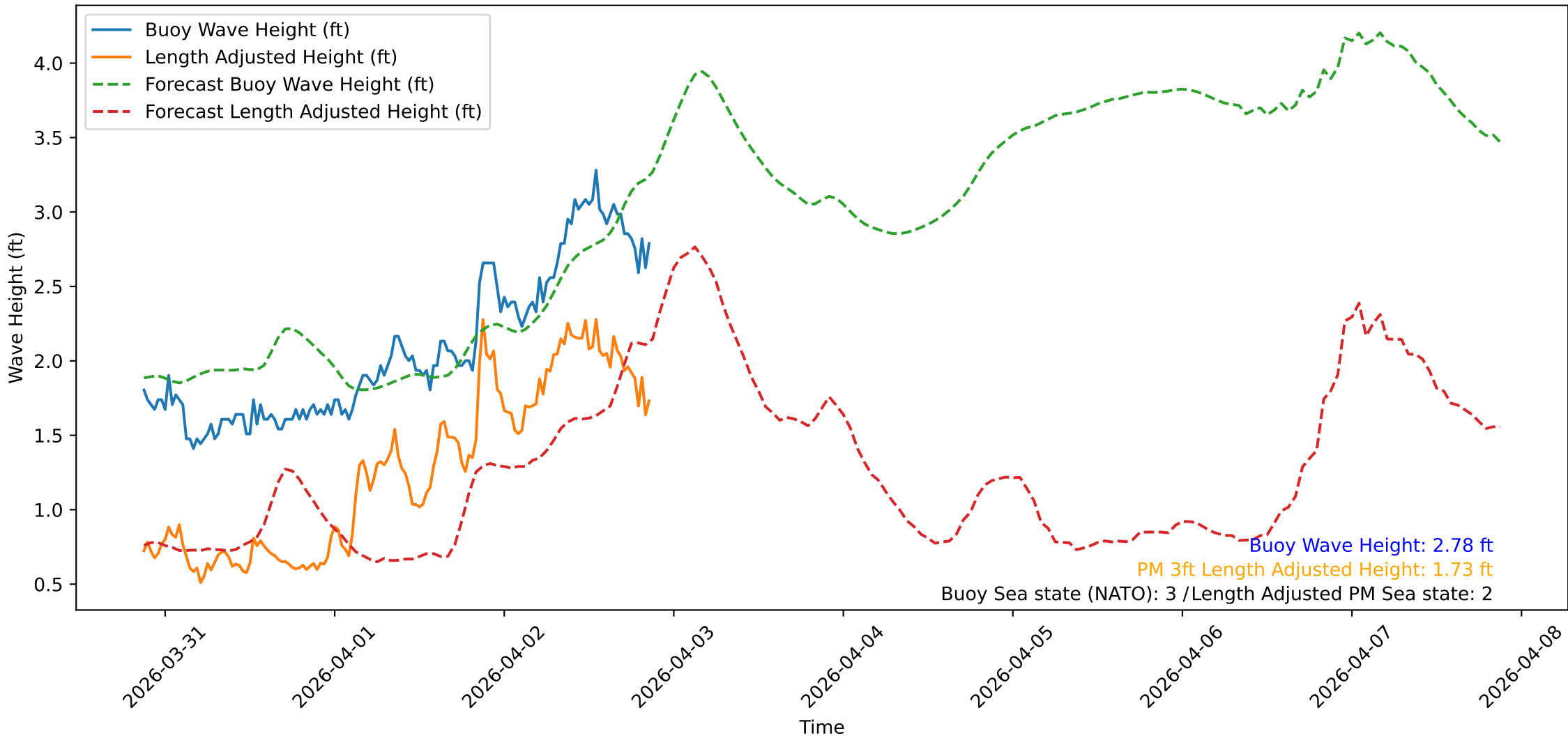
Wave Heights over Time for Green Beach at 2026-04-02 21:11:09
