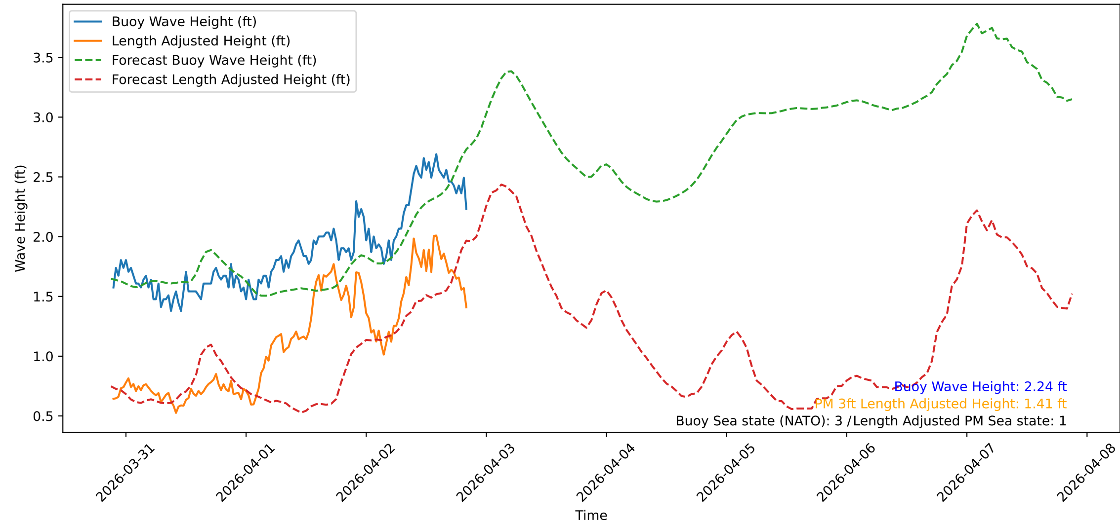
Wave Heights over Time for Red Beach at 2026-04-02 21:10:47
