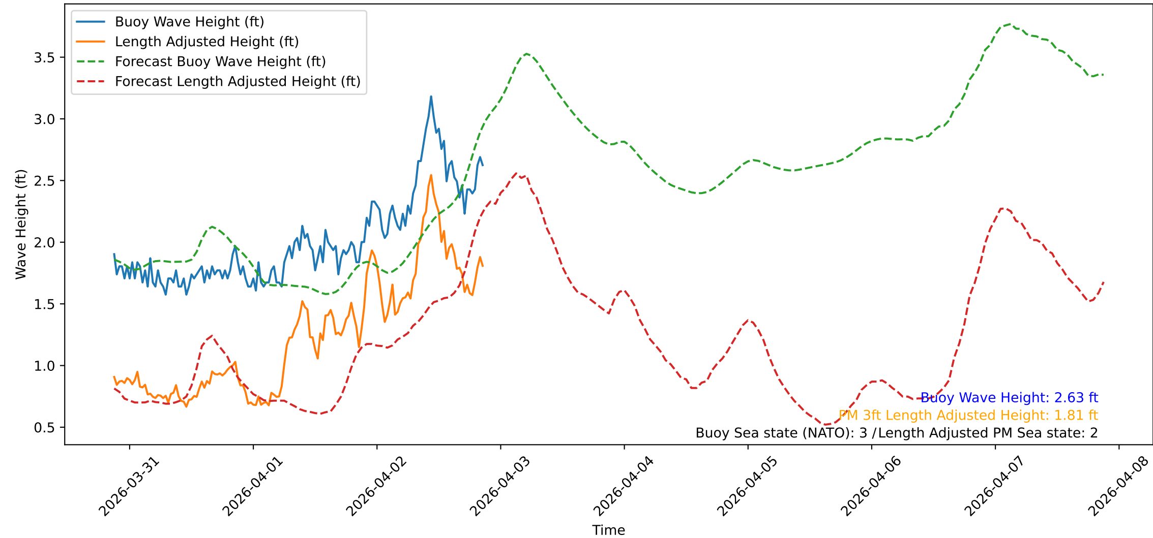
Wave Heights over Time for Oceanside Harbor at 2026-04-02 21:10:31
