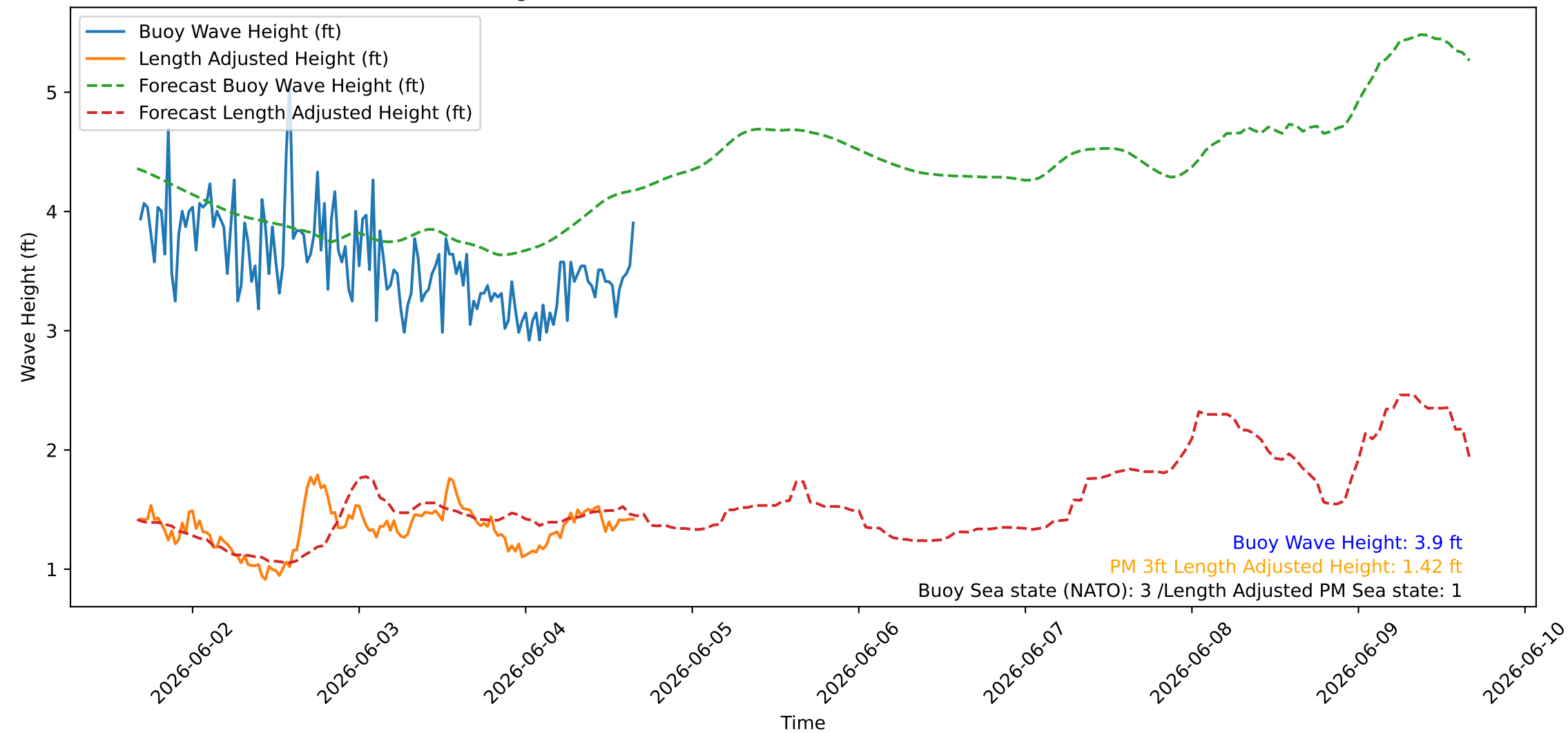
Wave Heights over Time for Oceanside Harbor at 2026-06-04 16:20:26
