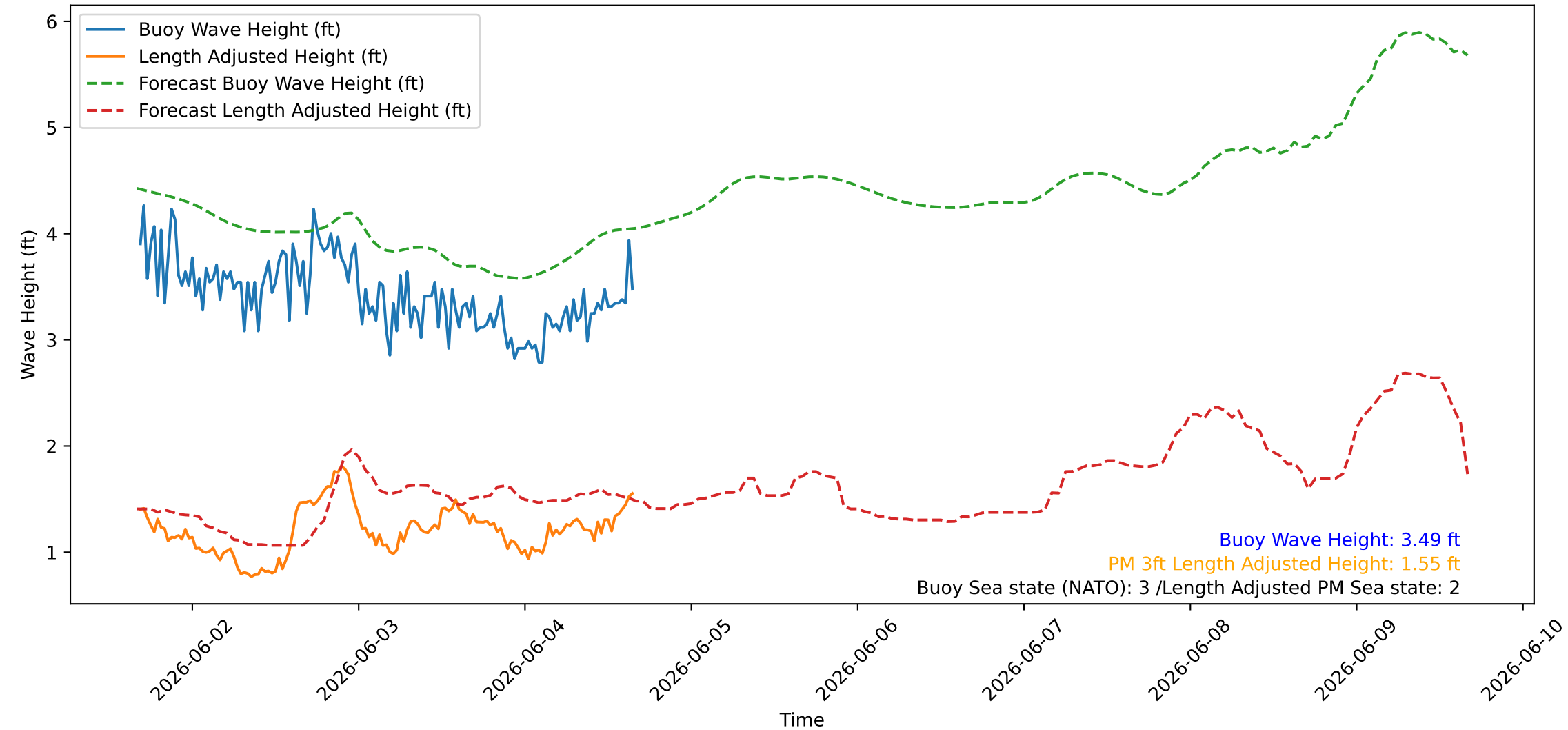
Wave Heights over Time for Green Beach at 2026-06-04 16:21:10
