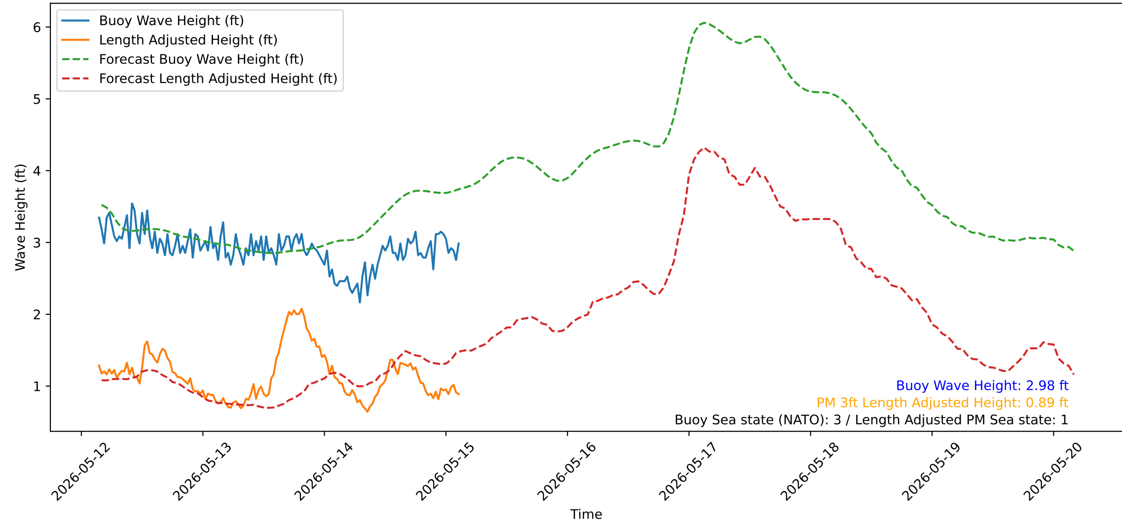
Wave Heights over Time for Oceanside Harbor at 2026-05-15 03:40:31
