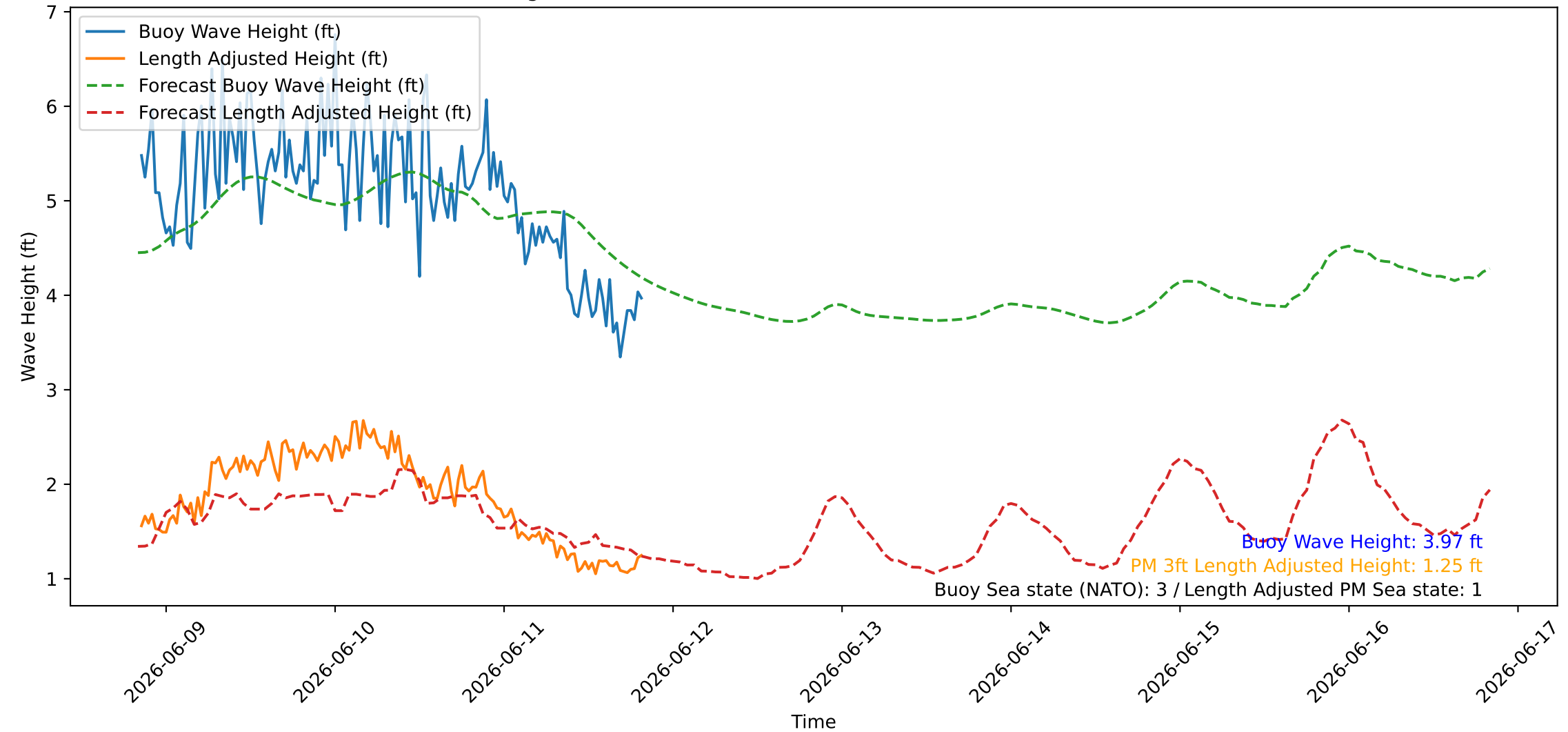
Wave Heights over Time for Oceanside Harbor at 2026-06-11 20:20:26
