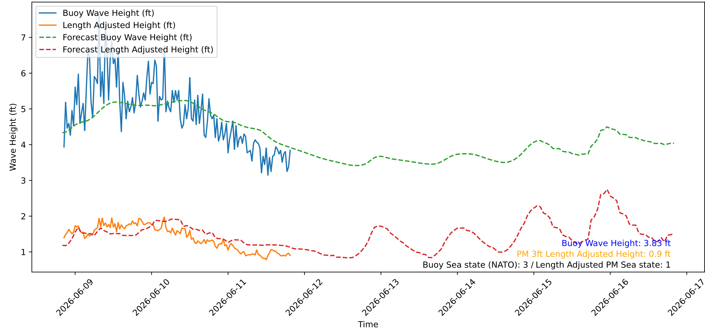
Wave Heights over Time for Red Beach at 2026-06-11 20:20:47
