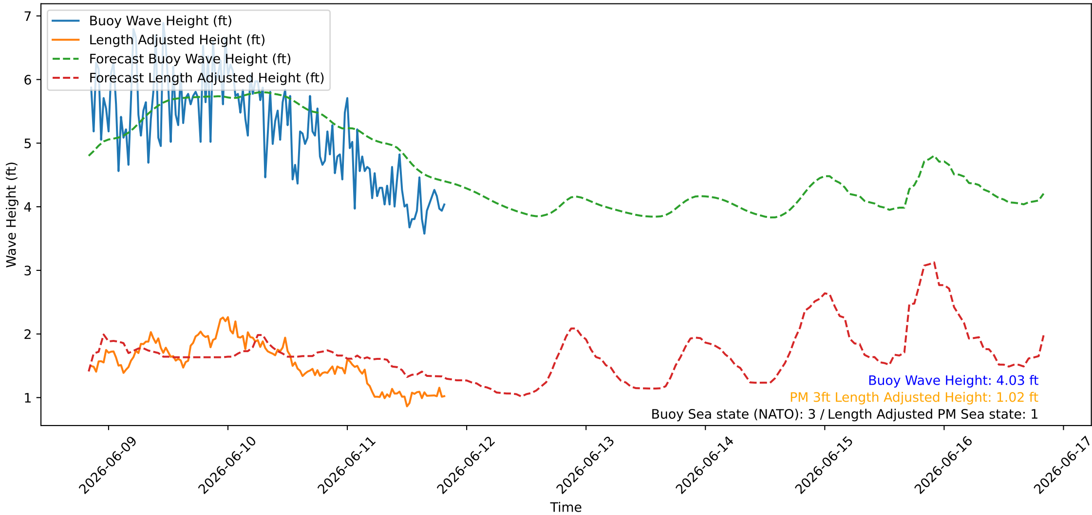
Wave Heights over Time for Green Beach at 2026-06-11 20:21:10
