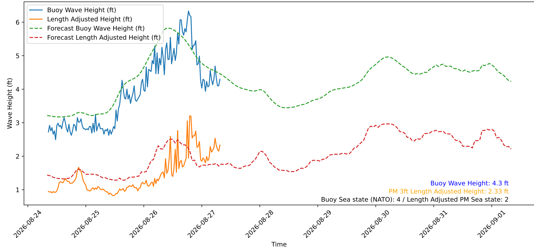
Wave Heights over Time for Green Beach at 2026-08-27 08:11:11
