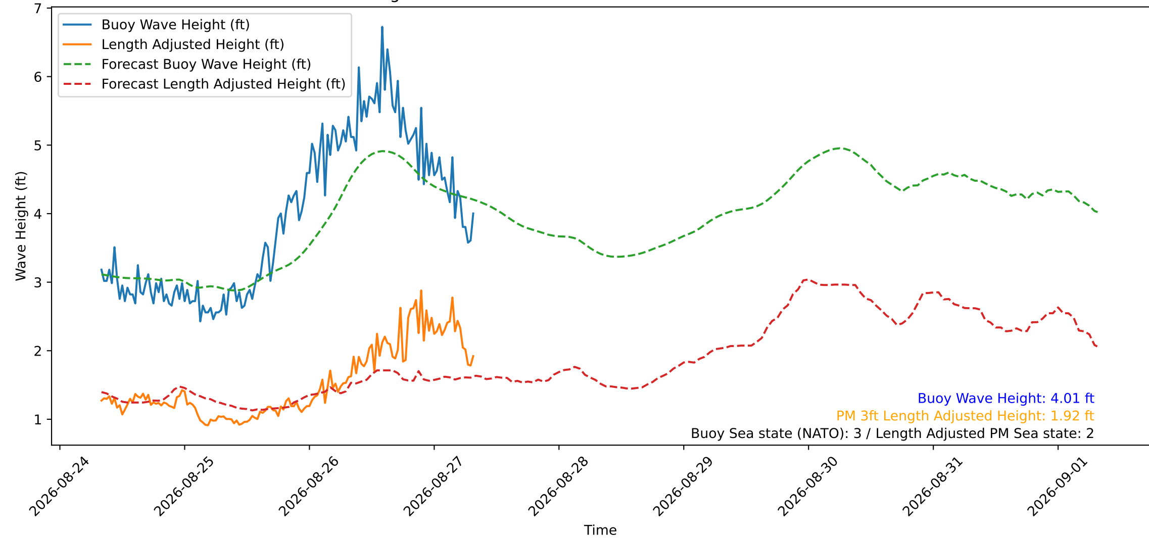
Wave Heights over Time for Oceanside Harbor at 2026-08-27 08:10:29
