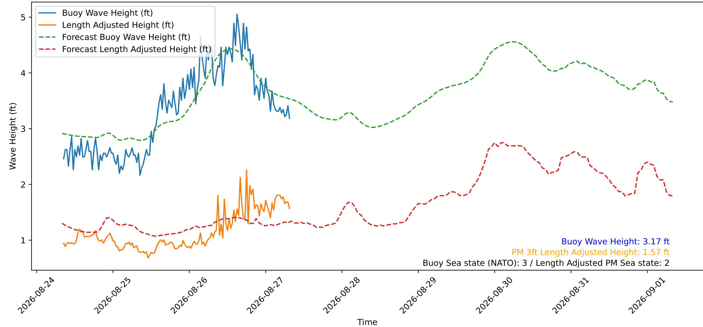
Wave Heights over Time for Red Beach at 2026-08-27 08:10:49
