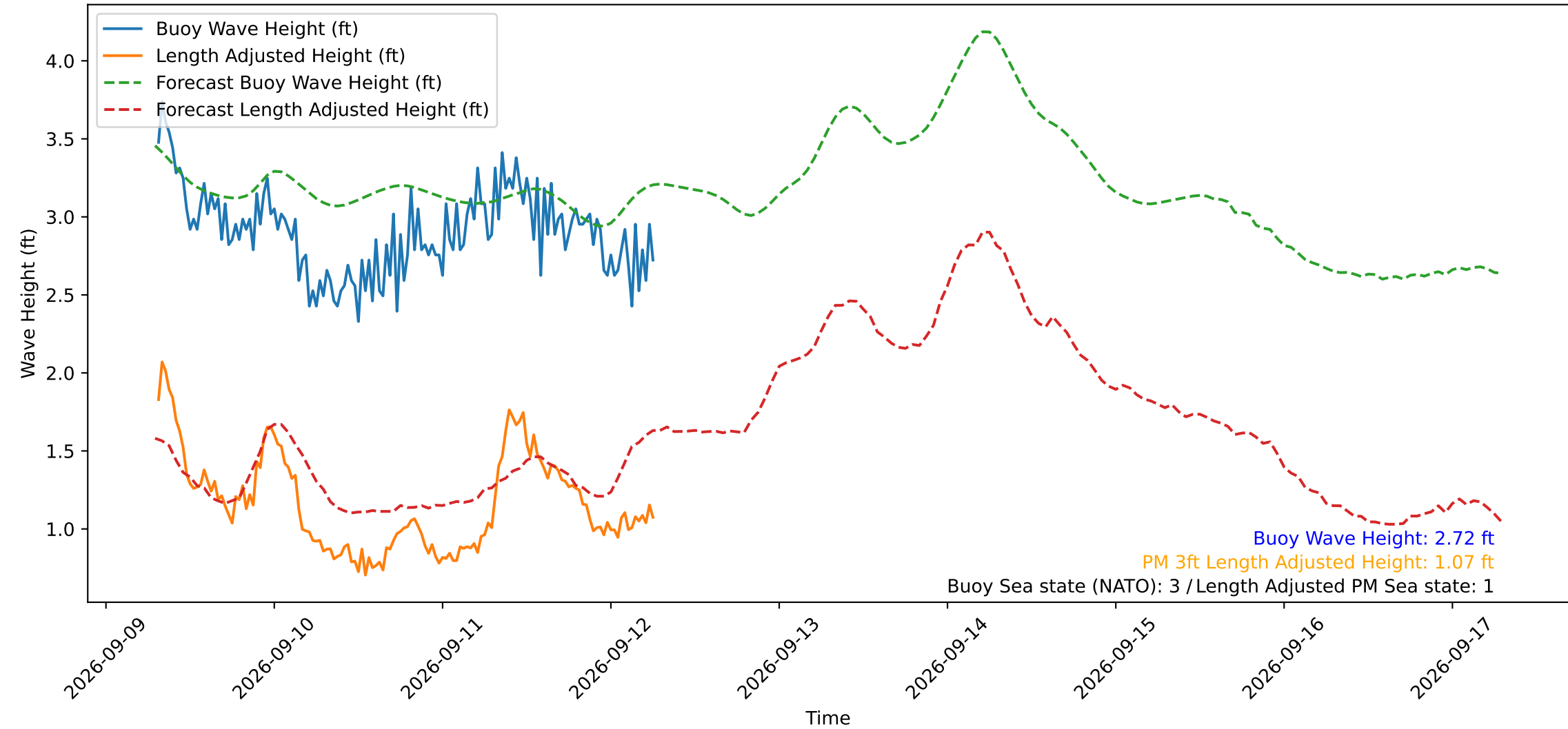
Wave Heights over Time for Red Beach at 2026-09-12 07:00:50
