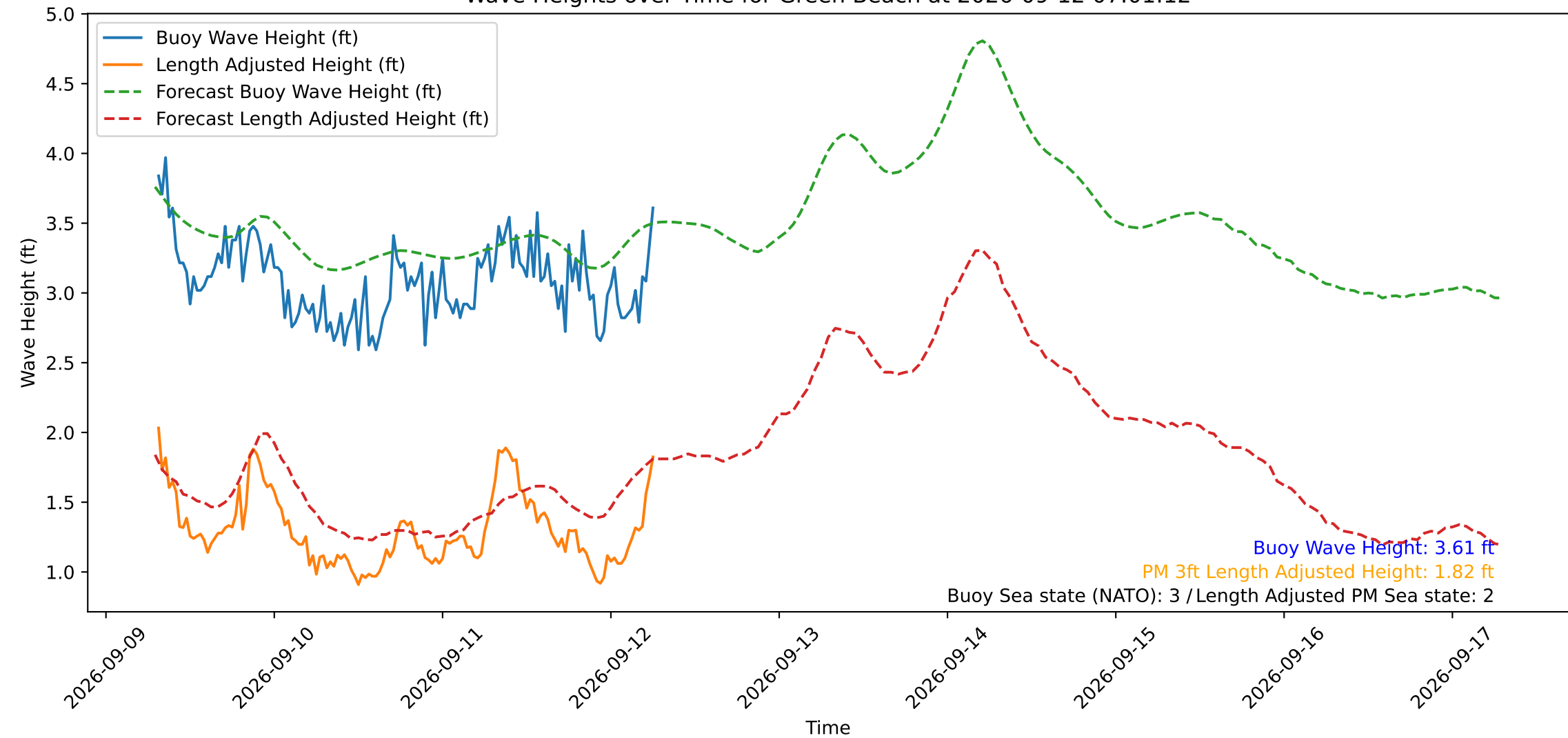
Wave Heights over Time for Green Beach at 2026-09-12 07:01:12
