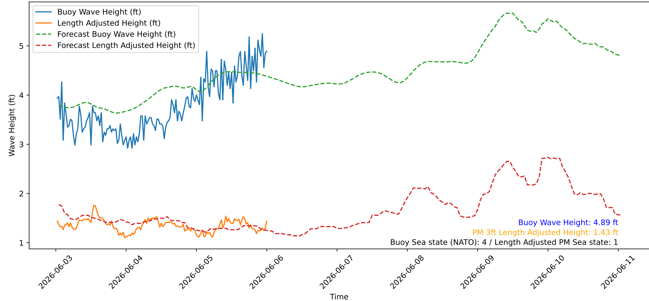
Wave Heights over Time for Oceanside Harbor at 2026-06-06 00:40:26
