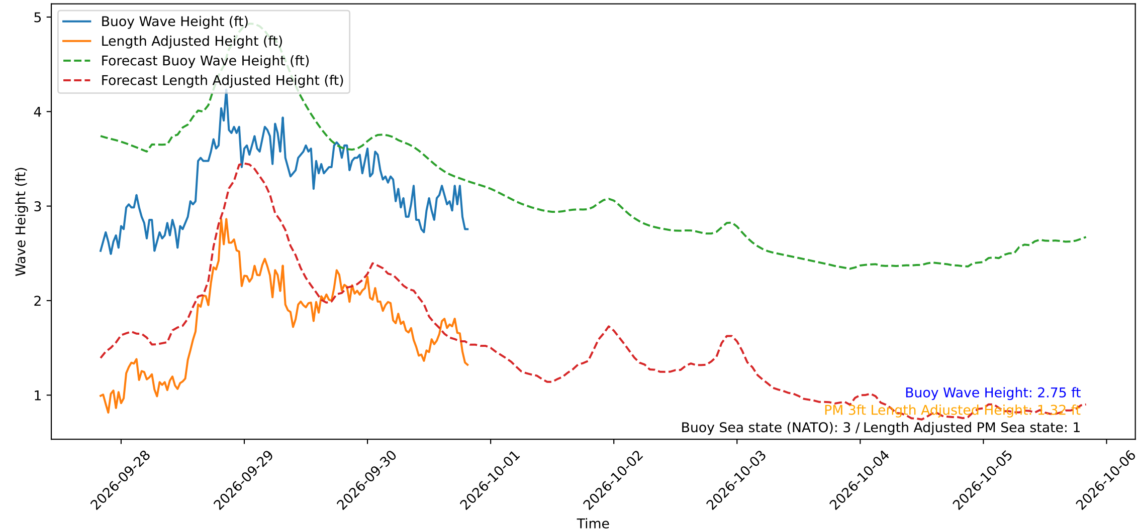
Wave Heights over Time for Oceanside Harbor at 2026-09-30 20:10:29
