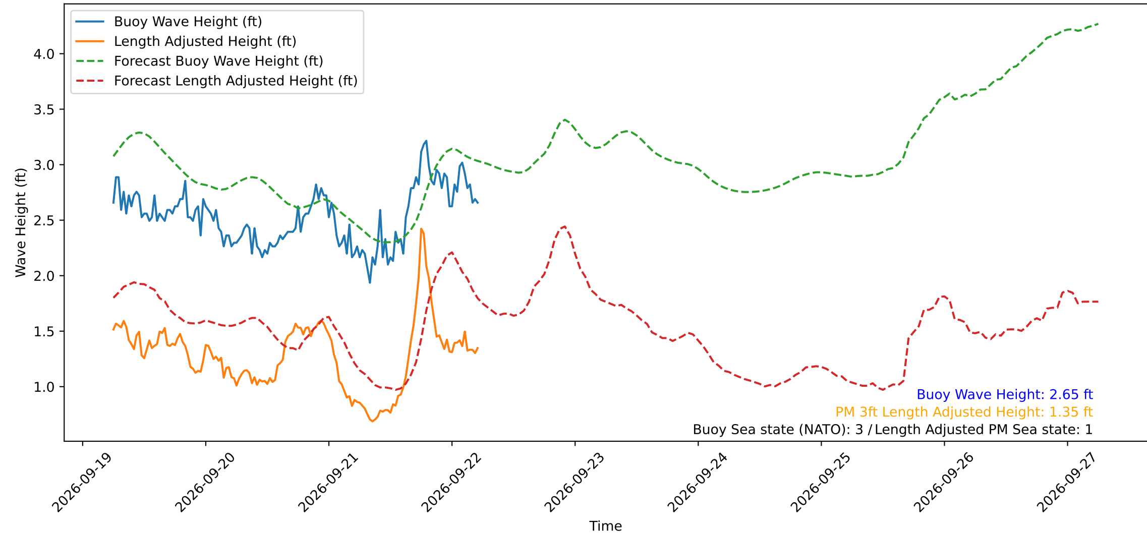
Wave Heights over Time for Green Beach at 2026-09-22 05:41:12
