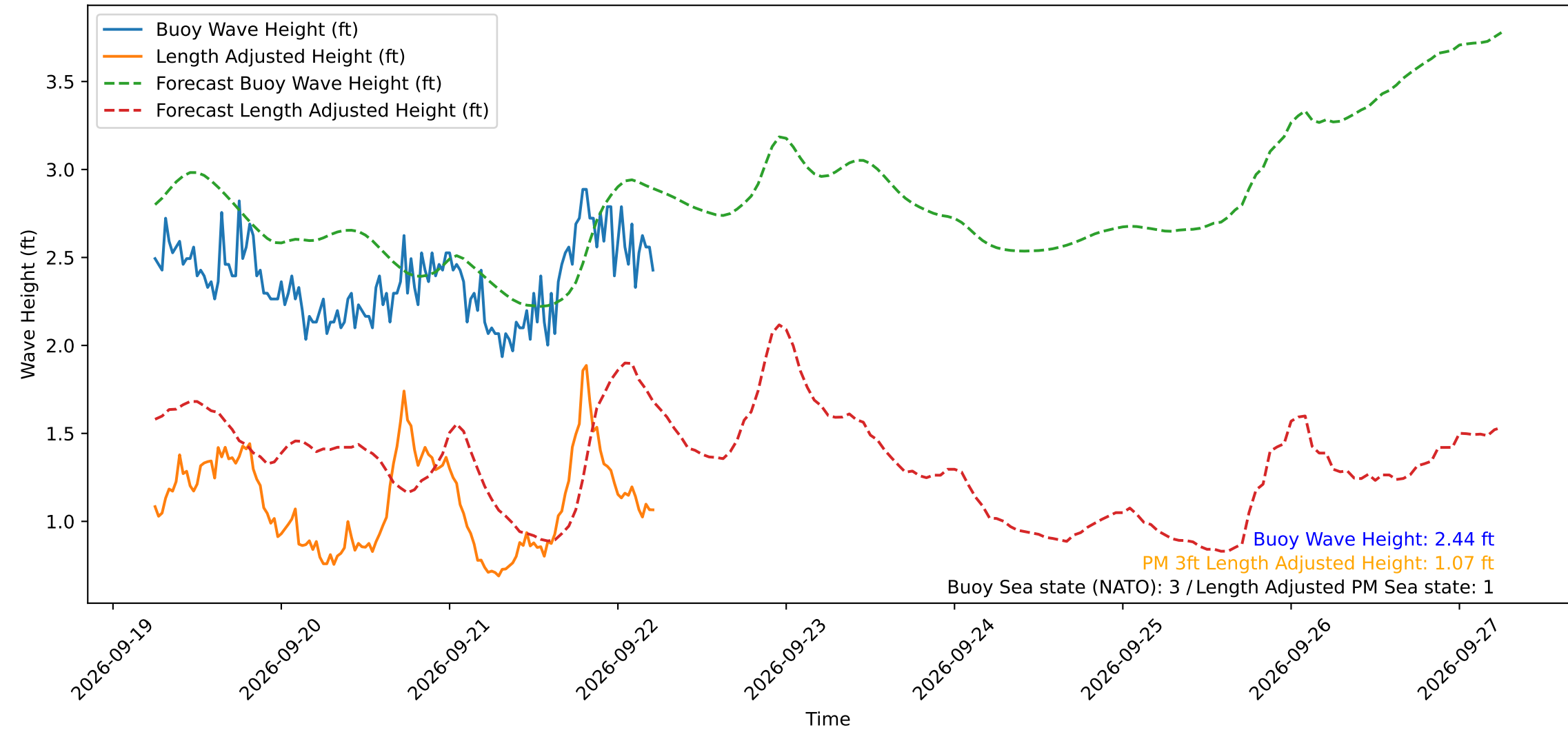
Wave Heights over Time for Red Beach at 2026-09-22 05:40:49
