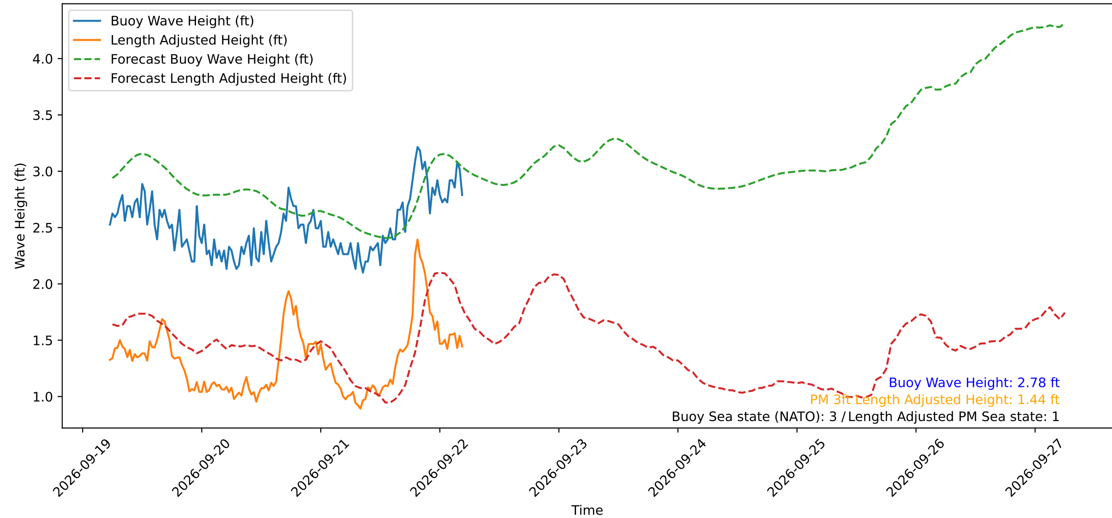
Wave Heights over Time for Oceanside Harbor at 2026-09-22 05:40:30
