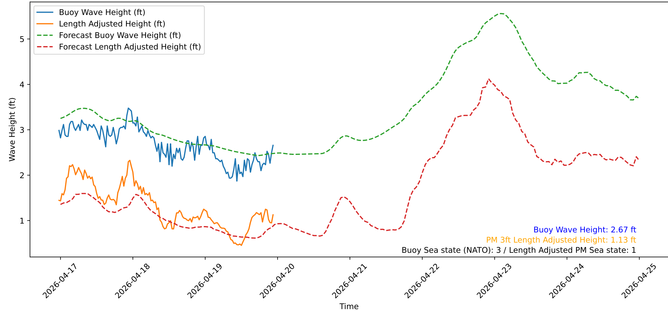
Wave Heights over Time for Green Beach at 2026-04-19 23:31:12
