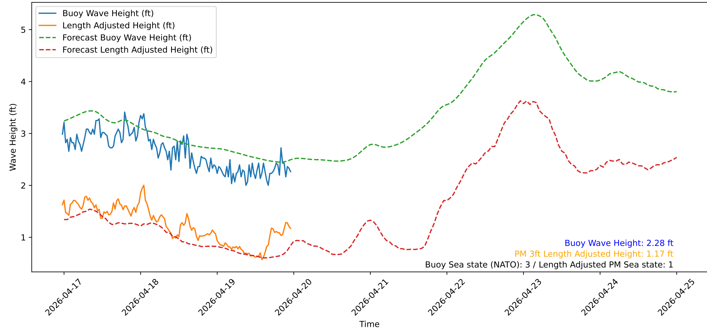
Wave Heights over Time for Oceanside Harbor at 2026-04-19 23:30:31
